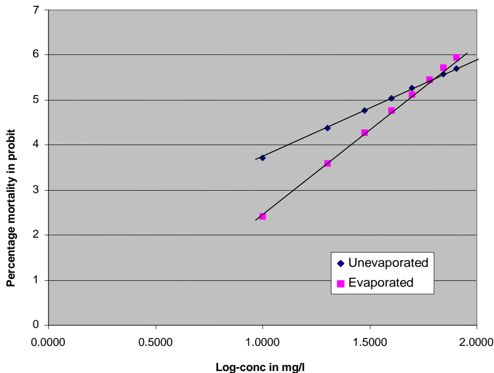
Figure 1. Log-dose, Mortality curve of evaporated and unevaporated crude water extract of Alternanthera sesselis on adult Bulinus (phy) globosus .
