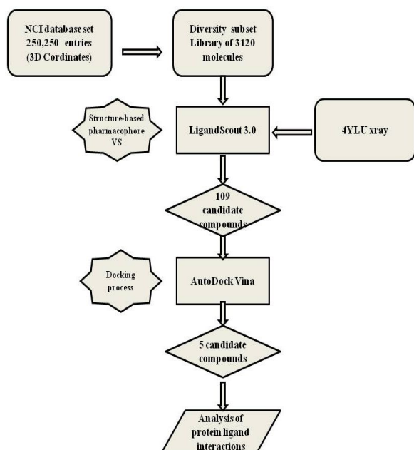
Figure 1: Schematic representation of the structure-based virtual screening work-flow
