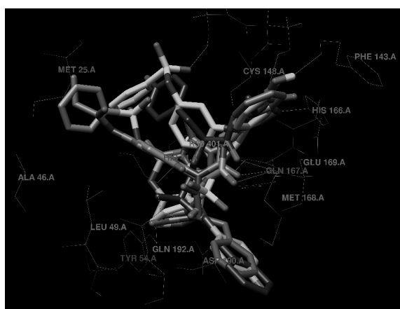
Figure 4: The 3D diagrams of interaction between the MERS-CoV 3CLpro and the five hit compounds overlaid on R30 x-ray ligand (colored black). The dotted lines show the hydrogen bond between the compounds and the binding.
