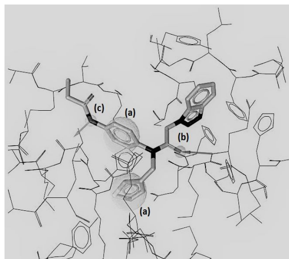
Figure 2: The macromolecule-ligand-complex-based pharmacophore model shows two hydrophobes (a), one hydrogen acceptor (b) and one hydrogen donor (c)
