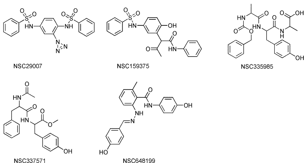
Figure 3: 2D chemical structures of the selected hit compounds
