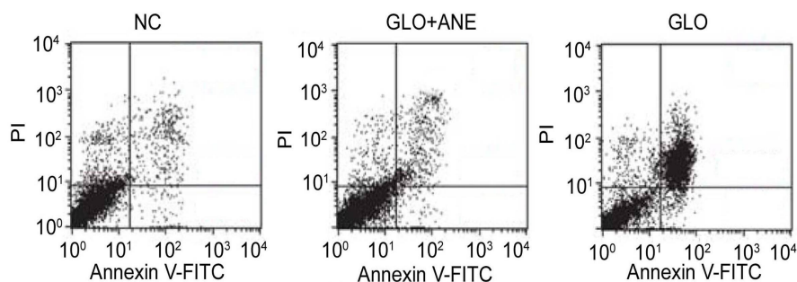
Figure 4: Artemisia annua extract prevented glyoxal-induced apoptosis in HRECs. Flow cytometry was used to determine the effect of glyoxal and Artemisia annua extract on apoptosis in HRECs after 24 h. Staining of HRECs was performed using Annexin V-FITC and PI, followed by FACS
