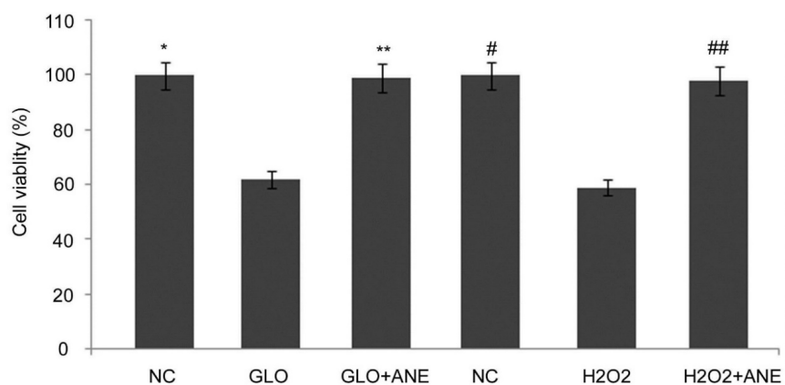
Figure 3: Artemisia annua extract prevented glyoxal-mediated loss of viability in HRECs. * p < 0.005 (glyoxal vs. control); ** p > 0.05 (glyoxal vs glyoxal + Artemisia annua extract). HRECs were exposed to H_2O_2 and then treated with Artemisia annua extract for 24 h. # p < 0.001 ( H_2O_2 vs. normal control); ## p < 0.0001 ( H_2O_2 vs H_2O_2 + Artemisia annua extract)
