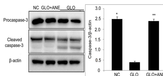
Figure 1: Artemisia annua extract inhibited glyoxal-induced cleavage of caspase-3 in HRECs. The quantification of caspase-3 level in HRECs following treatment with glyoxal and/or Artemisia annua extract was performed using Quantity One software. * p < 0.05 (glyoxal vs. normal control); ** p < 0.01 (glyoxal vs. glyoxal + Artemisia annua extract)
