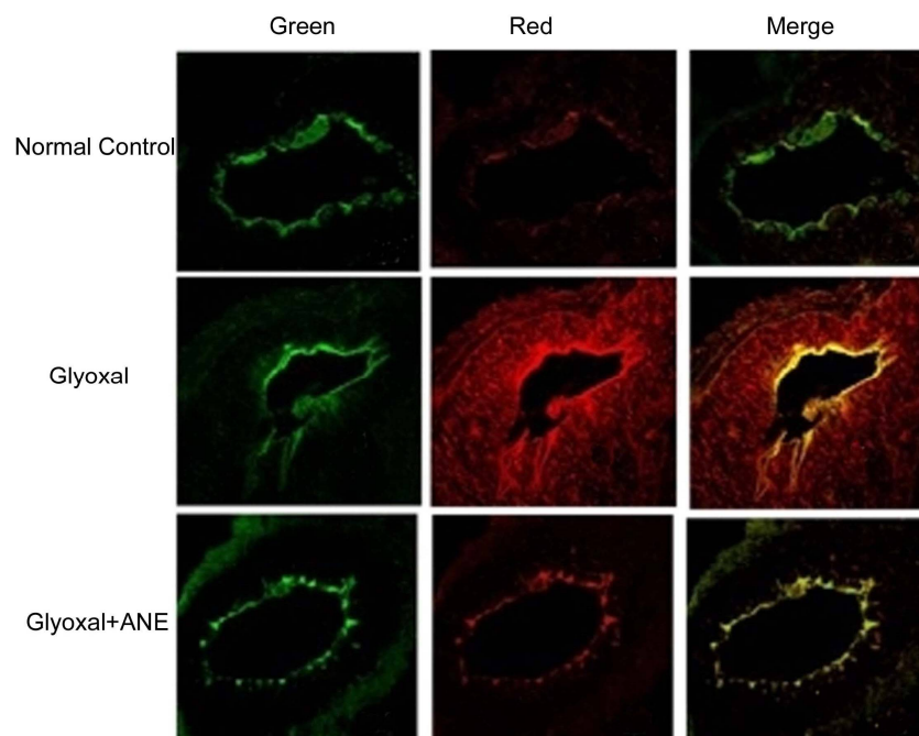
Figure 5: Effect of Artemisia annua extract on glyoxal-induced changes in mitochondrial membrane potential in HRECs. The cells were incubated with JC-1 after treatment with glyoxal and Artemisia annua extract for 24 h. Inverted fluorescent microscope and Image-Pro Plus software were used for measurement of fluorescence. The loss in membrane potential in cells treated with glyoxal was prevented by addition of Artemisia annua extract
