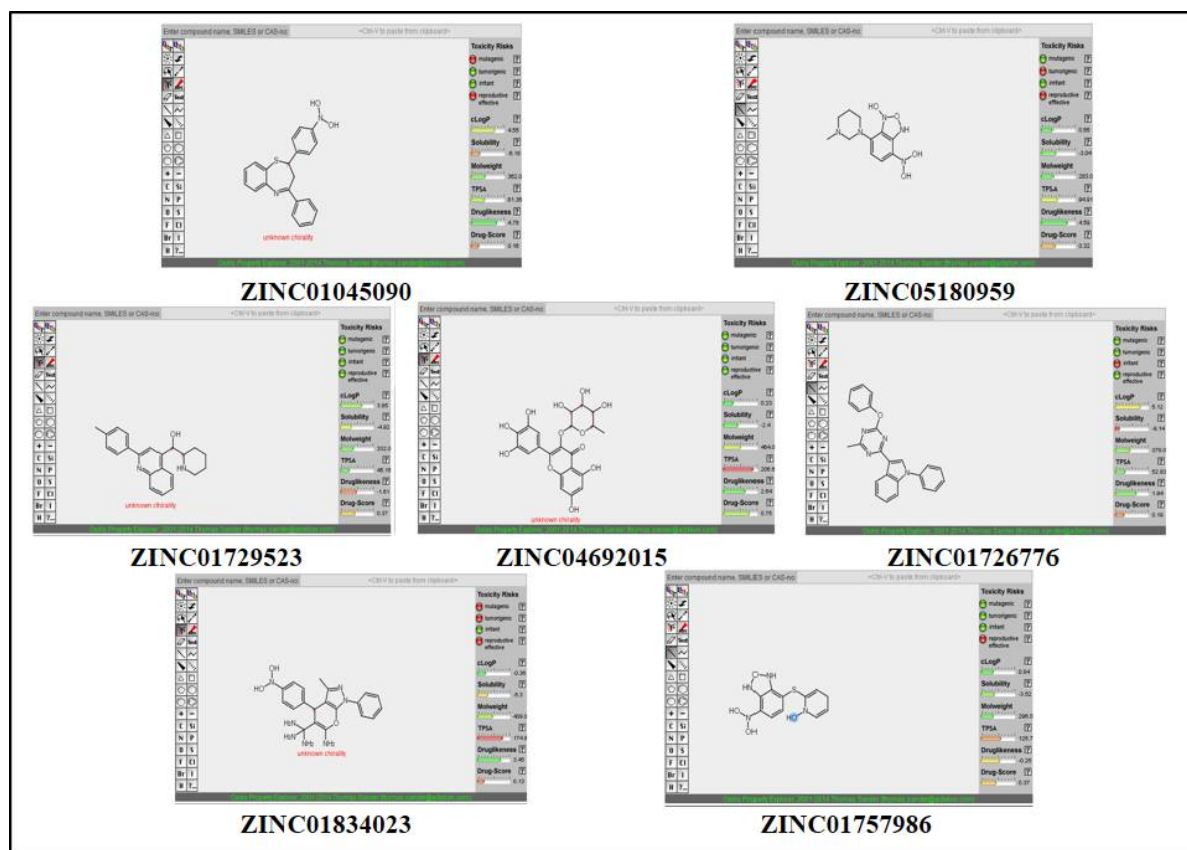
Figure 3: ADME-T profiling and toxicity prediction of the virtually-screened lead compounds [13-15]
