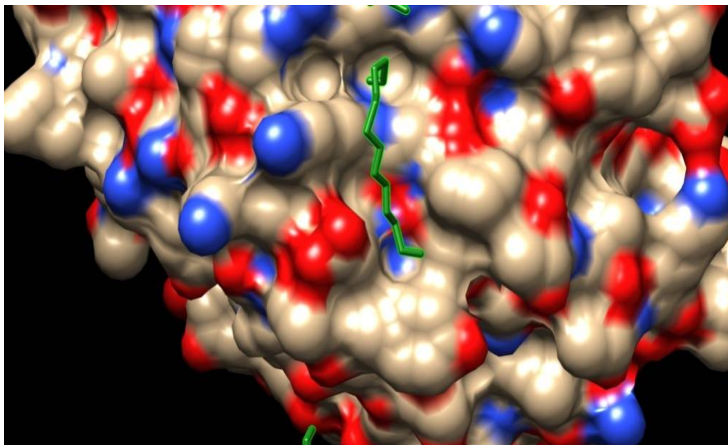
Figure 1: Binding mode and chemical interactions of the ligand hexaethylene glycol within the active binding site of human Myocilin Olfactomedin Domain protein
