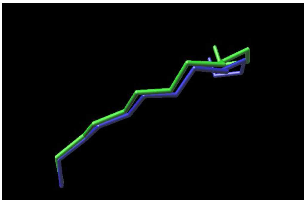
Figure 2: Overlay of chemical structures of docked conformation of the ligand with respect to its crystallized bioactive conformation [12]
