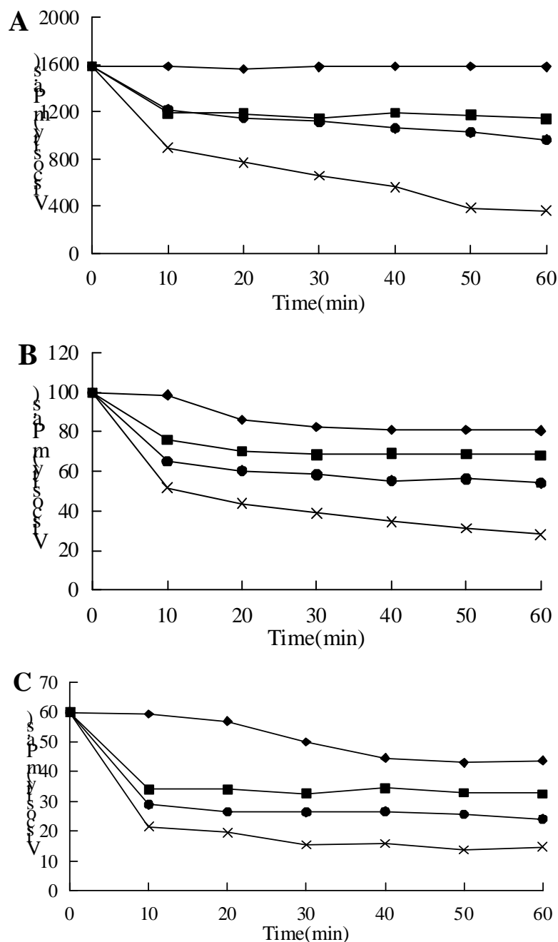
Figure 3: Effect of temperature and dilution on broth viscosity. Culture broth diluted 2-fold (A); culture broth diluted 3-fold (B); culture broth diluted 5-fold (C). Note: \blacklozenge = fermentation broth was treated at 35 °C; \blacksquare = fermentation broth was treated at 45 °C; \bullet = fermentation broth was treated at 55 °C. \times = fermentation broth was treated at 65 °C
