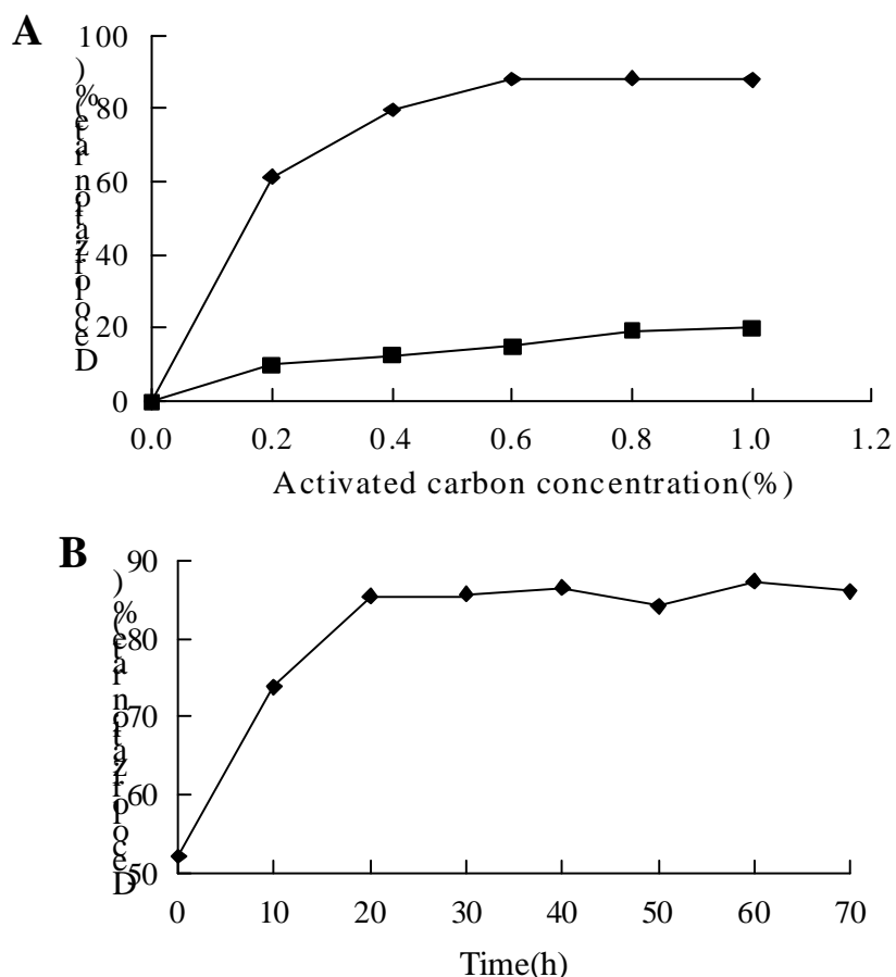
Figure 6: Effect of activated carbon powder and activated carbon granules (A), and effect of shaking time (B) on removal of pigment from fermentation liquid. Note: ◆ means powdered activated carbon. ■ means granular activated carbon
