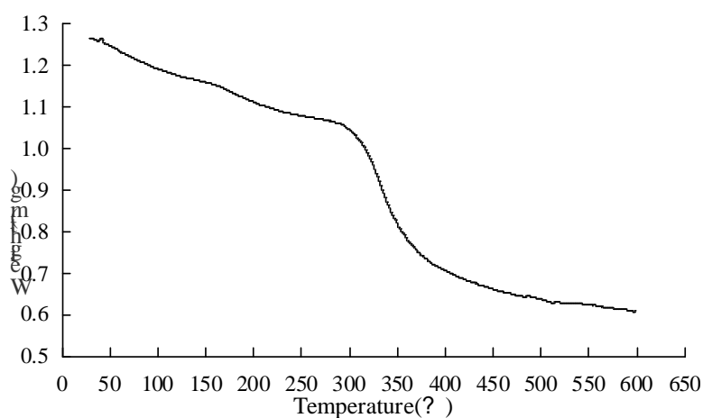
Figure 8: Thermal properties of \gamma -PGA
