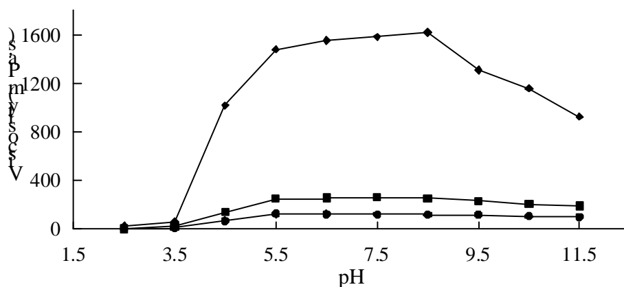
Figure 4: Effect of pH and dilution on broth viscosity. NOTE: \blacklozenge = dilution 1-fold. \blacksquare = dilution 2-fold. \bullet = dilution 3-fold
