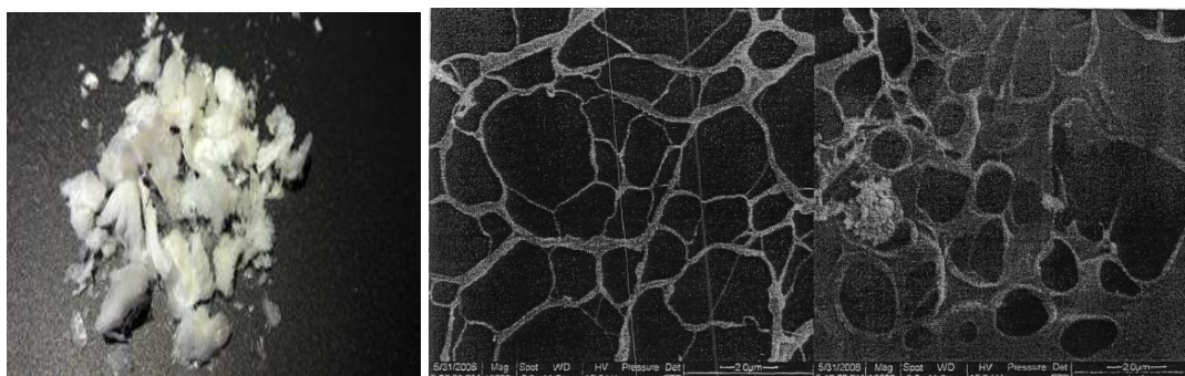
Figure 7: Concentrated solution of \gamma -PGA pre-frozen at -70^{\circ}\text{C} for 24 h, and freeze-dried at -55^{\circ}\text{C} for 48 h
