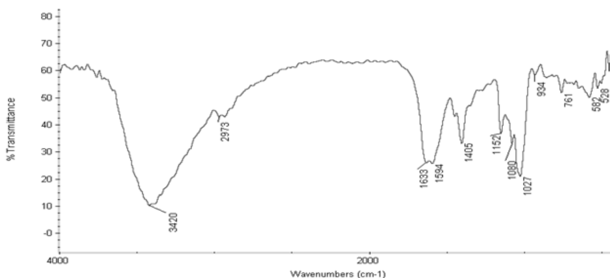
Figure 9: Infrared (FT-IR) absorption spectrum of \gamma -PGA in KBr pellet
