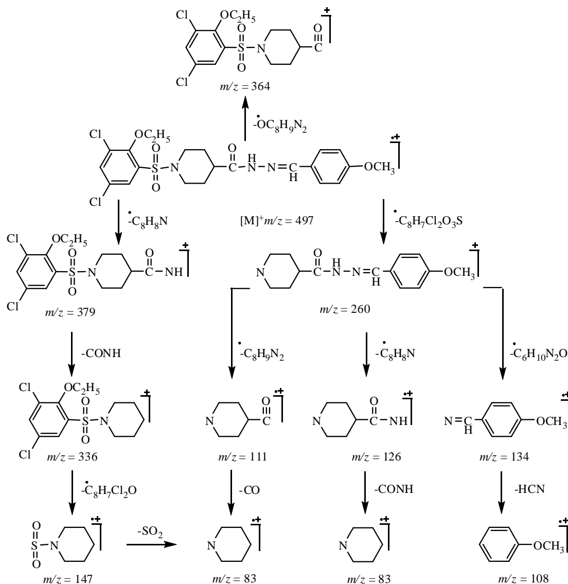
Figure 1: Mass fragmentation pattern of 1-[(3,5-dichloro-2-ethoxyphenyl)sulfonyl]- N' -(4-methoxybenzylidene)piperidin-4-carbohydrazide ( 8a )
