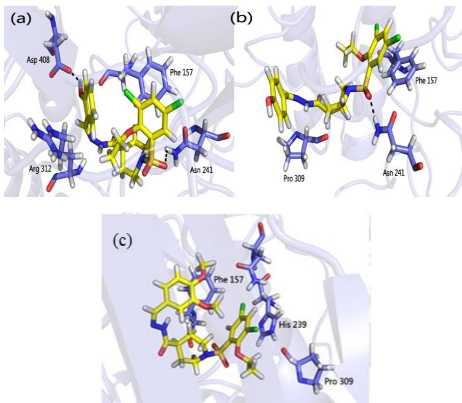
Figure 2: Binding models of compounds; (a): Compound 8e nicely binds to α-glucosidase through Asn 241 and Asp and two π-π interactions with Phe 157 and Arg 312. (b): Compound 8b binds well to α-glucosidase through Asn 241 and one π-π interaction with Phe 157. (c): Compound 8g binds to α-glucosidase and shows two π-π interactions with Phe 157 and His 239
