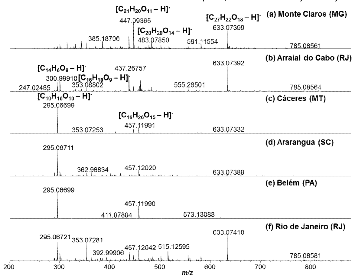
Figure 2: ESI(-)-FT-ICR mass spectra for ethanolic extracts of Euphorbia tirucalli
