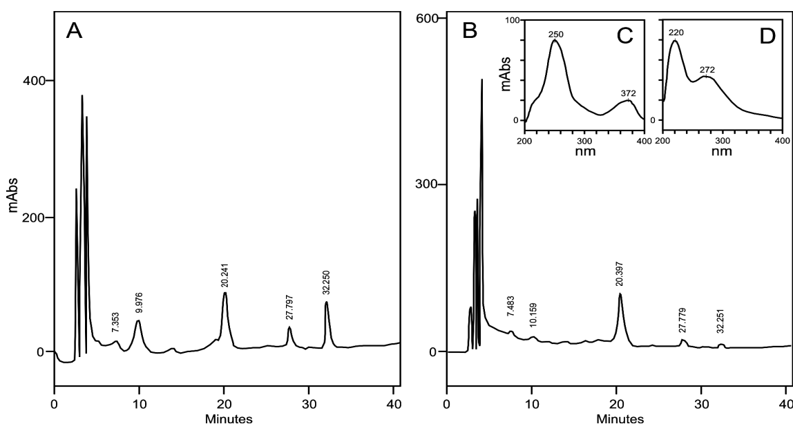
Figure 1: HPLC chromatogram profiles of Euphorbia tirucalli extracts at a wavelength of 240 nm (A. Montes Claros, MG; B. Arraial do Cabo, RJ). C and D. Ultraviolet spectra of tannins found in the extracts
