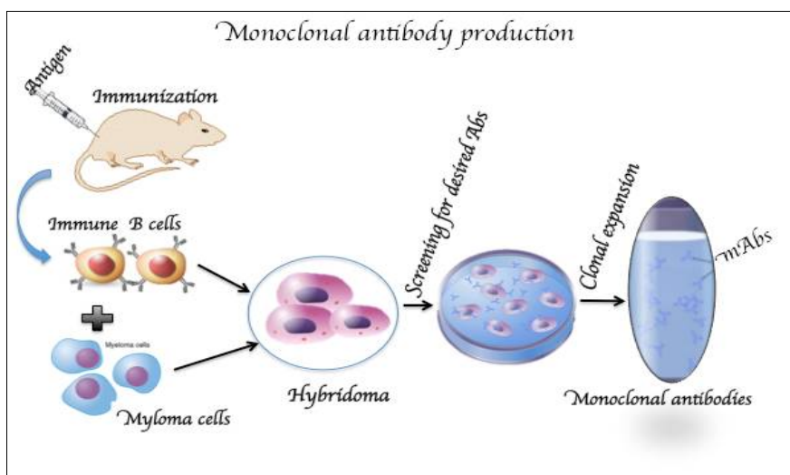
Figure 1: Steps involved in the production of mAbs
