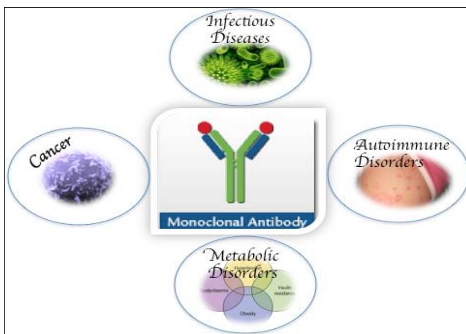
Figure 3: Some areas for therapeutic applications of mAbs
