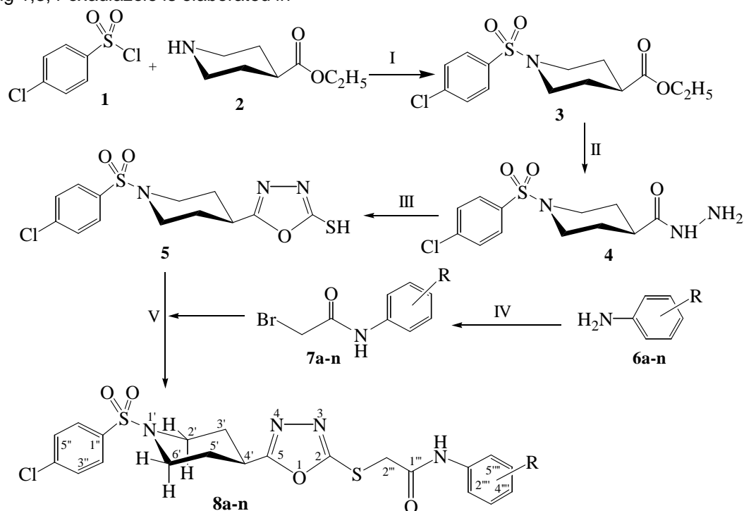
Figure 1: Protocol for synthesis of N -substituted acetamide derivatives of azinane bearing 1,3,4-oxadiazole. Reagents & conditions: (I) 15 % \text{Na}_2\text{CO}_3 solution, \text{H}_2\text{O} , stir for 3 hours. (II) \text{N}_2\text{H}_4 \cdot \text{H}_2\text{O} , \text{EtOH} , reflux for 2.5 hours. (III) \text{CS}_2 , \text{KOH} (s), \text{EtOH} , reflux for 5 hours. (IV) \text{BrCH}_2\text{COBr} , 15 % \text{Na}_2\text{CO}_3 solution, \text{H}_2\text{O} , stir for 1 hour. (V) Dimethyl formamide, \text{LiH} , stir for 3 - 4 hours.
