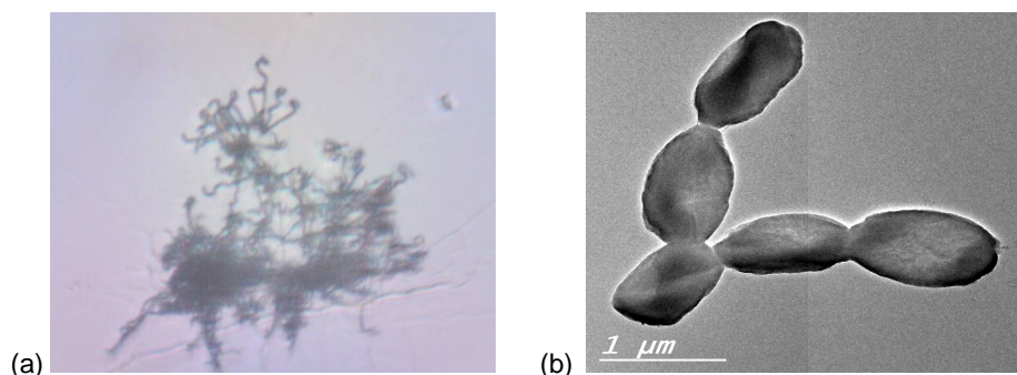
Figure 3: The morphology of Streptomyces sp. MU NRC-77 showed (a) spore chains of the spiral type by Light microscope at 200 X and (b) smooth spore surface observed under TEM at 40,000 X, The bar represents.
