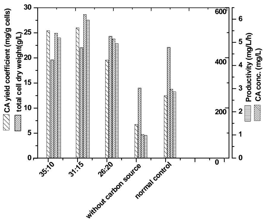
Figure 8: The effect of different combination of soluble starch and glycerol concentration on cell growth and clavulanic acid production by Streptomyces sp. MU-NRC-77
