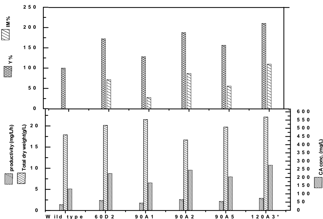
Figure 2: Comparative screening of mutants with wild type for clavulanic acid production IM %: production improvement percentage, Y %: clavulanic acid yield percentage; *selected strain
