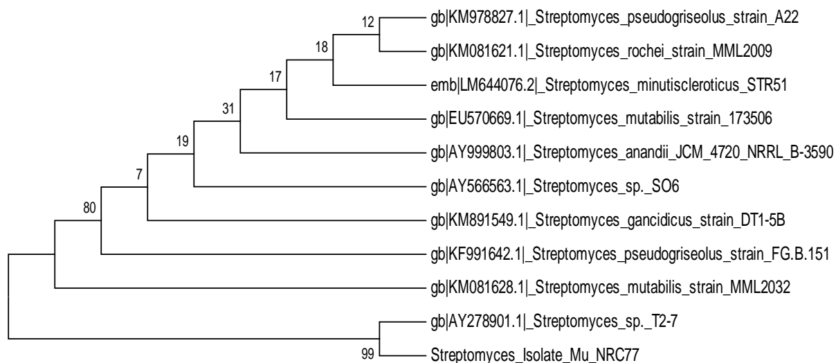
Figure 4: Phylogenetic tree showing the position of Streptomyces sp. Mu-NRC77, Neighbor-joining method
