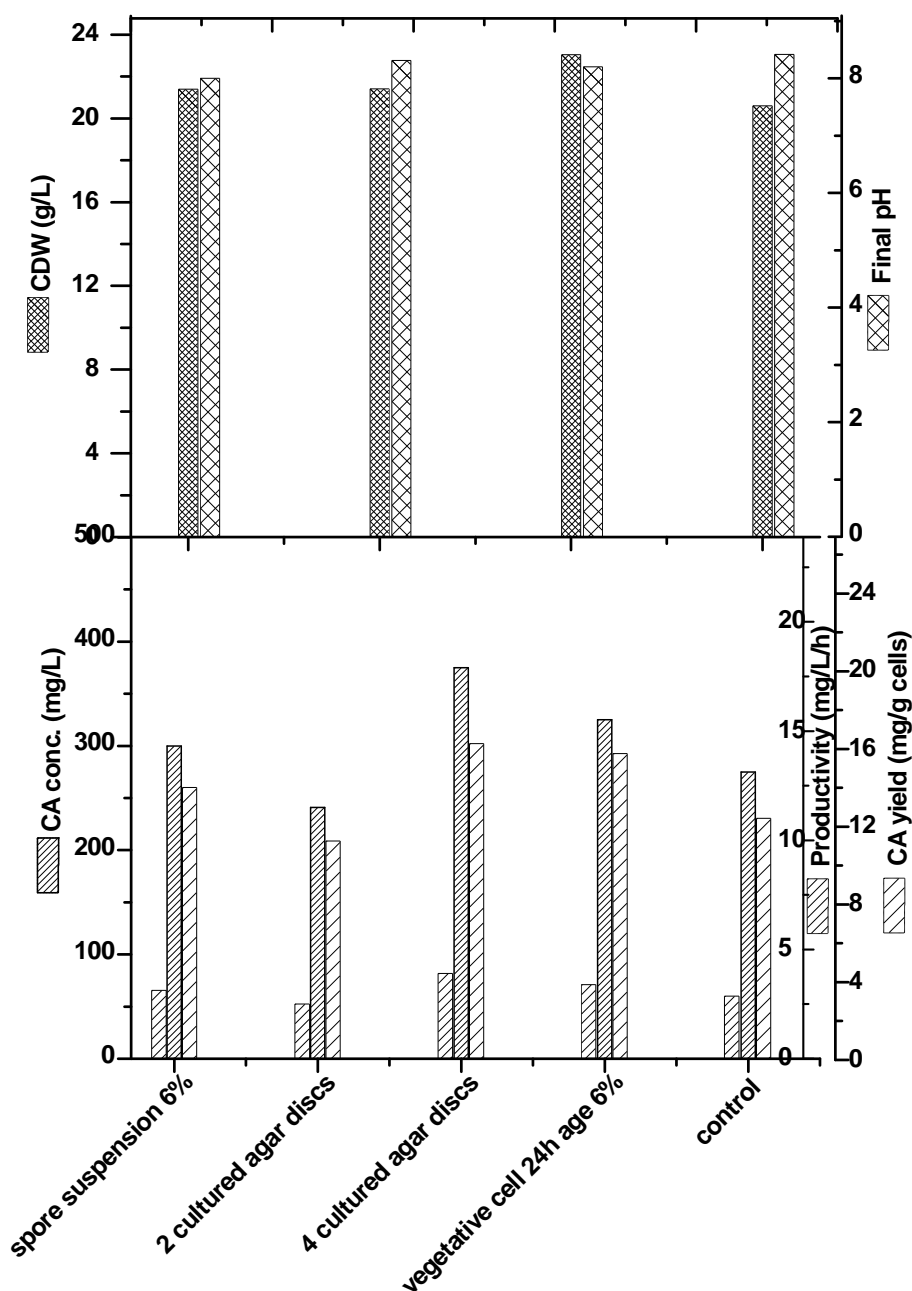
Figure 6: Effect of different inoculum type and size on cell growth and clavulanic acid production by Streptomyces sp. MU-NRC77
