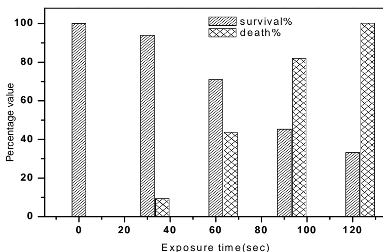
Figure 1: Effect of UV radiation on the growth of Streptomyces sp. NRC 77
