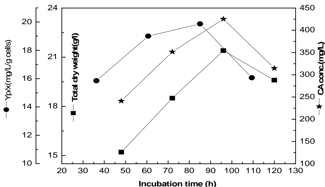
Figure 5: The effect of incubation period on cell growth and clavulanic acid production by Streptomyces sp. MU-NRC77
