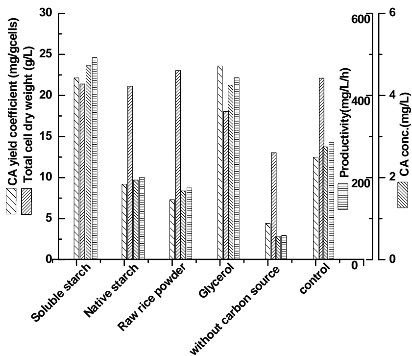
Figure 7: The effect of different carbon source on cell growth & clavulanic acid production by Streptomyces sp. MU-NRC77
