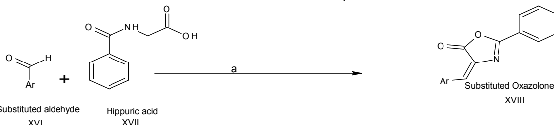
Scheme 4: (g) CH 3 COONa, CH 3 COOH, 2 h (XVIIIa. 52.12 %, XVIIIb. 55.13 %, XVIIIc. 69.13 %, XVIIId. 63.18 %, XVIIIe. 48.19 %, XVIIIf. 64.85 %)
