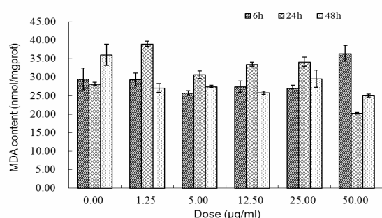
Fig 6: Effects of C. ambrosioides essential oil treatment on MDA content in MCF-7 cells
