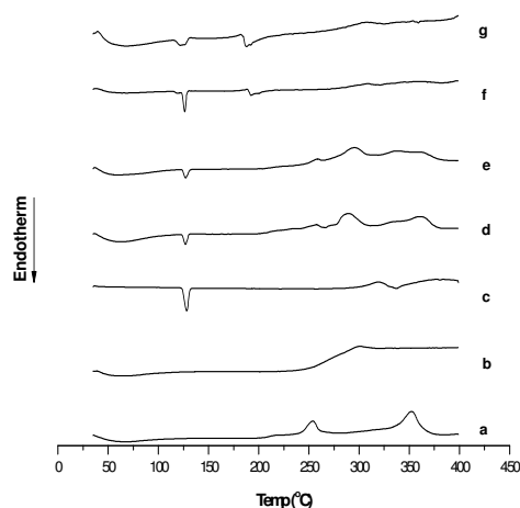
Figure 4: DSC thermograms of sodium alginate (a), chitosan (b), nimodipine (c), physical mixture of nimodipine with sodium alginate (d), physical mixture of nimodipine, sodium alginate and chitosan (e), nimodipine-loaded alginate beads (f), and nimodipine-loaded alginate beads coated with chitosan (g)
