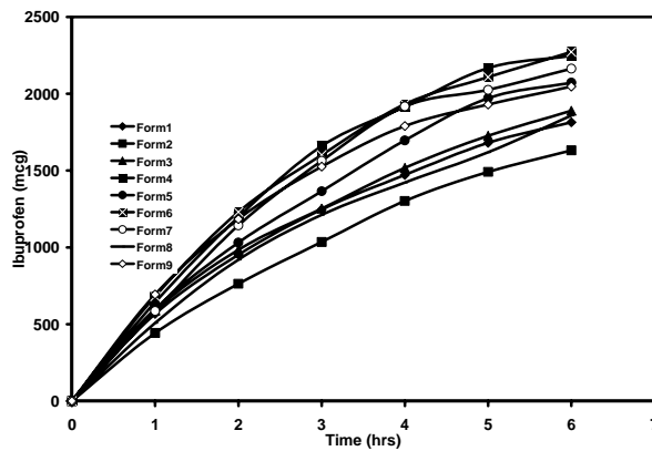
Figure 1: Cumulative drug released from various formulations
