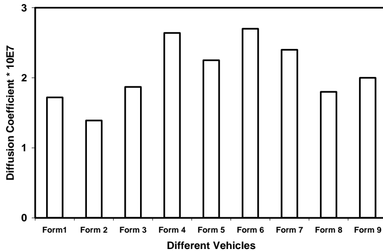
Figure 2: Diffusion coefficient of the ibuprofen from various ointment bases
