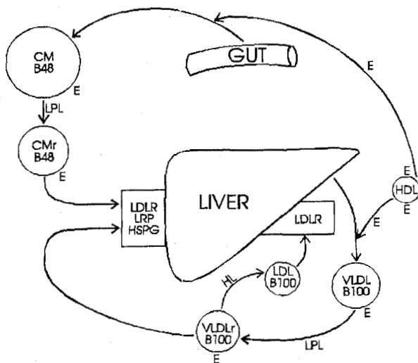
Fig. 1. Schematic representation of remnant lipoprotein metabolism. Chylomicrons (CM) from the gut and hepatic VLDL undergo triglyceride hydrolysis by lipoprotein lipase (LPL) and chylomicron remnants (CMr) and VLDL remnants (VLDLr) are formed. VLDLr can be converted to LDL by hepatic lipase (HL) or can be taken up directly by the liver as is the case with CMr. ApoE mediates binding of remnants to hepatic lipoprotein receptors. The hepatic lipoprotein receptors are the LDL receptor (LDLR), the LDL receptor related protein (LRP) and heparan sulfate proteoglycans (HSPG).
