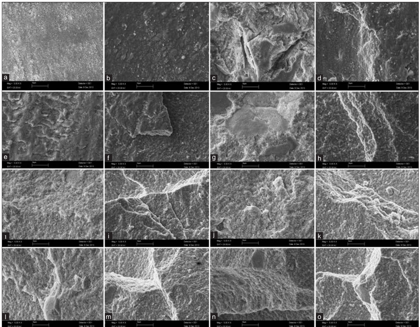
Figure 3: (a) Scanning electron microscopic images of different surface treatments on the surface of ZrO 2 (×5000) (a) No treatment presintered ZrO 2 , (b) After sintering ZrO 2 , (c) Sandblasted presintered ZrO 2 , (d) After sintering ZrO 2 in letter “c”, (e) 1 W laser irradiation presintered ZrO 2 , (f) After sintering ZrO 2 in letter “e”, (g) 2 W laser irradiation pre-sintered ZrO 2 , (h) After sintering ZrO 2 in letter “g”. (b) Scanning electron microscopic images of different surface treatments on the surface of ZrO 2 (×5000) (i) 3 W laser irradiation presintered ZrO 2 , (i) After sintering ZrO 2 in letter “i”, (j) 4 W laser irradiation presintered ZrO 2 , (k) After sintering ZrO 2 in letter “j”, (l) 5 W laser irradiation presintered ZrO 2 , (m) After sintering ZrO 2 in letter “l”, (n) 6 W laser irradiation presintered ZrO 2 , (o) After sintering ZrO 2 in letter “n”
