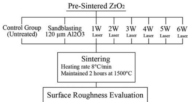
Figure 1: The schematic test protocol
