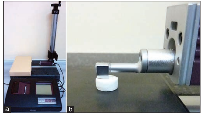
Figure 2: Evaluation of the surface roughness. (a) The photography of the profilometer, (b) measuring surface roughness of the pre-sintered ZrO 2
