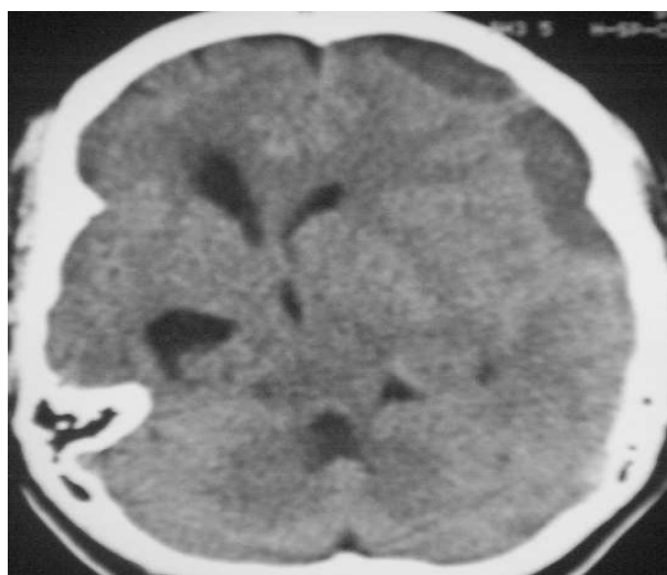
Figure 3: Subdural Effusion/Empyema
