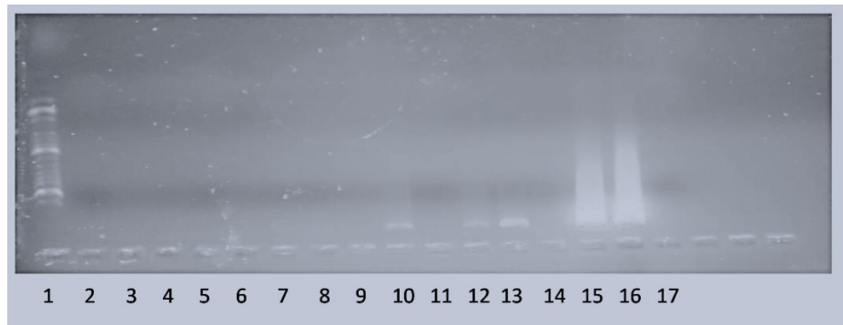
Lane 1: DNA Ladder (50 bp); Lane 2: IP01N (DNA purity @ A_{260}/A_{280} - 1.23; DNA Conc. 1.3 ng/ \mu L); Lane 3: IP07N (DNA purity @ A_{260}/A_{280} - 0.95; DNA Conc. 10.8 ng/ \mu L); Lane 4: IP026N (DNA purity @ A_{260}/A_{280} - 1.3; DNA Conc. 0.14 ng/ \mu L); Lane 5: IP35N (DNA purity @ A_{260}/A_{280} - 3.1; DNA Conc. 0.04 ng/ \mu L); Lane 6: IP62N (DNA purity @ A_{260}/A_{280} - 1.9; DNA Conc. 2.3 ng/ \mu L); Lane 7: IP95S (DNA purity @ A_{260}/A_{280} - 1.0; DNA Conc. 5.9 ng/ \mu L); Lane 8: IP101N (DNA purity @ A_{260}/A_{280} - 1.2; DNA Conc. 1.2 ng/ \mu L); Lane 9: IP128H (DNA purity @ A_{260}/A_{280} - 1.1; DNA Conc. 0.97 ng/ \mu L); Lane 10: IP147N (DNA purity @ A_{260}/A_{280} - 1.2; DNA Conc. 5.8 ng/ \mu L); Lane 11: IP157H (DNA purity @ A_{260}/A_{280} - 8.1; DNA Conc. 6.1 ng/ \mu L); Lane 12: IP178S (DNA purity @ A_{260}/A_{280} - 1.4; DNA Conc. 1.8 ng/ \mu L); Lane 13: IP189N (DNA purity @ A_{260}/A_{280} - 1.8; DNA Conc. 4.7 ng/ \mu L); Lane 14: IP209N (DNA purity @ A_{260}/A_{280} - 2.0; DNA Conc. 1.1 ng/ \mu L); Lane 15: Nm ATCC (DNA purity @ A_{260}/A_{280} - 1.5; DNA Conc. 15.1 ng/ \mu L); Lane 16: Hi ATCC (DNA purity @ A_{260}/A_{280} - 1.48; DNA Conc. 20.0 ng/ \mu L); Lane 17: Sp ATCC (DNA purity @ A_{260}/A_{280} - 1.6; DNA Conc. 16.6 ng/ \mu L)
