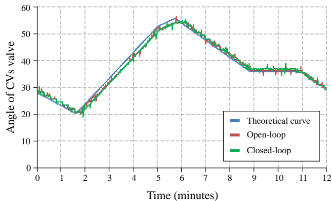
Figure 6 Opening curves of CVs valve
