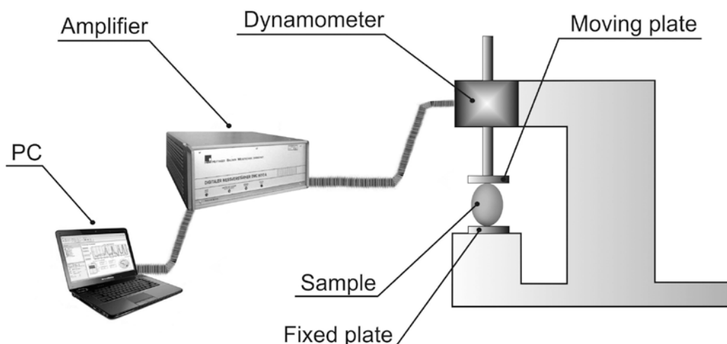
Figure 1 Schematic presentation of universal testing machine used to measure the rupture forces
