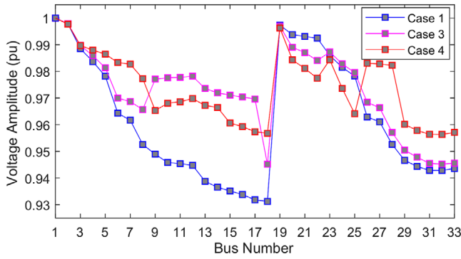
FIGURE 6 Comparison of voltage amplitudes in deterministic test studies
