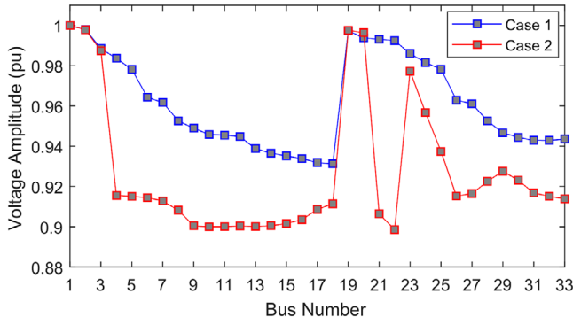
FIGURE 5 Comparison of the voltage amplitudes in cases 1 and 2
