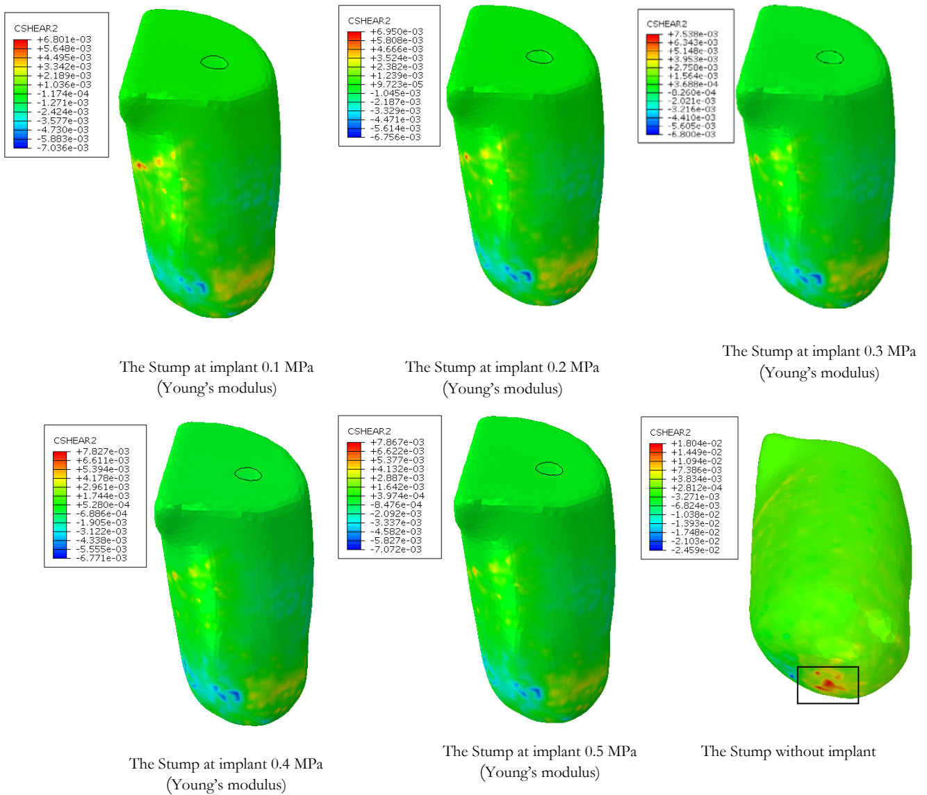
Figure 7: Longitudinal shear stress distributio (MPa) on the stump-prosthetic interface for all implant stiffness cases and the case without implant.
