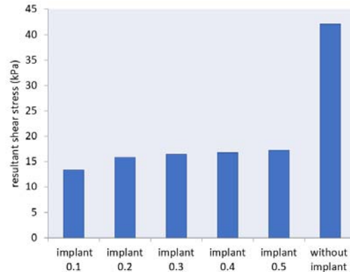
Figure 9: Resultant shear stress (kPa) on the stump-prosthetic interface for all implant stiffness cases and the case without implant.
