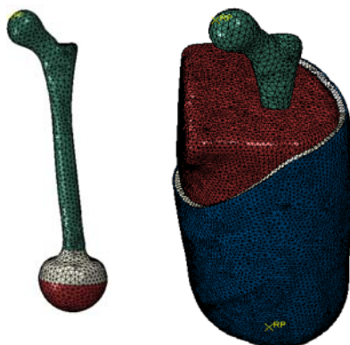
Figure 4: Mesh of the analyzed (FE) model
