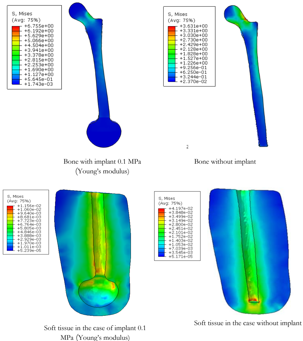
Figure 5: Von Mises stress distribution (MPa) on the limb with and without implant
