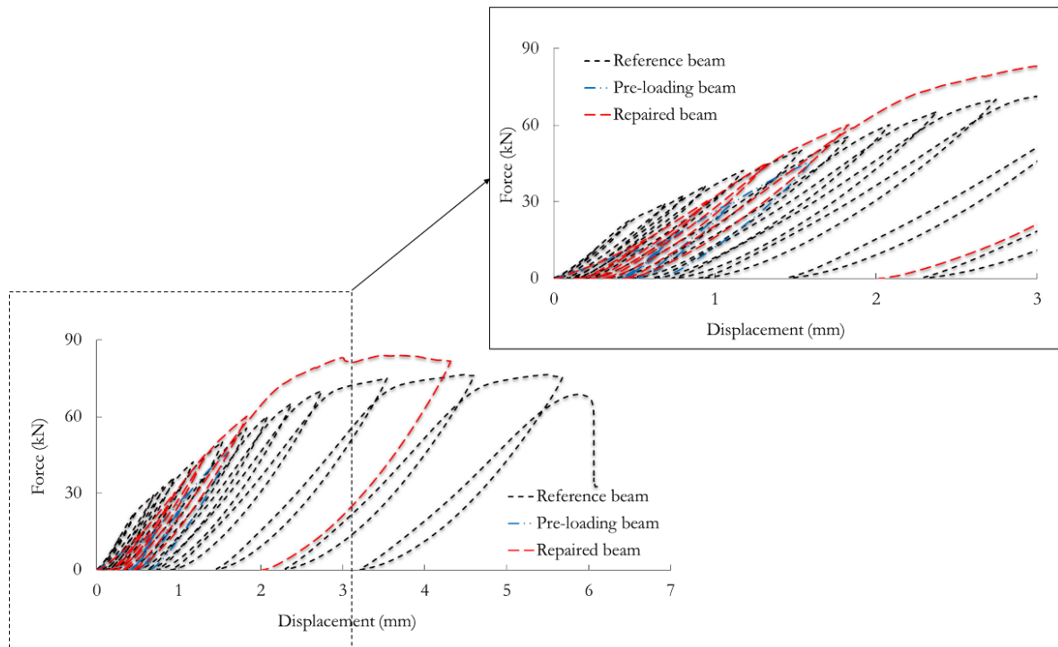
Figure 10: Beam #3.
