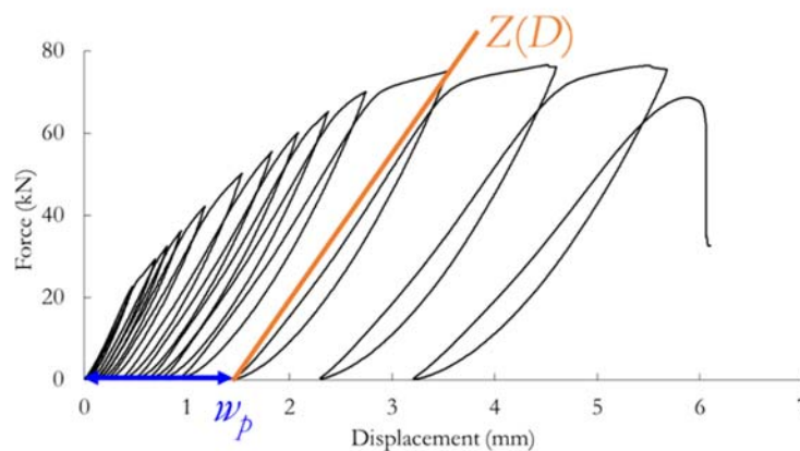
Figure 5: Graphical representation of damage measurement.
