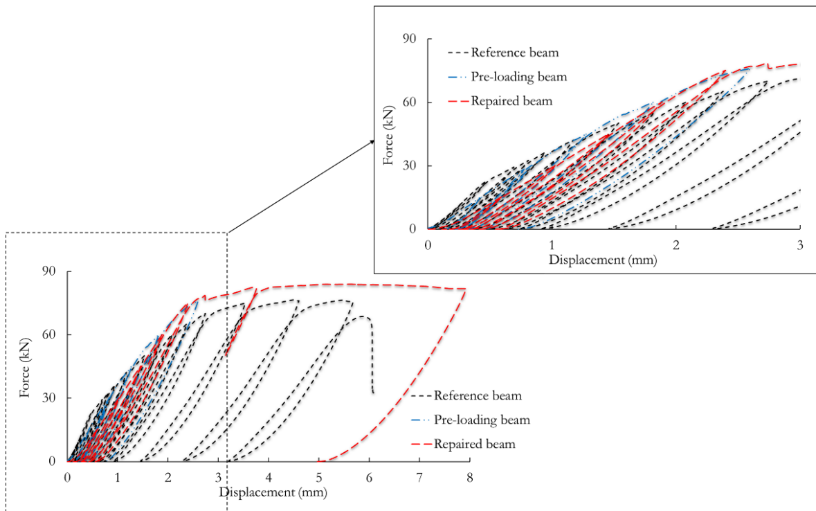
Figure 8: Beam #1.
