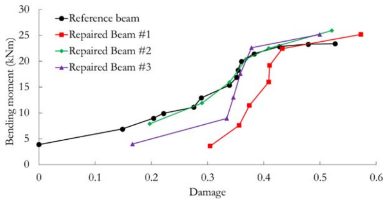
Figure 7: Bending moment and damage values at each cycle.
