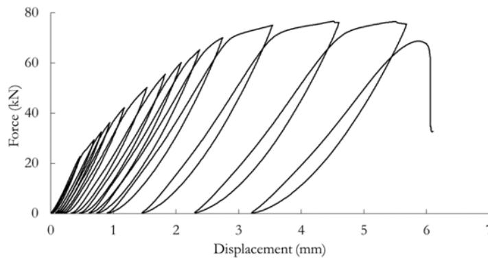
Figure 6: Force-displacement response of the reference beam.
