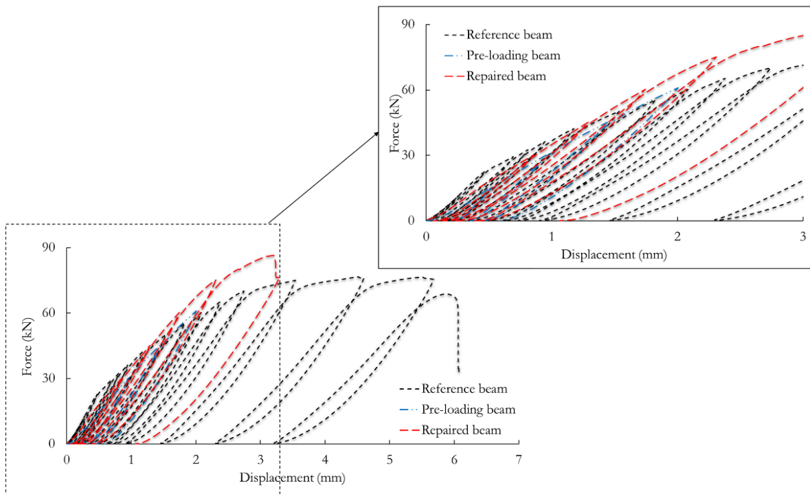
Figure 9: Beam #2.
