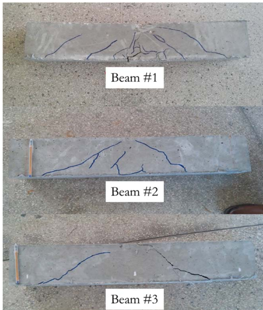
Figure 11: Cracking pattern of the repaired beams.
