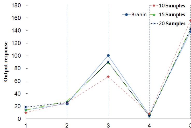
Figure 5: The error at the check points.
