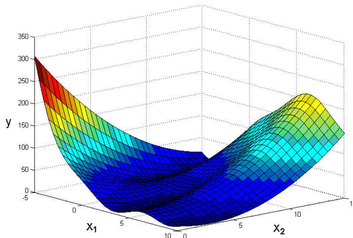
Figure 3: The 3 dimensional plot of Branin function.
