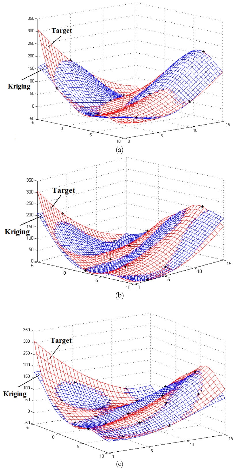
Figure 4: The Kriging model for Branin Function for different number of samples: (a) 10 samples, (b) 15 samples, (c) 20 samples.
