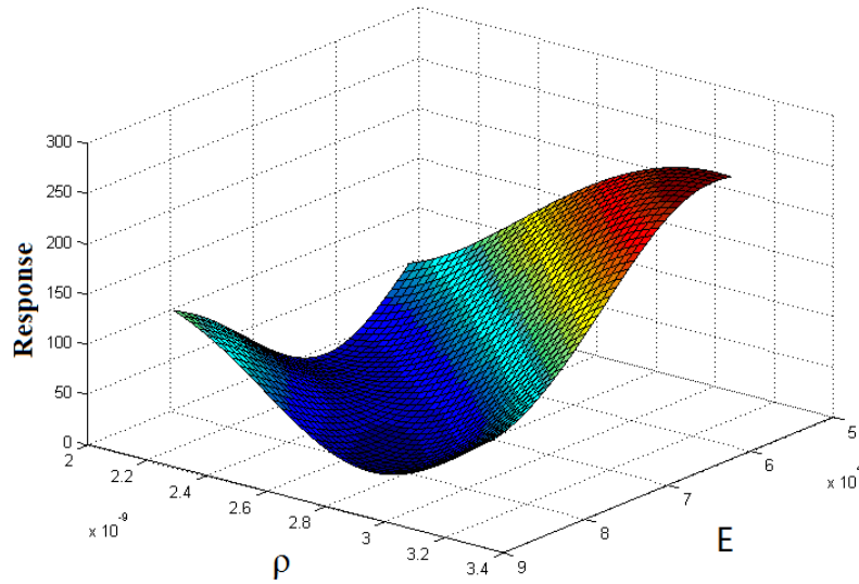
Figure 10: The Kriging model in (E, \rho ) dimension
