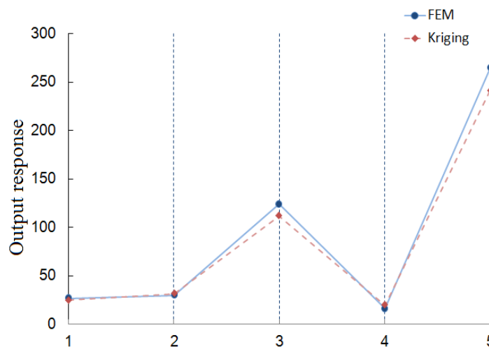
Figure 11: The error at checking points.
