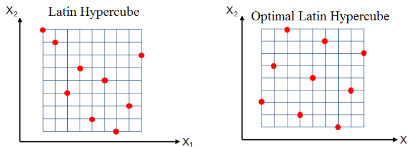
Figure 2: The comparison of Latin Hypercube to OLH.
