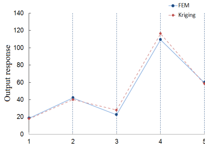
Figure 9: The error at check points.
