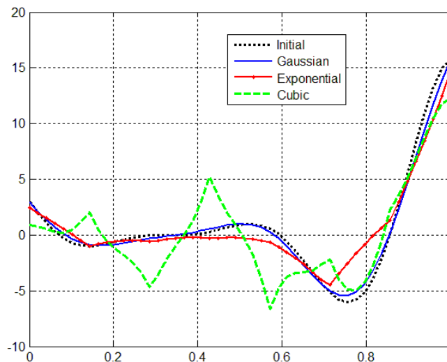
Figure 1: The approximation result by Kriging model using different correlation functions.
