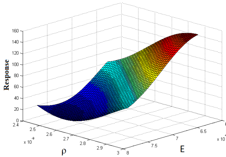
Figure 8: The Kriging model in (E, \rho ) dimension.
