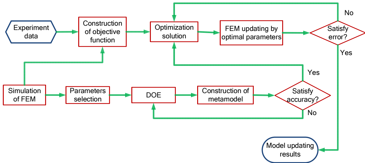
Figure 6: Flow chart of the process of model updating.
