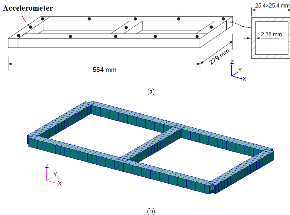
Figure 7: The frame structure: (a) The frame geometry for experiment, (b) The FEM.
