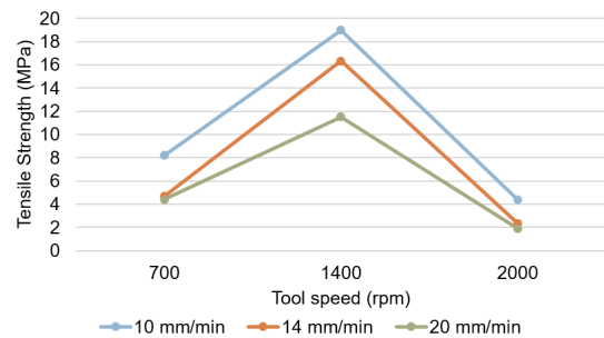
Figure 9: Effect of tool rotational speed on tensile strength.
