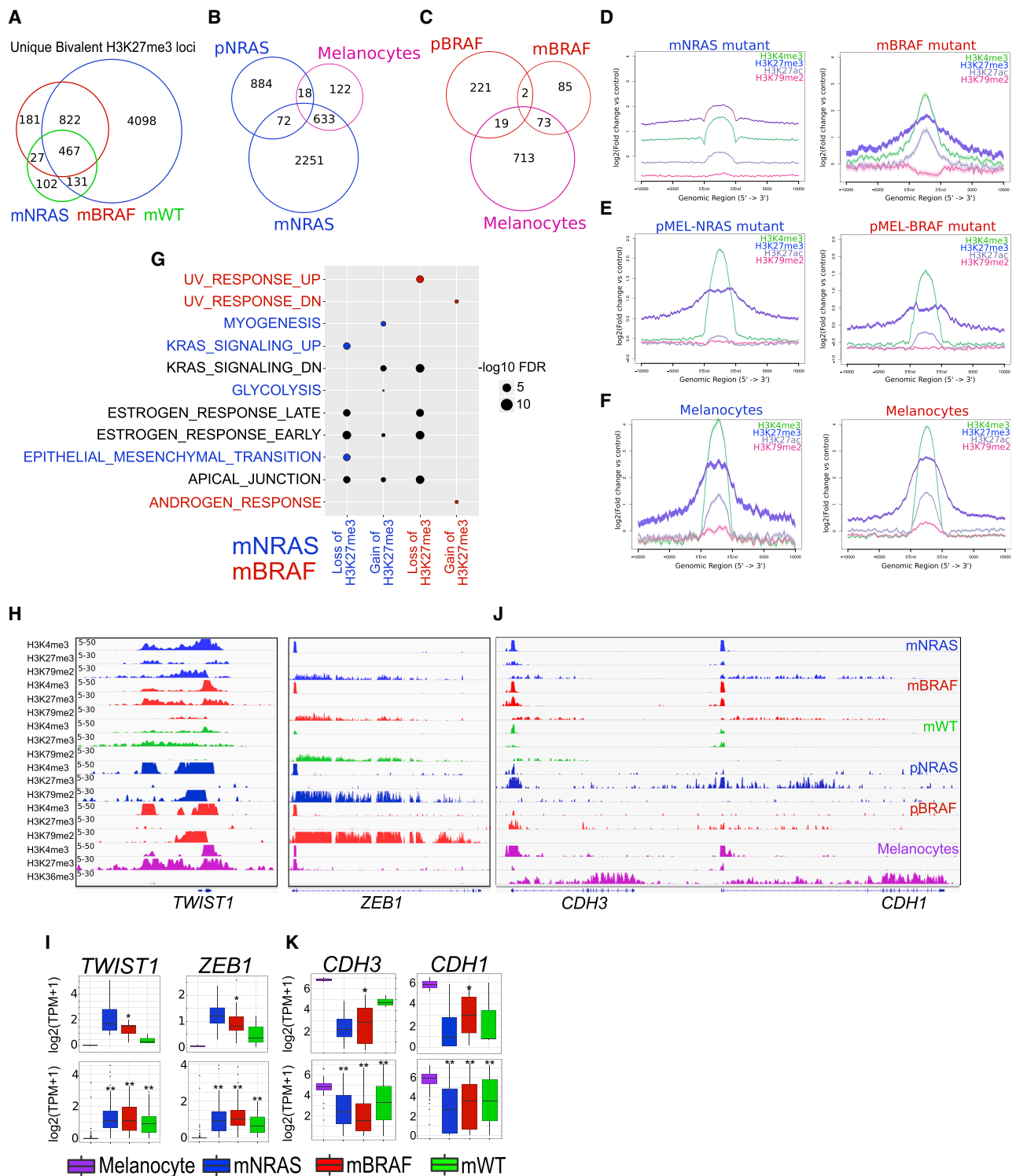
Figure 2. Bivalent domains are lost and gained on mesenchymal genes
