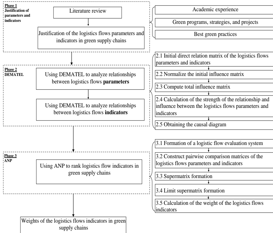
Fig. 3 Algorithm of the combined DEMATEL-ANP method for evaluating the parameters and indicators of logistics flows in green supply chains
