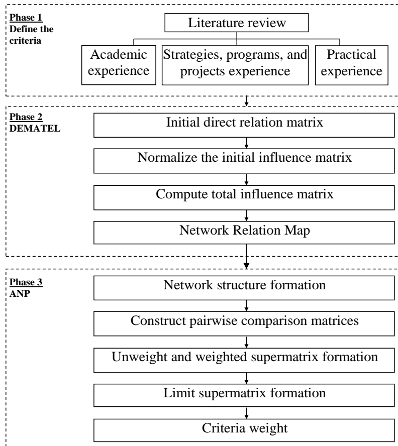
Fig. 2 Combined DEMATEL-ANP algorithm
