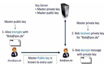
Fig 3.1 Identity-Based Encryption
