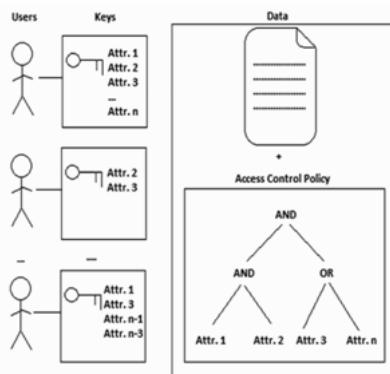
Fig 3.3 Ciphertext-policy attribute-based encryption
