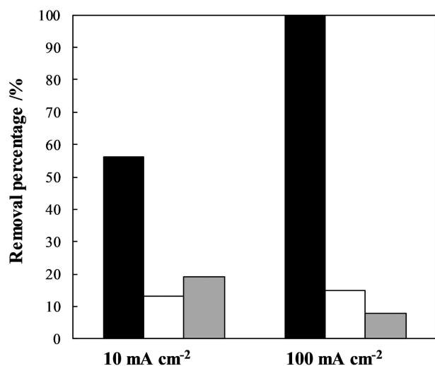
Figure 2. Removal percentage of uric acid (■), urea (□) and creatinine (●) during the electrolysis of penicillin G solutions in urine media. Electric charge passed: 1.5 \text{ Ah dm}^{-3} at 10 \text{ mA cm}^{-2} and 2.5 \text{ Ah dm}^{-3} at 100 \text{ mA cm}^{-2} .
