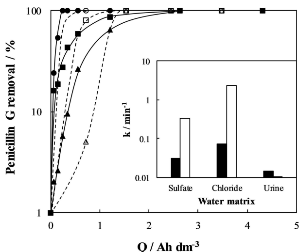
Figure 1. Influence of the current density on penicillin G removal as function of the applied electric charge during the electrolysis with diamond anodes. C_0 : 100 \text{ mg dm}^{-3} . (■) 2000 \text{ mg dm}^{-3} \text{ Na}_2\text{SO}_4 ; (●) 2000 \text{ mg dm}^{-3} \text{ NaCl} ; (▲) urine. Black symbols: 10 \text{ mA cm}^{-2} ; white symbols 100 \text{ mA cm}^{-2} .
