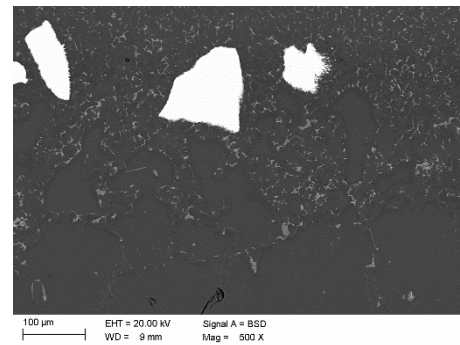
Fig. 14. The surface layer of AlSi9Cu alloy after melting the ceramic powder, laser power 1.5 kW, 1.5 g/min, remelting rate 0.25 m/min
