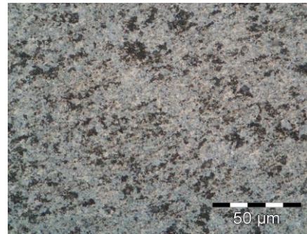
Fig. 3. Ceramic Matrix Composite F1200, with aluminium oxide matrix reinforced B 4 C [the authors own work]
