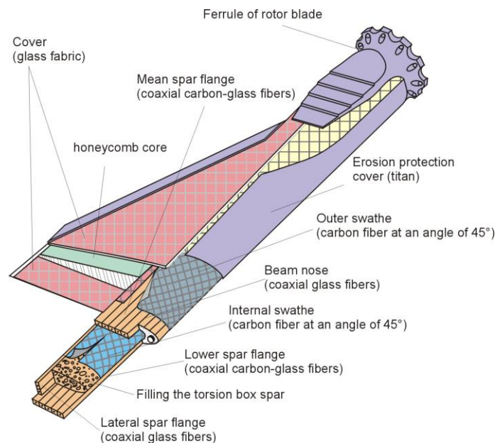
Fig. 9. Rotor blade of a modern helicopter [16]
