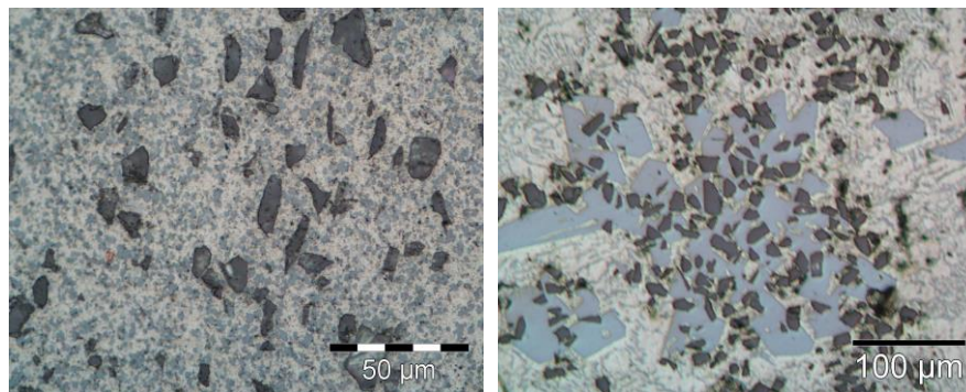
Fig. 4. Examples of Metal Matrix Composites a) ASCM alloy+SiC9%; b) AlSi25+SiC20% [the authors own work]
