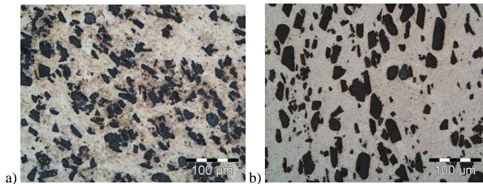
Fig. 10. Composite materials a) Duralcan W6A-15A, b) Duralcan W6A-20A [the authors own work]
