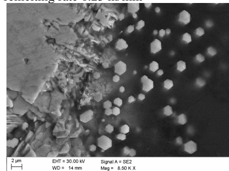
Fig. 16. Boundary of the powder-Al matrix of surface layer of AlSi9Cu alloy after melting the ceramic powder, laser power 2.0 kW, 8.0 g/min, remelting rate 0.25 m/min
