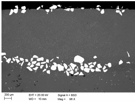
Fig. 11. The surface layer of AlSi9Cu alloy after melting the ceramic powder, laser power 2.0 kW, 1.5 g/min, remelting rate 0.25 m/min
