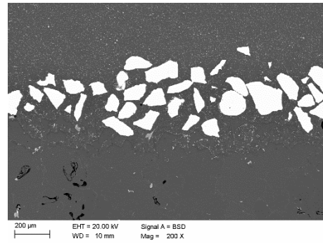
Fig. 12. The surface layer of AlSi9Cu alloy after melting the ceramic powder, laser power 2.0 kW, 1.5 g/min, remelting rate 0.25 m/min
