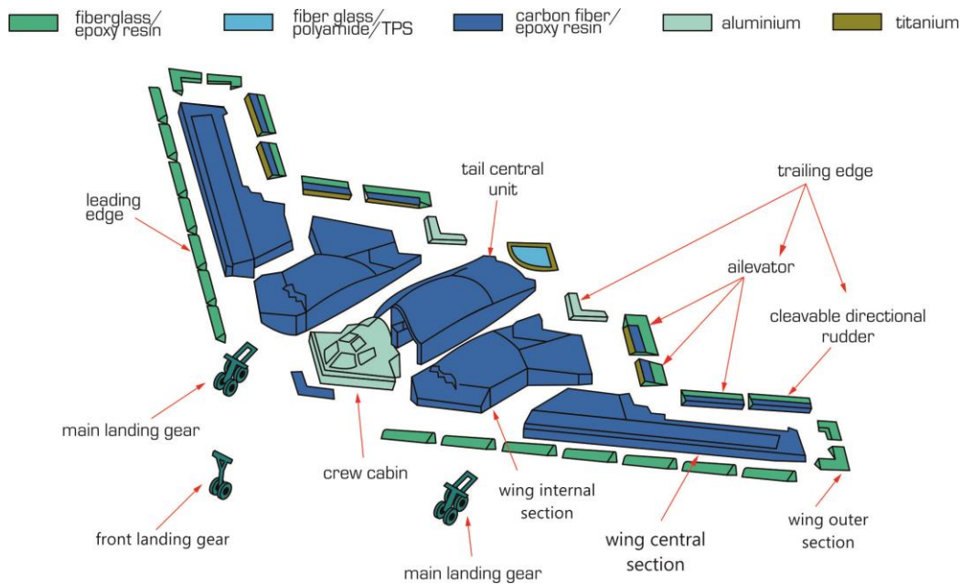
Fig. 7. Bomber B-2 Spirit of the stealth class [16]
