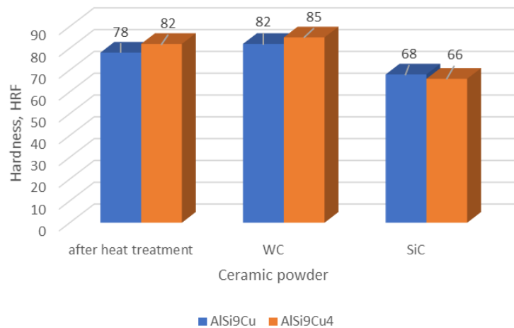
Fig. 17. Results of hardness measurements of samples from Al-Si-Cu casting aluminium after laser fusing
