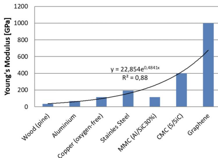
Fig. 19. Comparison of Young's modulus of basic construction materials used for aircraft construction based on [27-29]
