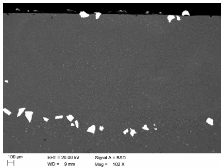
Fig. 13. The surface layer of AlSi9Cu alloy after melting the ceramic powder, laser power 1.5 kW, 1.5 g/min, remelting rate 0.25 m/min
