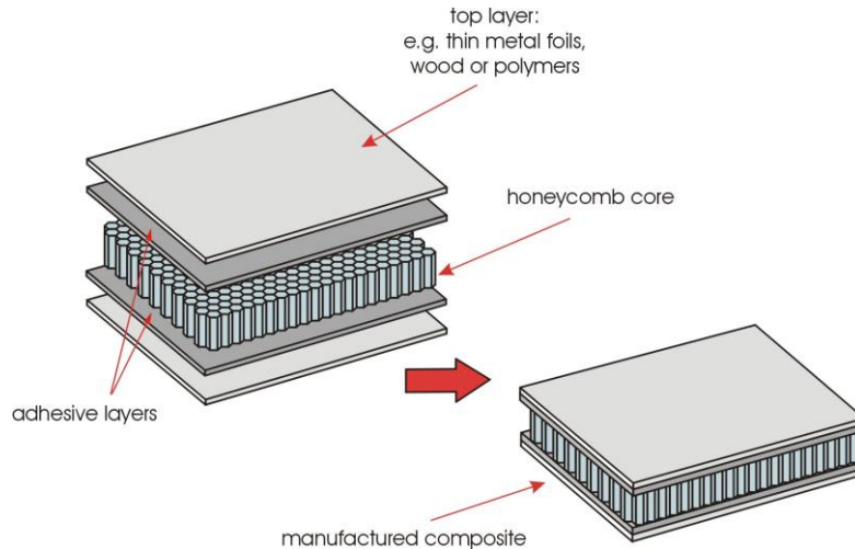
Fig. 1. Layers of the structure of a lightweight composite with a honeycomb core used on aircraft plating [5]
