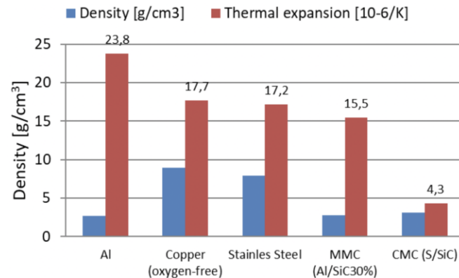
Fig. 18. Comparison of density and thermal expansion of construction materials used for aircraft construction; based on [27-29]
