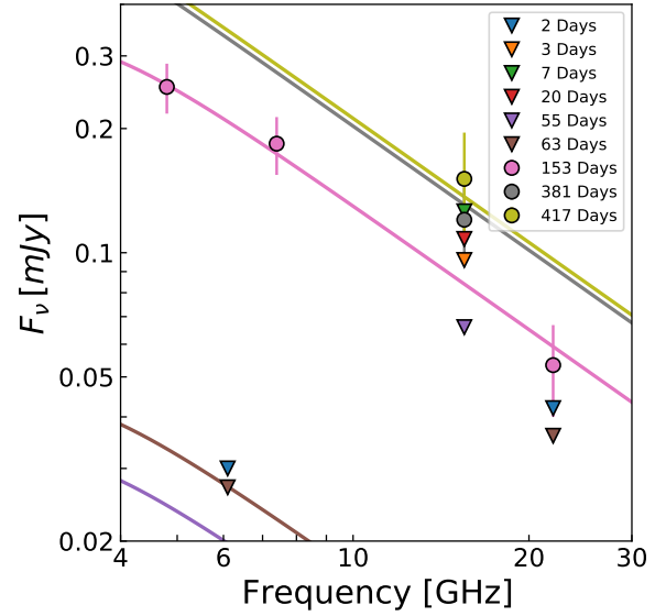
Figure 3. A fitted model for the radio emission originating from an outflow launched promptly after the stellar disruption and interacting with a CNM consisting of a varying two power-law density structure. In contrast to the single power-law CNM model presented in Figure 2, this model is consistent with both the radio detections and non-detections. However, this model is somewhat at odds with the CNM profiles that are usually found in other TDEs (see text for details). Triangles represent 3\sigma upper limits while circles represent the flux density level of detected emission.
