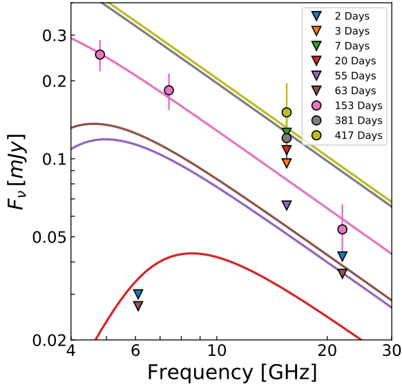
Figure 2. A fitted model for the radio emission originating from an outflow launched promptly after the stellar disruption and interacting with a CNM consisting of a single power-law density structure. This model can account for the VLA and AMI detected emission. However, the upper limit obtained at 63 days (brown triangle) strongly disagrees with the model. Triangles represent 3\sigma upper limits while circles represent the flux density level of detected emission.
