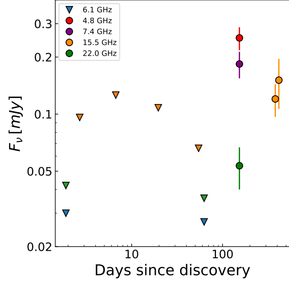
Figure 1. Radio light curves of iPTF16fnl as observed by the VLA and AMI-LA, and reported in §2. Triangles represent 3\sigma upper limits while circles represent the flux density level of detected emission. The color of the triangles and circles refers to the central radio frequency.
