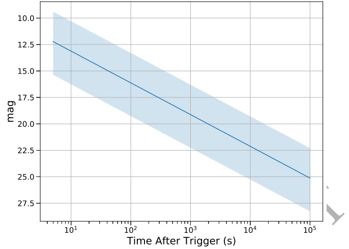
Figure 8. Simulated lightcurve of GRB optical afterglow following power-law decay t^{-1.2} . The shaded region indicates the 1\text{-}\sigma confidence level.
