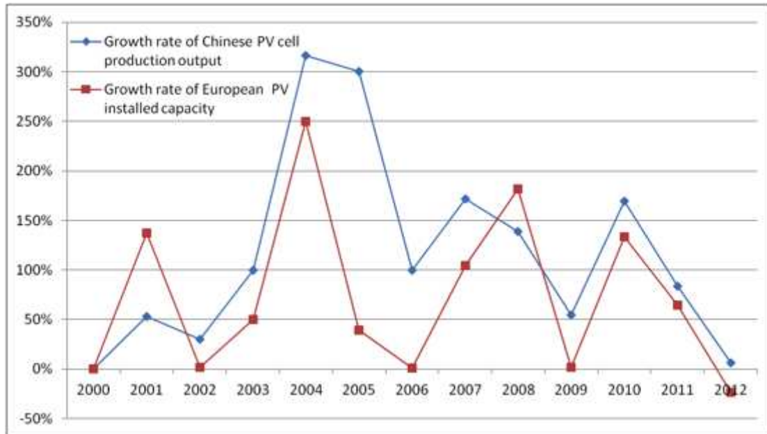
Fig. 6. Comparison of the growth rate of Chinese PV cell production output and European PV installation capacity from 2000 to 2012 (MW p )
