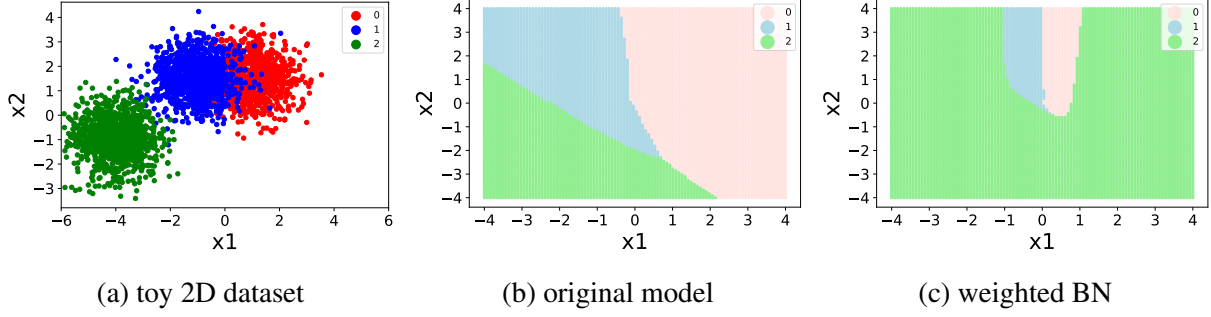
Figure 6.4: Shift of decision boundary using weighted BN
