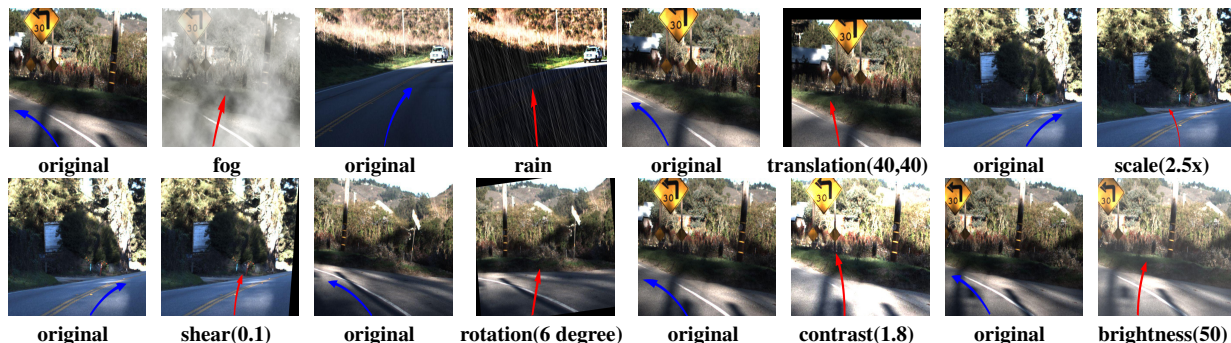
Figure 3.5: Sample images showing erroneous behaviors detected by DeepTest using synthetic images. For original images the arrows are marked in blue , while for the synthetic images they are marked in red . More such samples can be viewed at https://deeplearningtest.github.io/deepTest/ .
