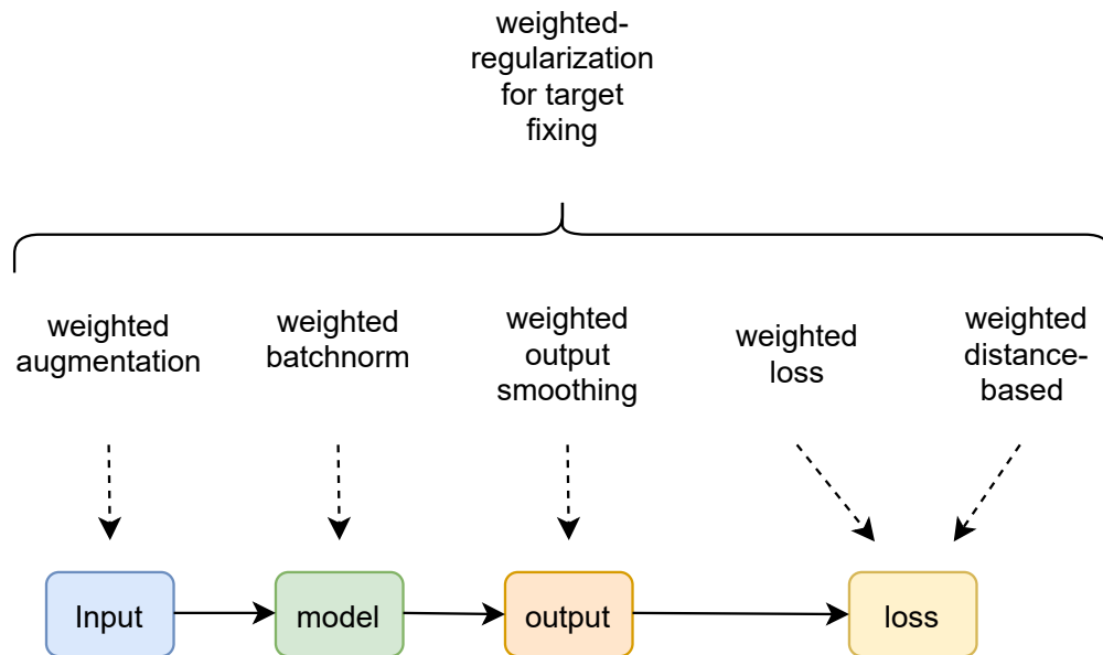
Figure 6.2: Overview of Weighted Regularization for Target Fixing
