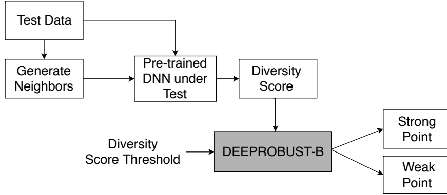
Figure 4.4: Workflow of DEEPROBUST-B
