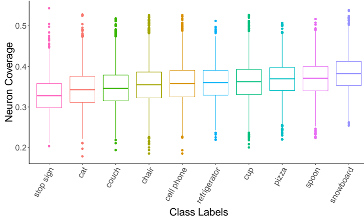
Figure 5.3: Distribution of neuron coverage per class label, for 10 randomly picked class labels, from the COCO dataset.
