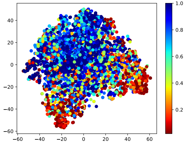
Figure 4.8: The t-SNE plot of correctly classified data points from Self-Driving dataset by the epoch model. data points are colored based on neighbor accuracy.
