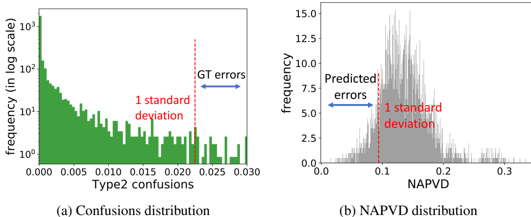
Figure 5.2: Identifying Type2 confusions for multi-classification applications. LHS shows how we marked the ground truth errors based on Type2 confusion score. RHS shows DeepInspect’s predicted errors based on NAPVD score.
