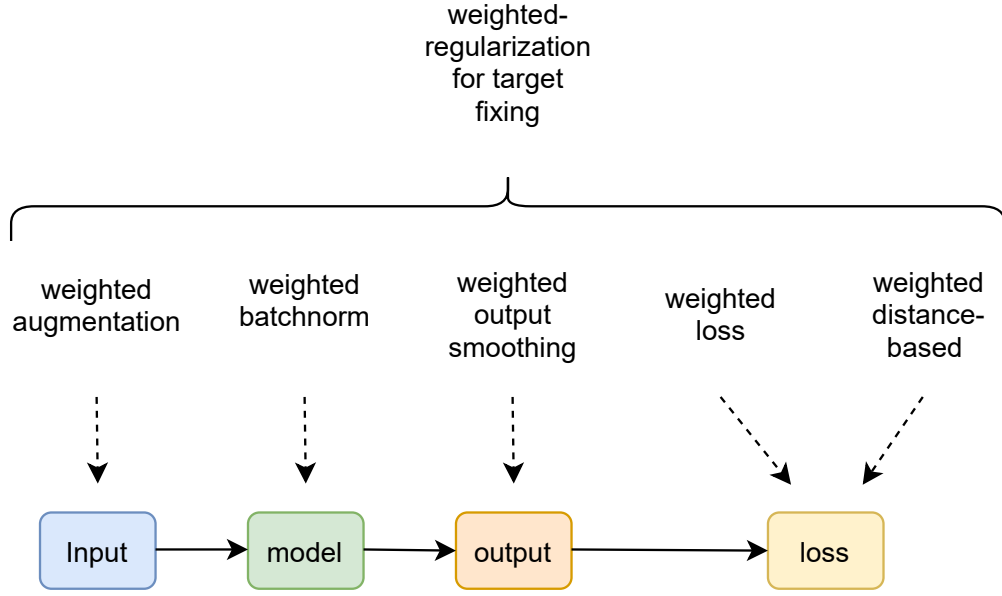
Figure 8: Overview of Weighted Regularization for Target Fixing
