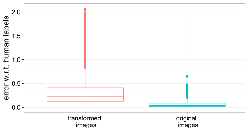
Figure 3.4: Deviations from the human labels for images that violate the metamorphic relation (see Equation 3.2) is higher compared to the deviations for original images. Thus, these synthetic images have a high chance to show erroneous behaviors.
