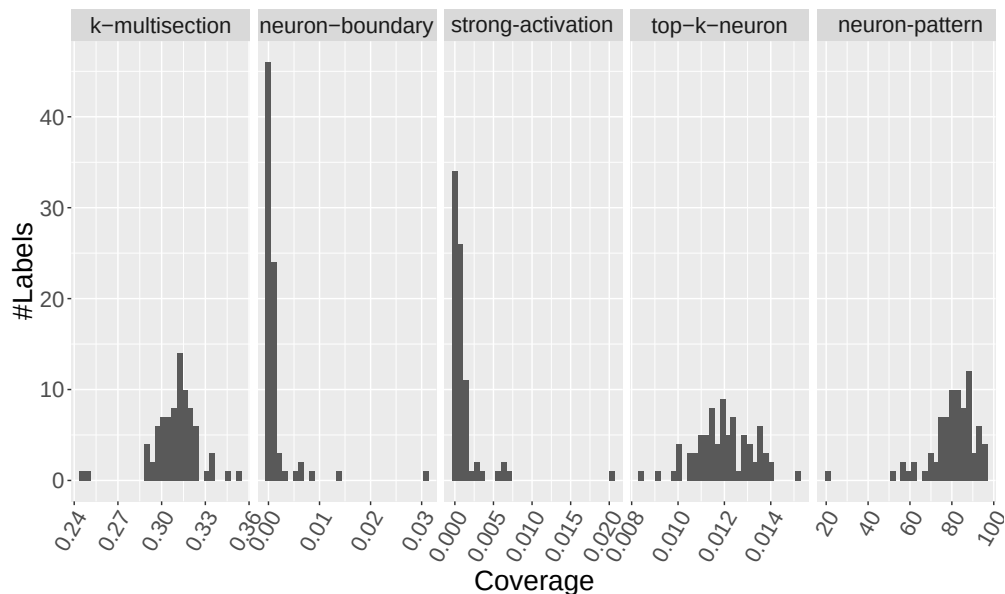
Figure 5.4: Histogram of DeepGauge [50] multi-granular coverage per class label for COCO dataset
