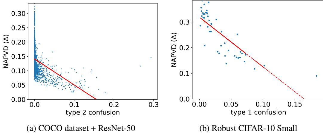
Figure 5.5: Strong negative Spearman correlation (-0.55 and -0.86) between NAPVD and ground truth confusion scores.
