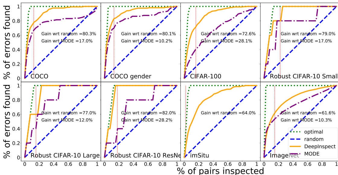
Figure 5.6: AUCEC plot of Type1/Type2 Confusion errors in three different settings. The red vertical line marks 1-standard deviation less from mean NAPVD score. DeepInspect marks all class-pairs with NAPVD scores less than the red mark as potential errors.
