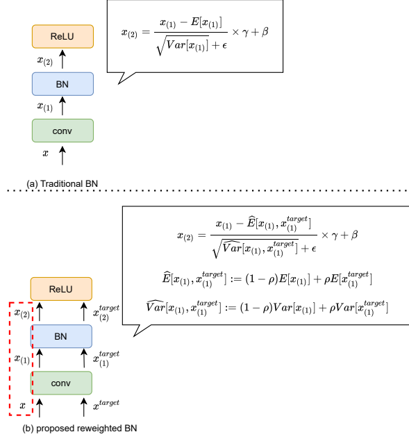
Figure 6.5: Illustration of the traditional BN layer and the proposed weighted BN layer.
