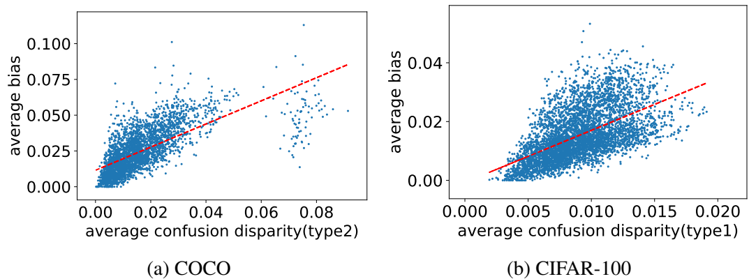
Figure 5.9: Strong positive Spearman’s correlation (0.76 and 0.62) exist between avg_cd and avg_bias while detecting classification bias.
