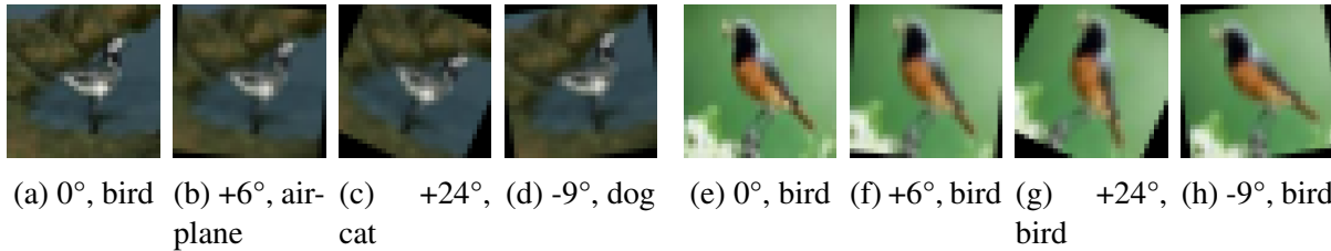
Figure 1: (a)-(d) A well-trained ResNet model [47] misclassifies the rotated variations of a bird image into three different classes though the original un-rotated image is classified correctly. (e)-(h) The same model successfully classifies all the rotated variants of another bird image from the same test set. The sub-captions consist of rotation degrees and the predicted classes.
