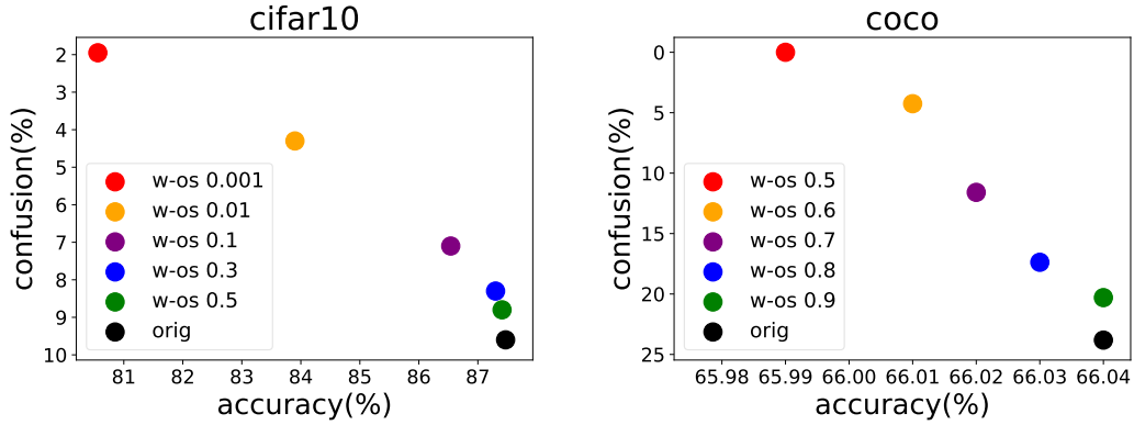
Figure 6.8: Accuracy and Confusion trade-off of different parameters for w-os.
