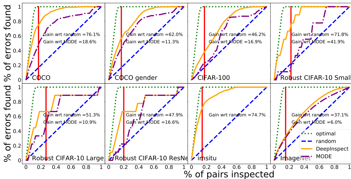
Figure 5.10: Bias errors detected w.r.t. the ground truth of avg_cd beyond one standard deviation from mean.
