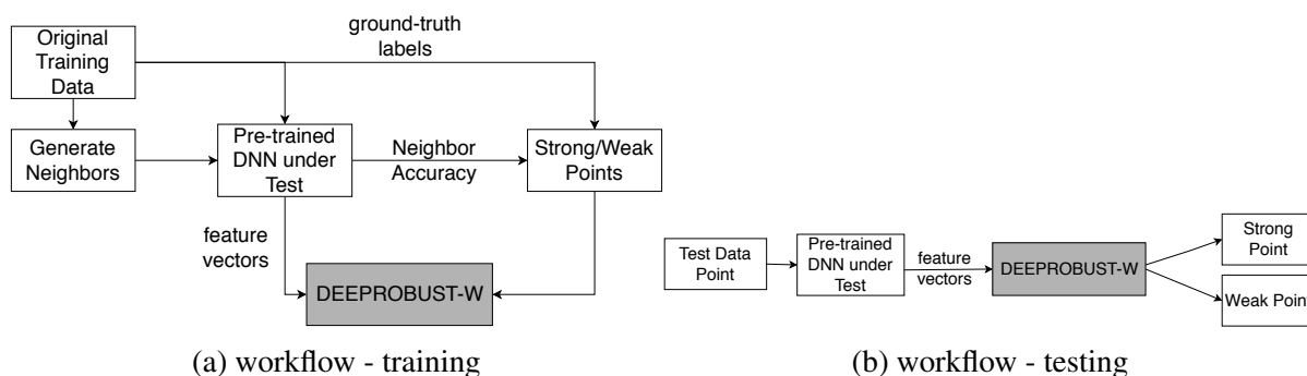
Figure 4.3: Workflow of DEEPROBUST-W
