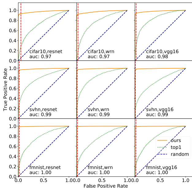
Figure 4.7: AUC-ROC curve with neighbor accuracy cutoff at 0.75. The red vertical line indicates when the diversity score threshold is chosen from training data.
