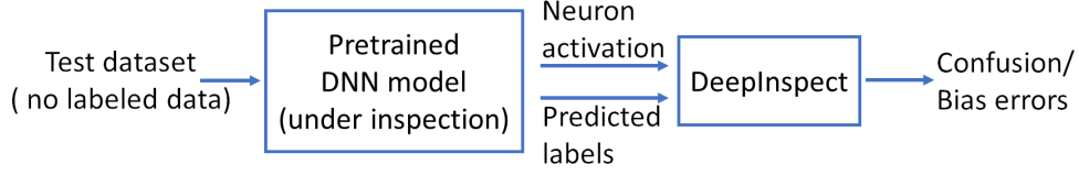
Figure 5.1: DeepInspect Workflow
