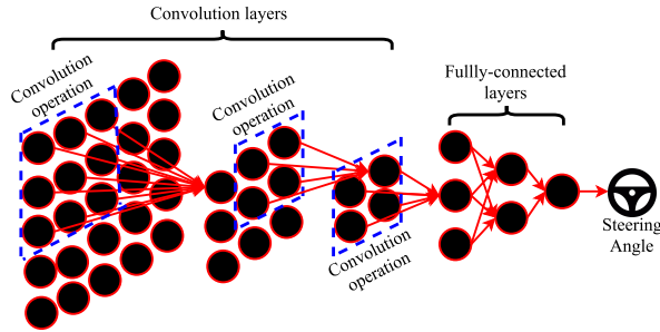
(a) A simplified CNN architecture
