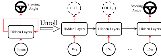
(b) A simplified RNN architecture
