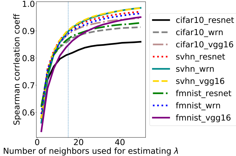
Figure 4.6: The spearman correlation coeff. between diversity score ( \lambda ) and neighbor accuracy, with varying #neighbors ( m ).
