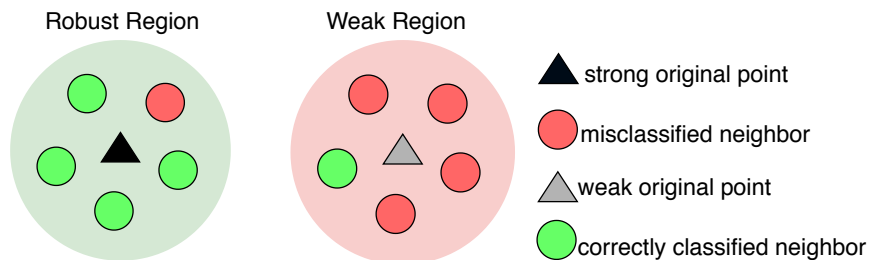
Figure 4.2: Illustrating our terminologies. The triangles are original points, and the small circles are their neighbors generated by natural variations. The light-green region is robust with higher neighbor accuracy, while the light-red region is vulnerable. The corresponding original points are robust and non-robust accordingly.
