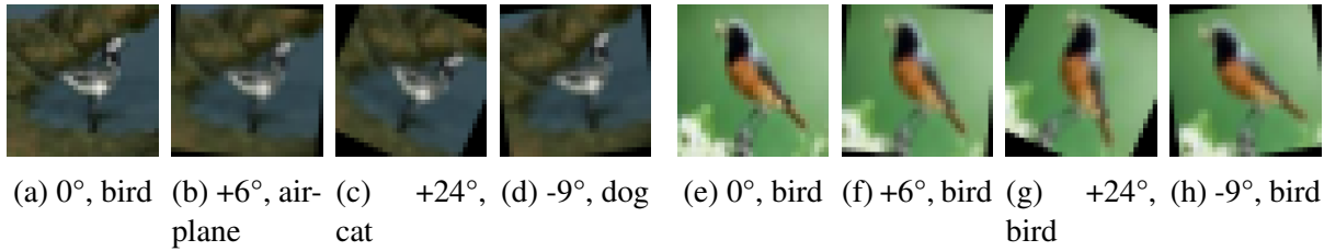
Figure 4.1: (a)-(d) A well-trained Resnet model [47] misclassifies the rotated variations of a bird image into three different classes though the original un-rotated image is classified correctly. (e)-(h) The same model successfully classifies all the rotated variants of another bird image from the same test set. The sub-captions consist of rotation degrees and the predicted classes.
