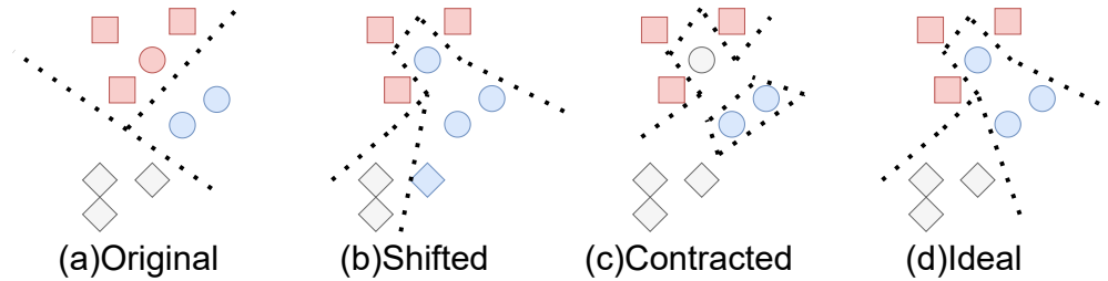
Figure 6.3: Illustration of different potential decision boundary before and after applying WR.
