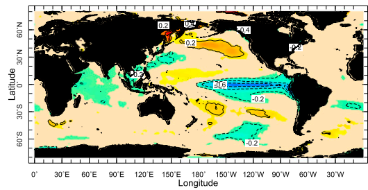
ECHAM5
