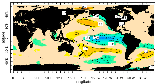
ECHAM4.5
