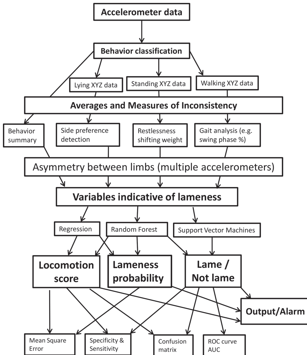
Figure 1. A schematic diagram of how lameness classification could be implemented using accelerometers. This figure is intended to be illustrative of a potential system. Other system configurations are discussed in the text. ROC = receiver operating characteristic; AUC = area under the curve.
