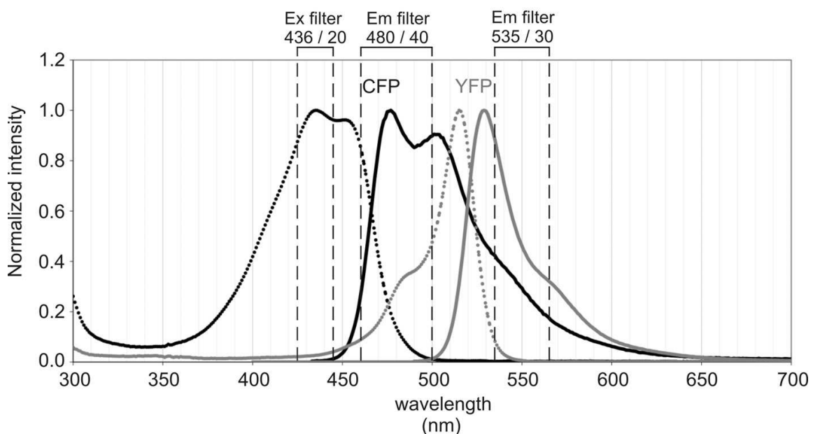
Fig. 9. CFP and YFP excitation and emission spectra. Excitation (dotted line) and emission (solid line) spectra of a CFP and YFP variant including the filters. The normalized spectra shown here have a large overlap. There is overlap in the excitation spectra but also in the emission spectra. Note that CFP covers almost the entire YFP spectrum. The bandpass filters are indicated.
