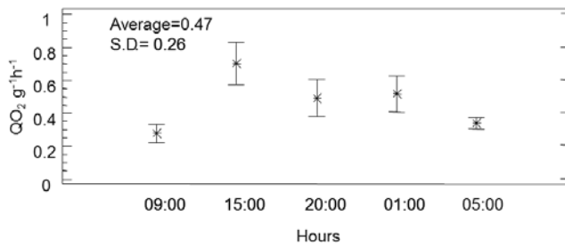
Figure 6. Oxygen consumption in natural condition for H. cyanoguttatus
