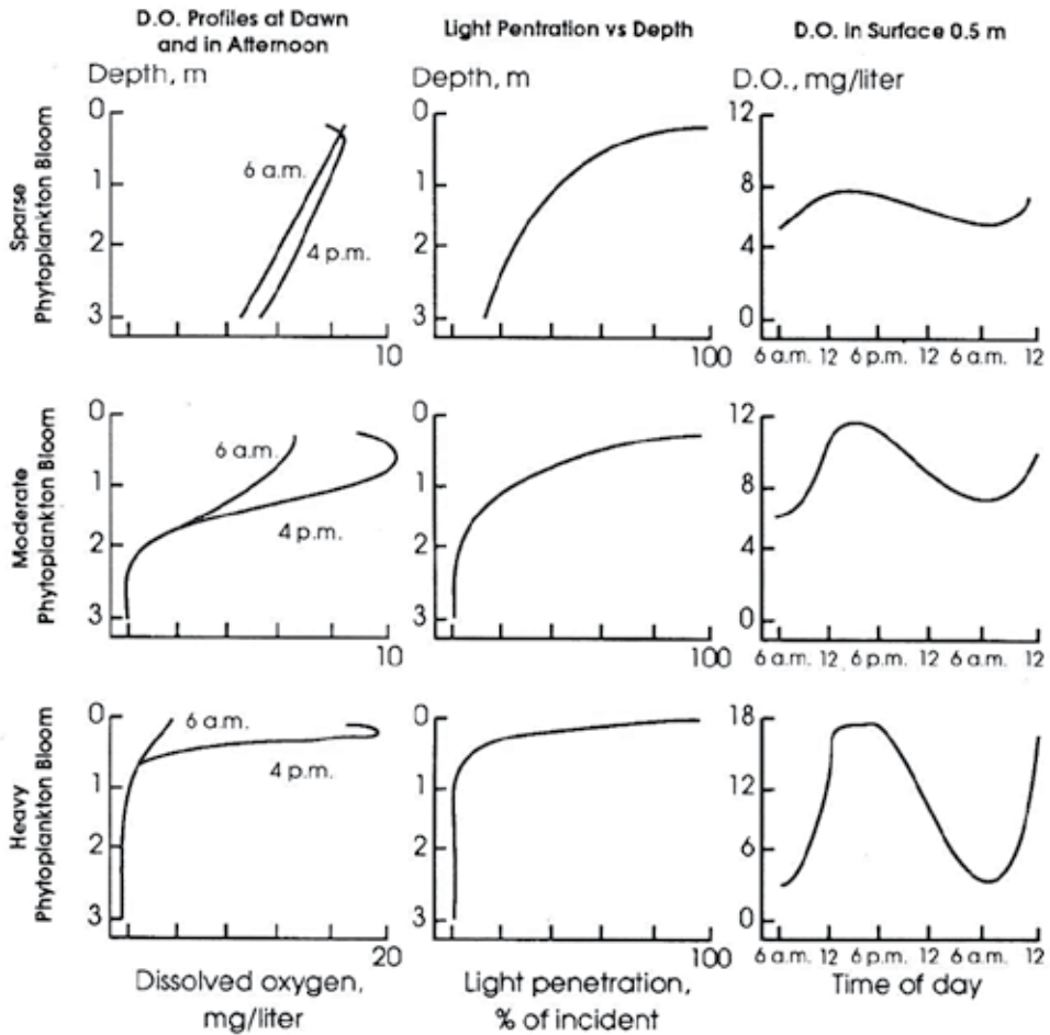
Figure 2. Relationships among phytoplankton density, dissolved oxygen, and light penetration in fish ponds (Boyd 1990).
