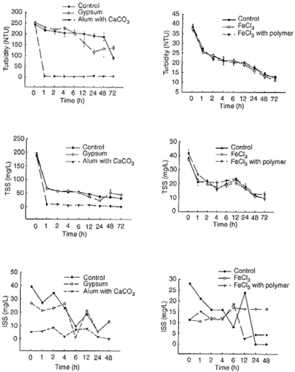
Figure 8. Means ( \pm SE) of turbidity, total suspended solids (TSS), and inorganic suspended solids (ISS) concentrations in alum with agricultural limestone, gypsum, ferric chloride, and ferric chloride with polymer ((polyacrylamide) treated and control over a 72-72 hour sedimentation period, N=3 (Ozbay 2005).
