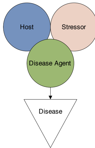
Figure 1. Interactive factors influencing disease in aquaculture (modified from [12]).
