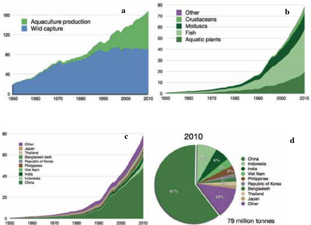
Figure 1. Global harvest of aquatic organisms in millions of tons between 1950-2010 (FAO 2011); b. Global aquaculture production in millions of tons between 1950-2010 (FAO 2011); c. Main aquaculture countries between 1950-2010 (FAO 2011); and d. Main aquaculture countries in 2010 (FAO 2011).
