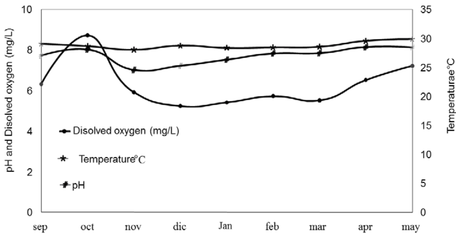
Figure 4. Environmental parameters tendency during an hydrologic cycle in Taxhido river.
