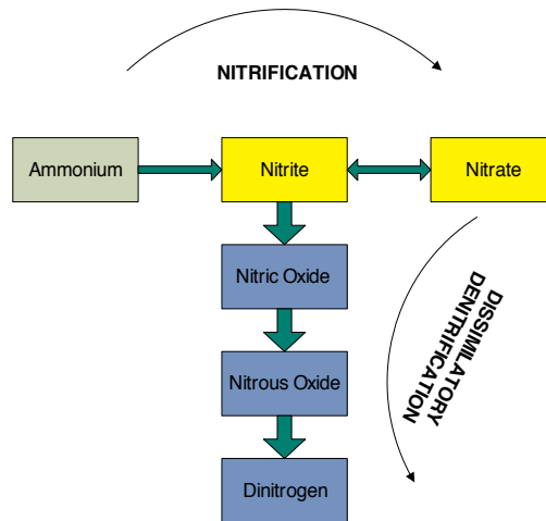
Figure 2. Nitrification and denitrification cycle [30].
