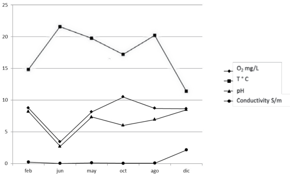
Figure 1. Environmental parameters during a hydrological cycle in San Martín Dam.
