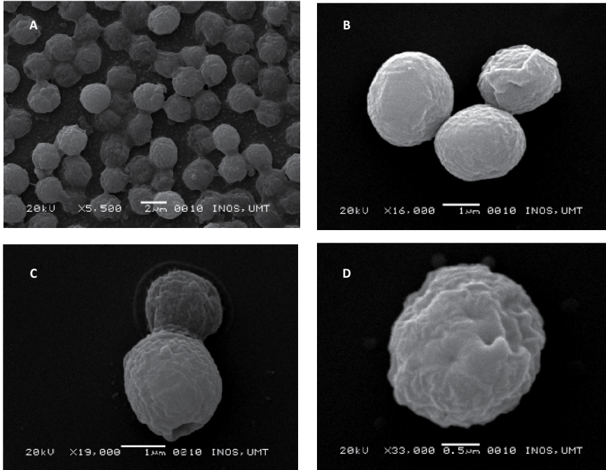
Figure 1. The scanning electron micrographs of C.vulgaris under different views and various magnifications. A, Cell aggregation. B, C.vulgaris cells under different magnification C. Cell division in C.vulgaris . D, Single cell and cell wall structures.
