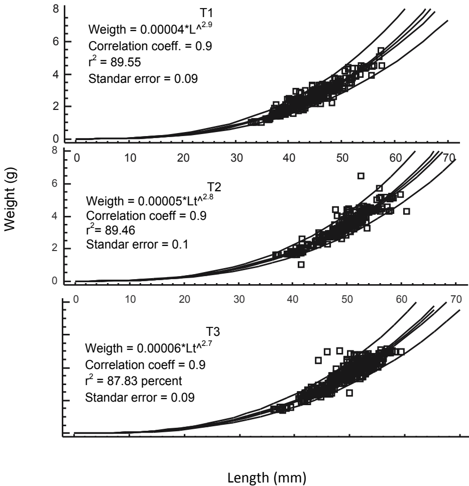
Figure 9. Regression for each one of treatments, values for the equation W=KL^b
