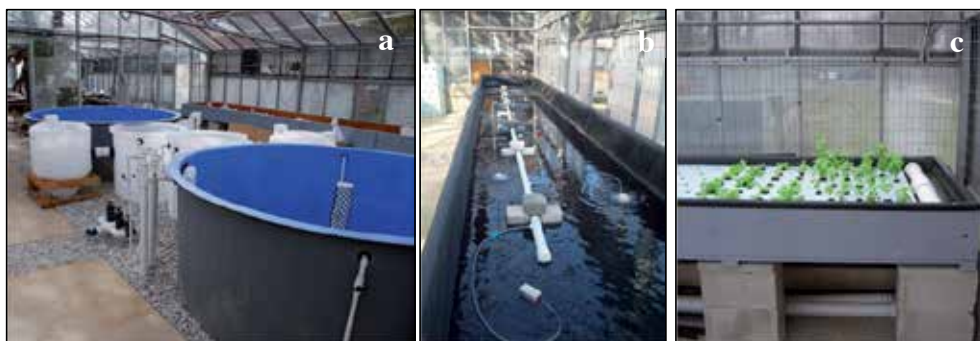
Figure 12. a. Construction of an airlift aquaponics system; b. Aquaponics raft raceway showing aeration for plant roots; c. Planting herbs in a floating Styrofoam sheet (Photos courtesy of Blank).
