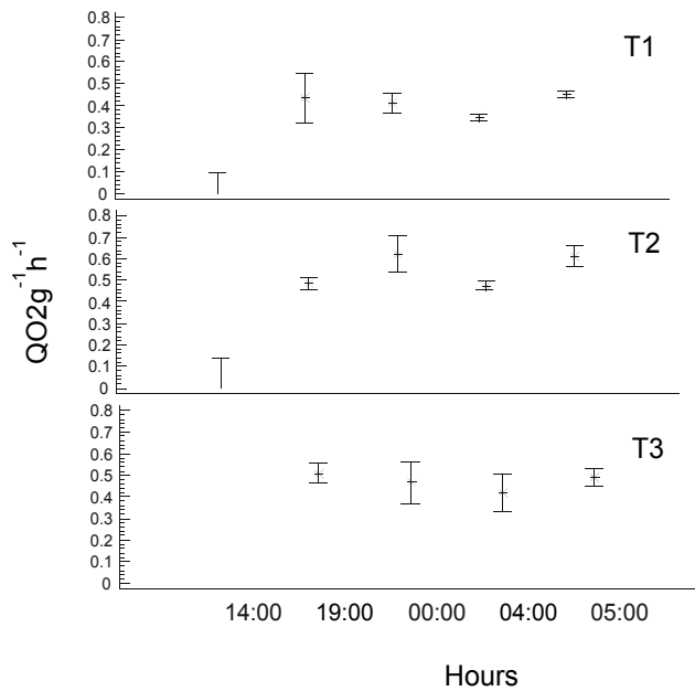
Figure 10. Oxygen consumption for each diet treatment at the end of the experiment
