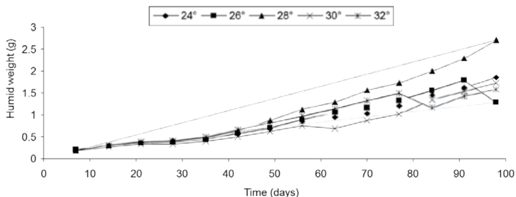
Figure 5. Humid weight behavior for the different temperature treatments
