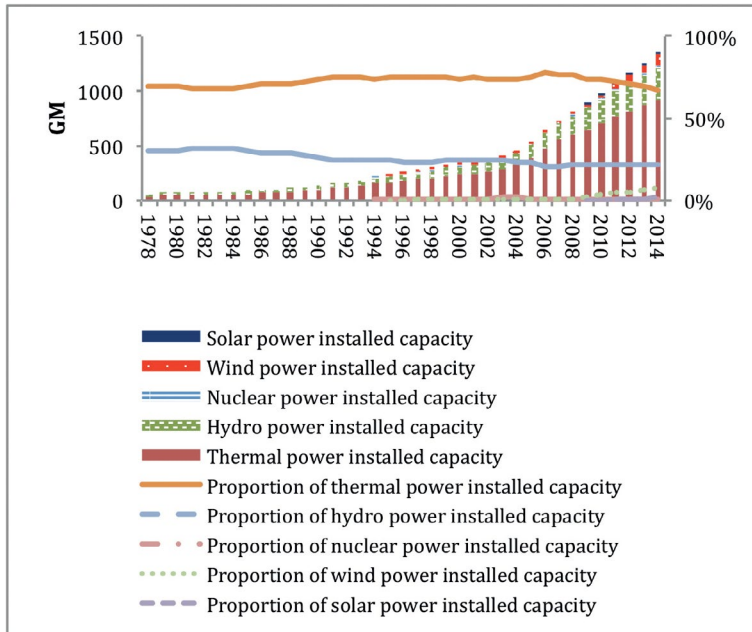
Figure 19.1 Power installed capacity mix in China
