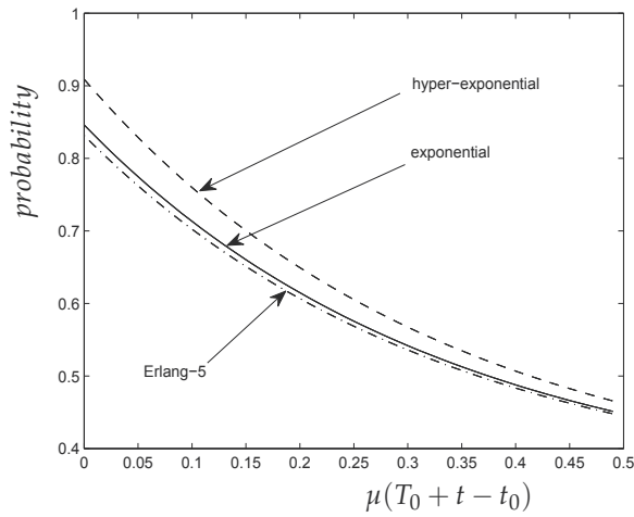
Fig. 3. Existence probability with \gamma = 1.0 and \Delta = 2.0
