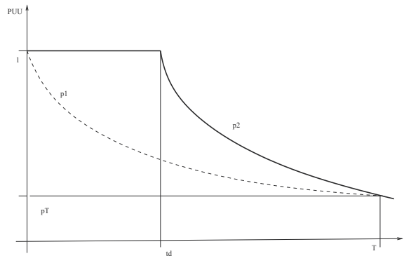
Fig. 7. A more realistic transition function P_{UU} in the time.
