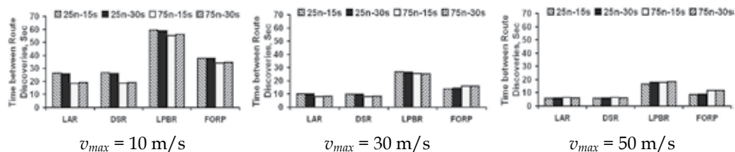
Fig. 9. Average Time between Successive Route Discoveries per Source-Destination Session
