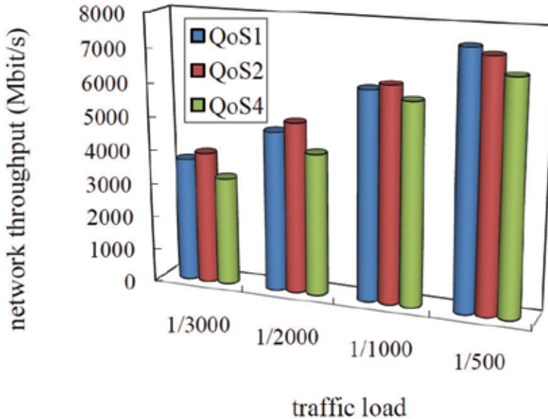
Fig. 7. Network throughput vs. traffic load (= QoS requirement times call arrival rate), where number of hosts=30, number of time slots=16, pose time=0, and mobility=4m/s.
