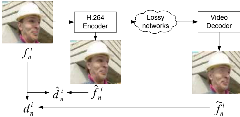
Fig. 6. Video Coding and Transmission System
