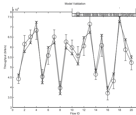
(d) NAMA with Node-Disjoint Routing Per-flow Throughput (50 Nodes Network, 20 flows)
