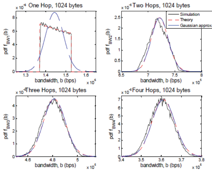
Fig. 3. Comparison of Equations 15 and 20 with QualNet® simulations and the proposed Gaussian approxin
