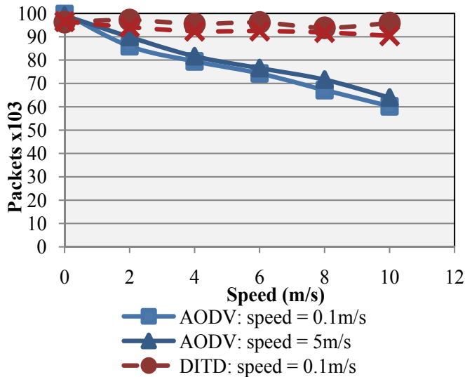
Figure 19: Packet Delivery Ratio for slow moving network under black hole attack
