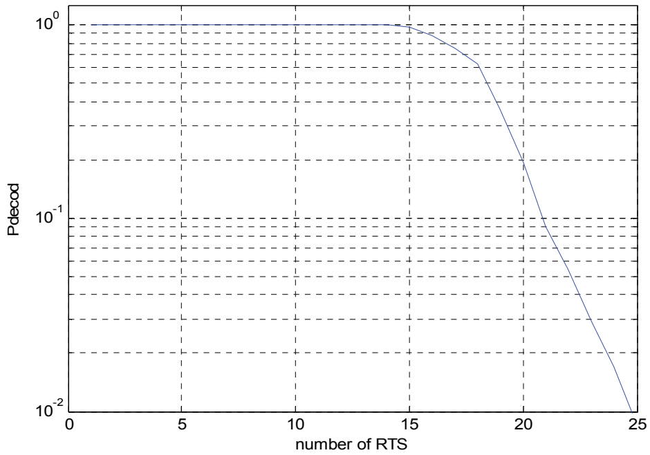
Fig. 7. The probability of correct decoding for 1-24 RTS packets
