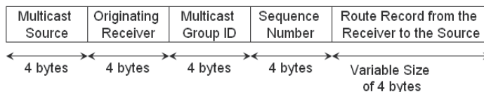
Fig. 16. Structure of Multicast Tree Establishment Message
