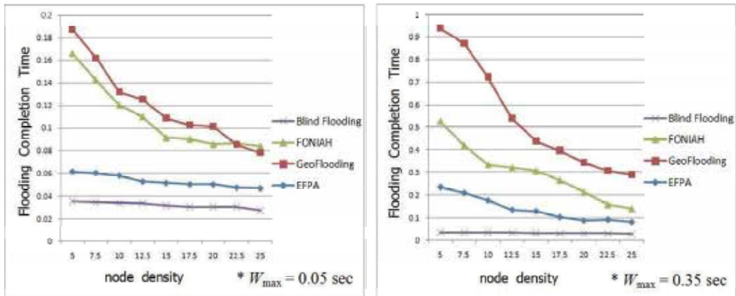
Fig. 10. Average delay with varying the maximum waiting time as 0.05sec and 0.35sec [taken from (Jaegal & Lee, 2008)]
