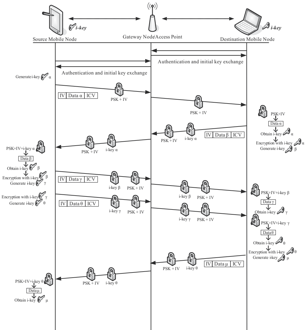
Fig. 3. Dynamic i-key encryption and decryption protocol procedures
