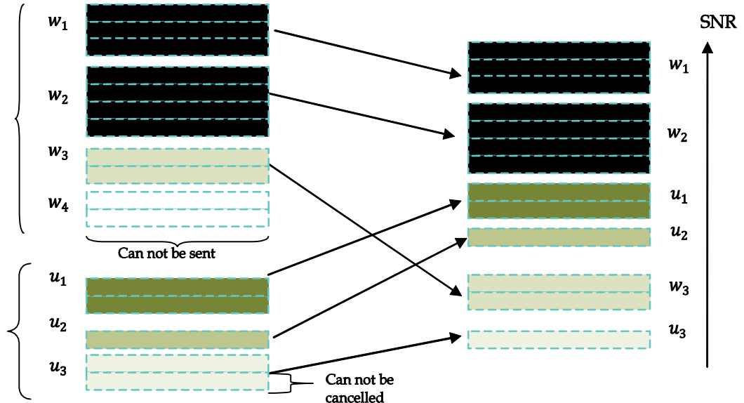
Fig. 19. An example of application of SNR based receiver protocol.
