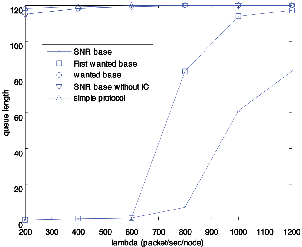
Fig. 27. Queue length versus network traffic.
