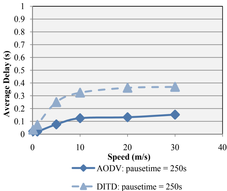
Fig. 17. Average end-to-end delay for partially stable network (250 second pause time)
