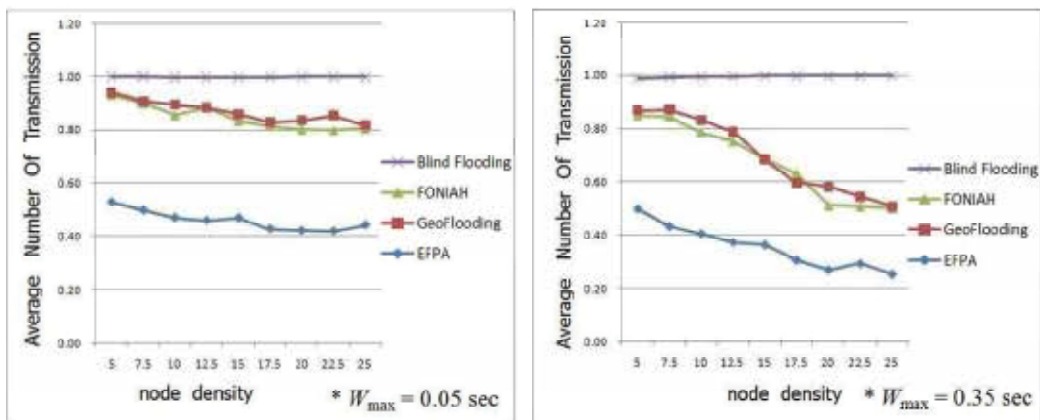
Fig. 9. Average number of transmissions with varying the maximum waiting time as 0.05sec and 0.35sec [taken from (Jaegal & Lee, 2008)]
