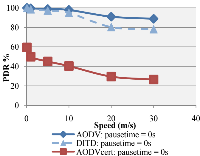
Fig. 12. Packet Delivery Ratio for highly mobile network (0 second pause time)
