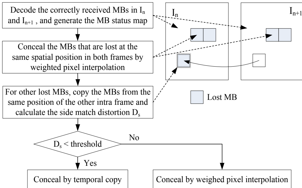
Fig. 3. Error concealment in intra frame for MSVC
