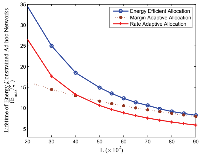
Fig. 8. Performance comparison among different allocation schemes
