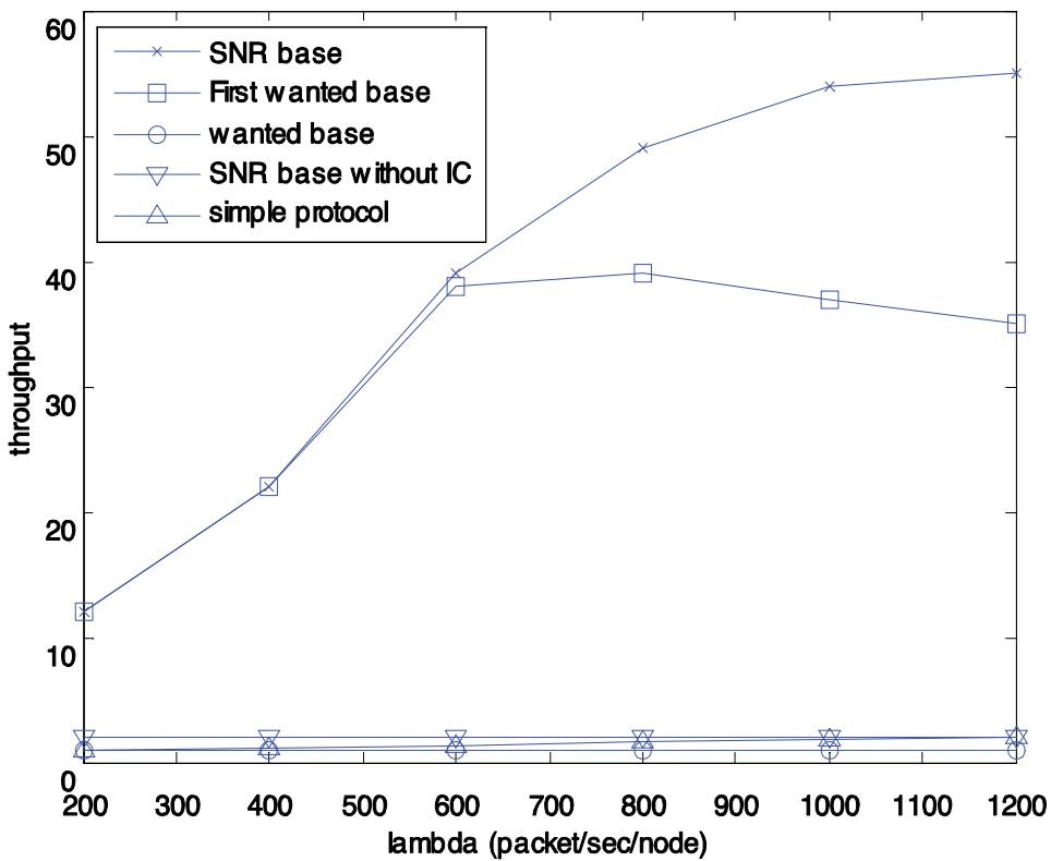
Fig. 26. Network throughput versus network traffic.
