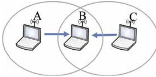
Fig. 1. Hidden terminal problem.
