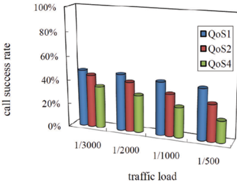
Fig. 8. Call success rate vs. traffic load, where number of hosts=30, number of time slots=16, pose time=0, and mobility=4m/s.
