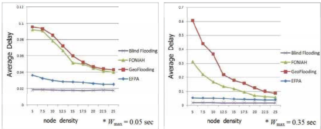
Fig. 11. Flooding completion time with varying the maximum waiting time as 0.05sec and 0.35sec [taken from (Jaegal & Lee, 2008)]
