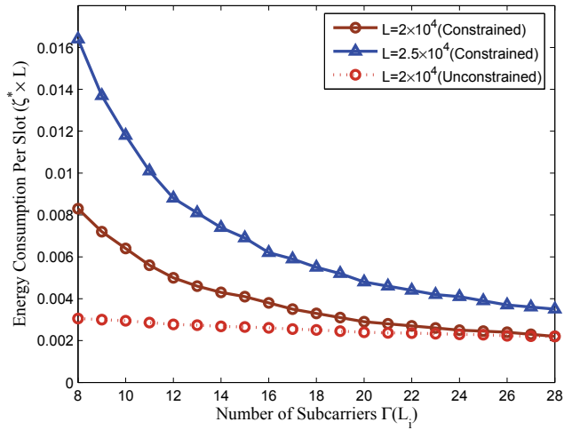
Fig. 7. Impact of number of available subcarriers to energy efficiency
