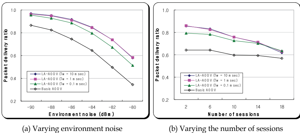
Fig. 5. Packet delivery ratio.
