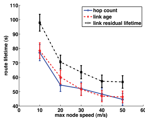
Fig. 1. Average route lifetime with ideal wireless transmissions: radio coverage only limited by the distance between nodes.
