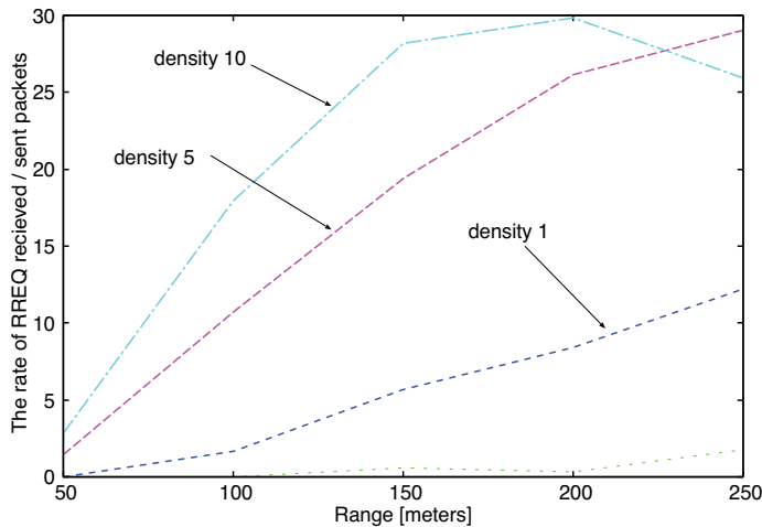
Fig. 17. The average number of RREQ adjacent nodes.
