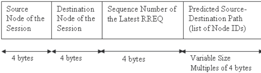
Fig. 6. Structure of the LPBR-RREP Packet
