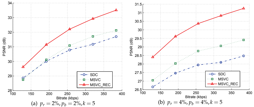
Fig. 8. Average PSNR vs Bitrate for SDC, MSVC, and MSVC_REC, Foreman sequence at 30 fps
