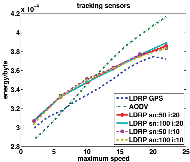
Fig. 8. The power consumption-throughput ratio (Joule/byte) gives an indication of the energetic cost of the network (lower is better).
