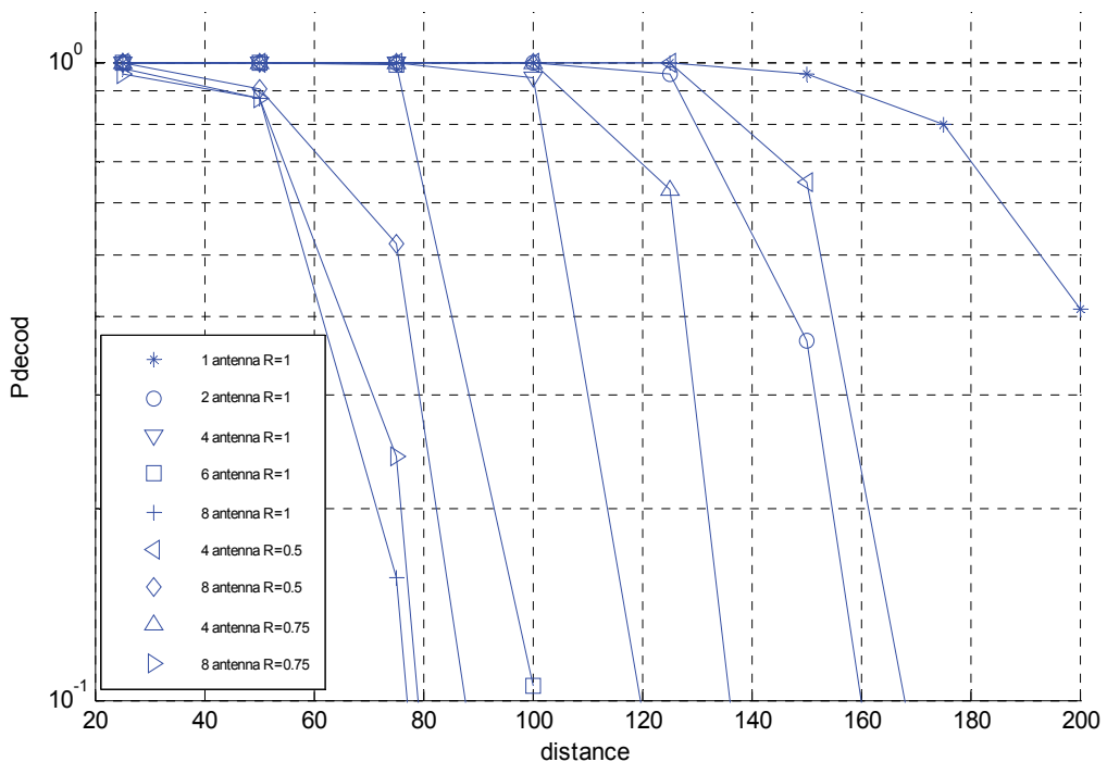
Fig. 12. Probability of correct packet reception for two users data transmission as a function of distance, with and without coding
