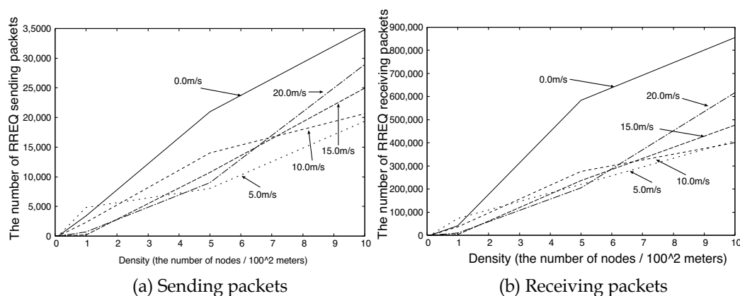
Fig. 5. The number of RREQ varying the node speed.
