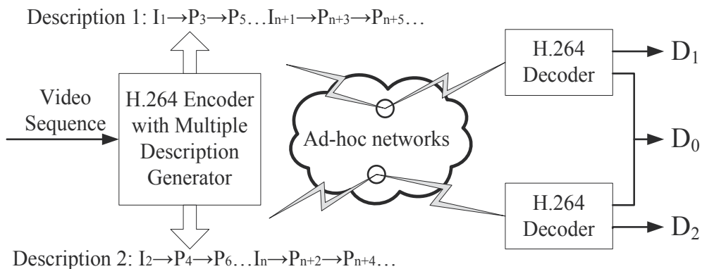
Fig. 1. MSVC system architecture
