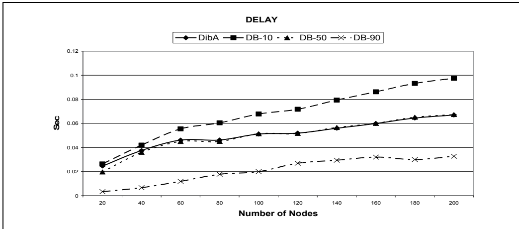
Fig. 12. Delay - Normal - BGR 5p/s
