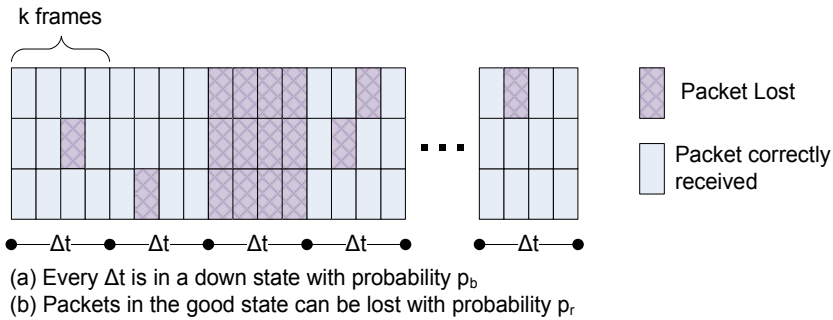
Fig. 7. Packet Loss Model
