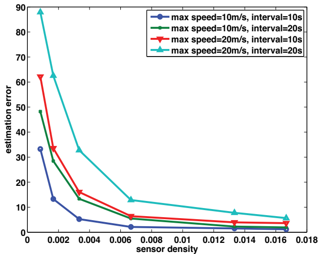
Fig. 4. Localization error of the estimates with respect to the real node location.
