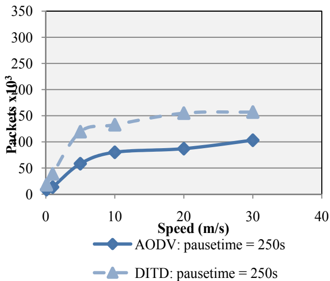
Fig.15. Control packet overhead for partially stable network (250 second pause time)
