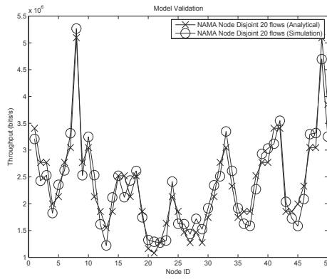
(b) NAMA with Node-Disjoint Routing Per-Node Throughput (50 Nodes Network, 20 flows)
