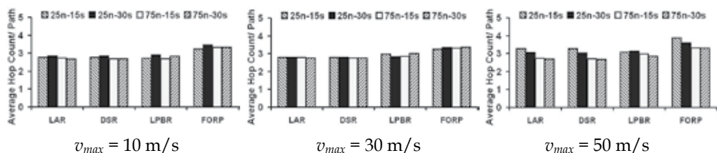
Fig. 10. Average Hop Count per Source-Destination ( s-d ) Path
