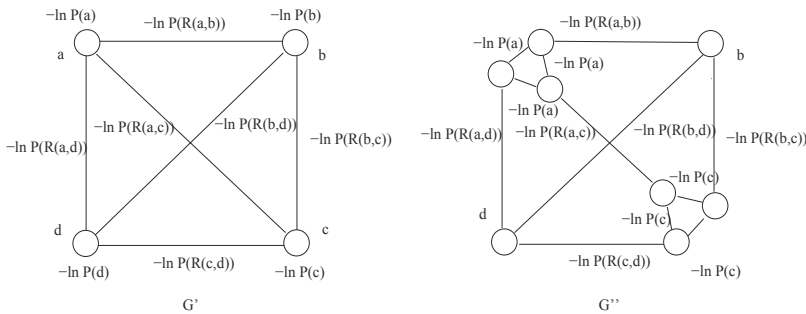
Fig. 2. The valuation of the topology graph
