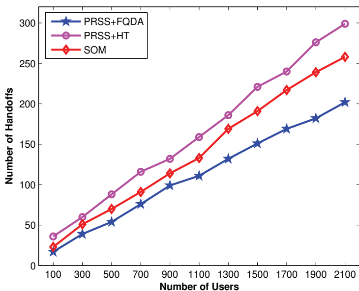
Fig. 8. Number of handoffs versus numbers of users (Arrival rate = 3 sec)
