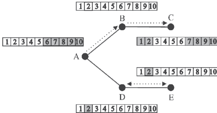
Fig. 3. Example of how bandwidth calculation is interfered by the hidden- and exposed-terminal problem.
