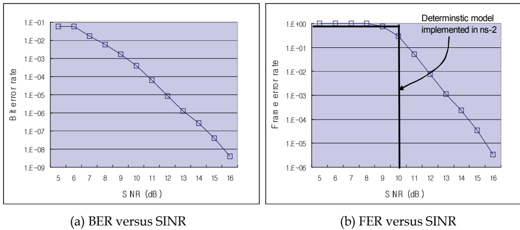
Fig. 4. BER and FER for QPSK with 2 Mbps in the Intersil HFA3861B radio chip. (The PHY frame size for calculating FER is assumed to be 864 bits, i.e. , 144-bit preamble, 48-bit PLCP header and 84-byte payload.)
