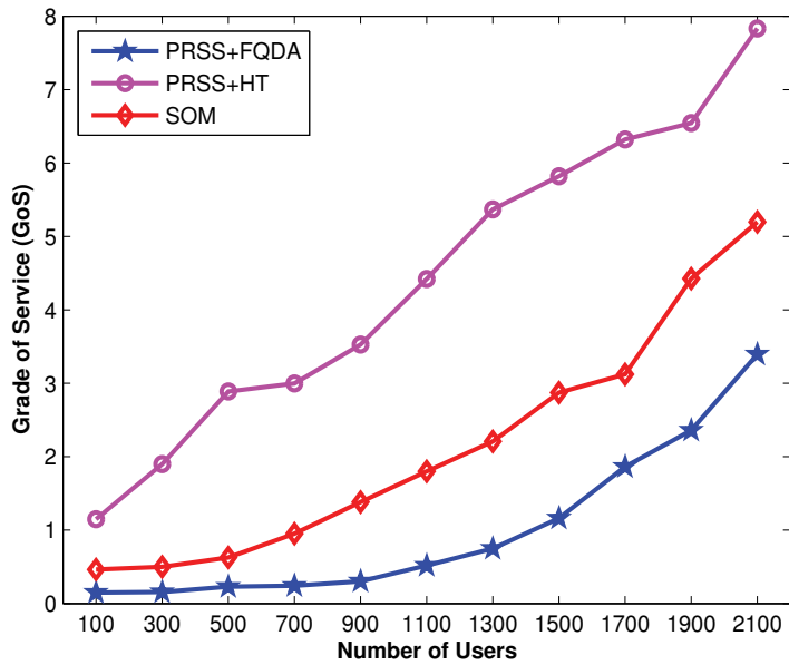
Fig. 10. GoS versus numbers of users (Arrival rate = 3 sec)
