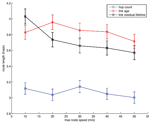
Fig. 2. Average route length (hops) with ideal wireless transmissions.
