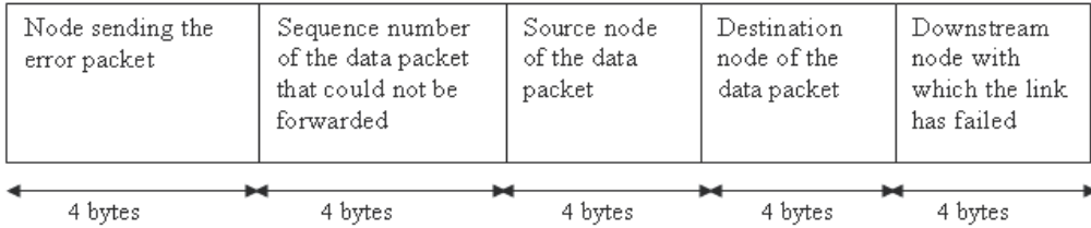
Fig. 5. Structure of the Route-Error Packet
