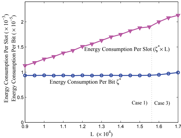
Fig. 6. Impact of L to energy efficiency
