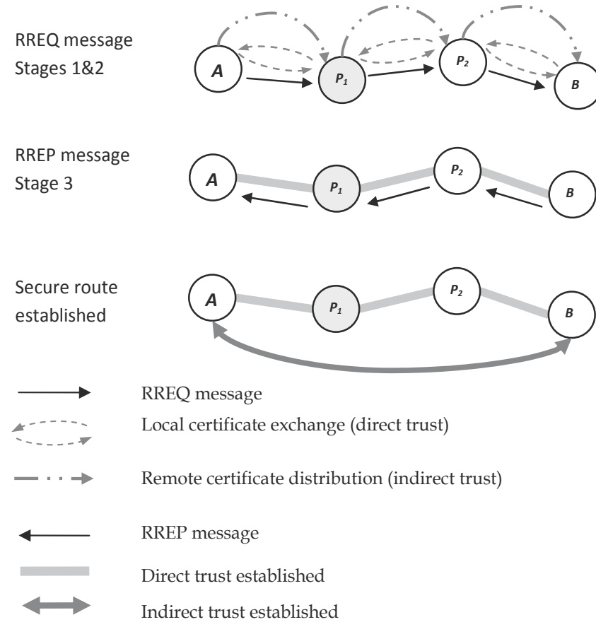
Fig. 5. Illustrating the certificate exchange protocol
