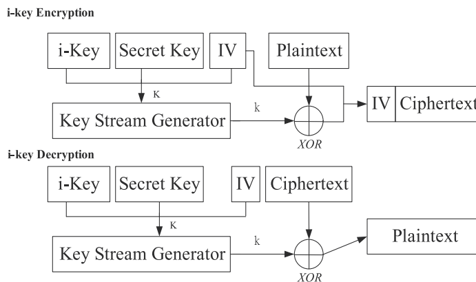
Fig. 2. Block diagram of i-key secure protocol
