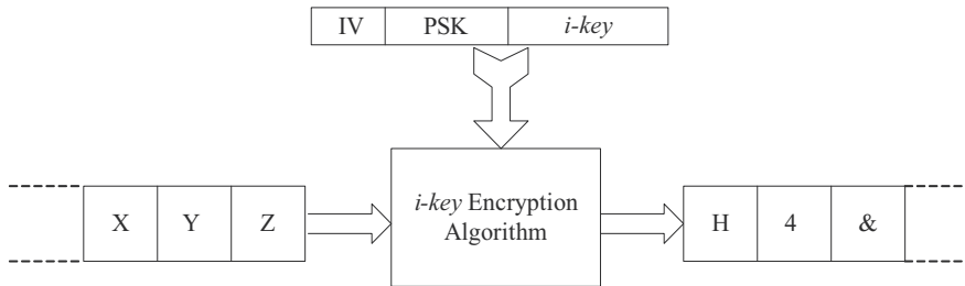
Fig. 4. Dynamic i-key encryption stream cipher
