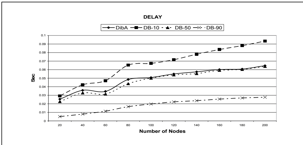
Fig. 15. Delay - Diverse - BGR 5p/s
