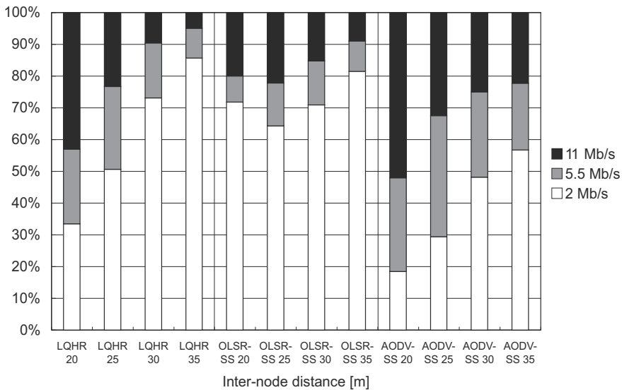
Fig. 10. The percentage of selected transmission speed for audio-video stream.
