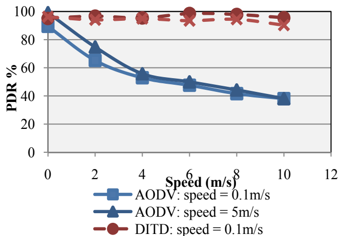
Fig. 21. Packet Delivery Ratio for slow moving network under black hole rush attack
