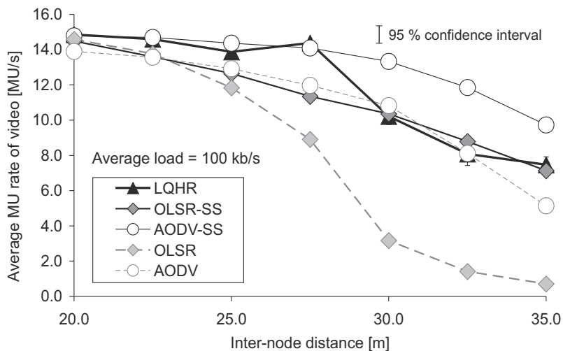
Fig. 6. Average MU rate of video.
