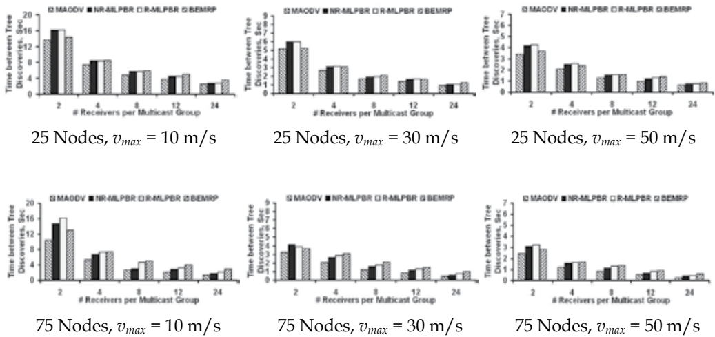
Fig. 22. Average Time between Successive Broadcast Tree Discoveries
