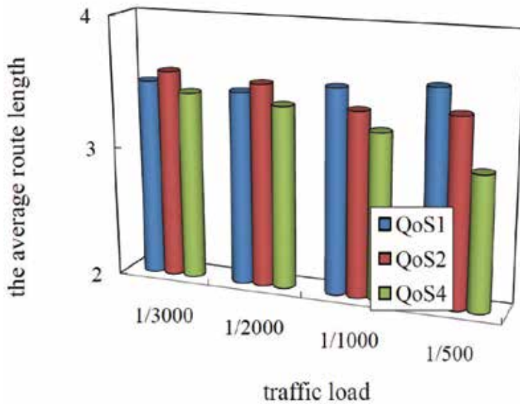
Fig. 9. The average route length v.s. traffic load, where number of hosts=30, number of time slots=16, pose time=0, and mobility=4m/s.
