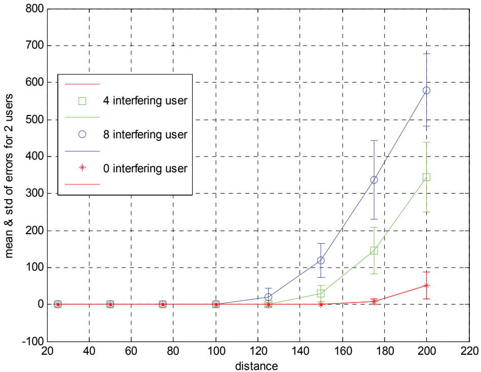
Fig. 9. Average and standard deviation of bit errors over two packets as a function of distance
