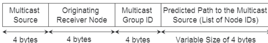
Fig. 19. Structure of the Multicast Predicted Path Message (MPPM)
