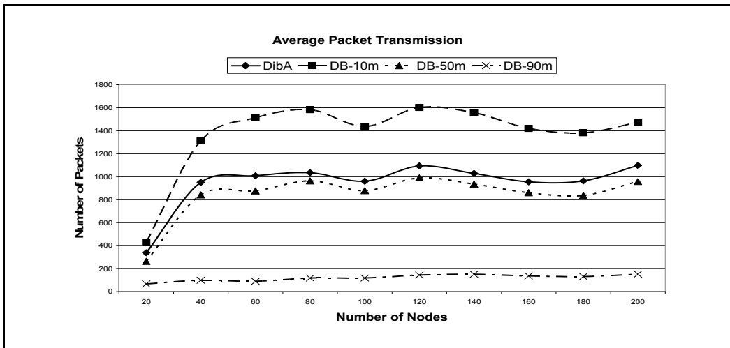
Fig. 19. APT - Normal - BGR 60p/s
