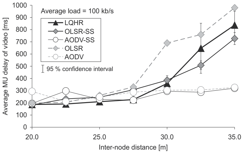
Fig. 7. Average MU delay of video.
