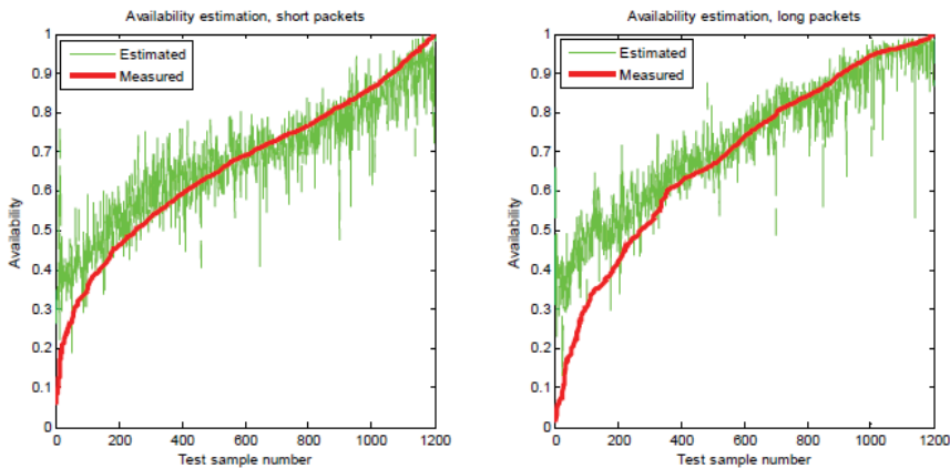
Fig. 17. Availability estimation on the test trace (data not seen by the system during training).
