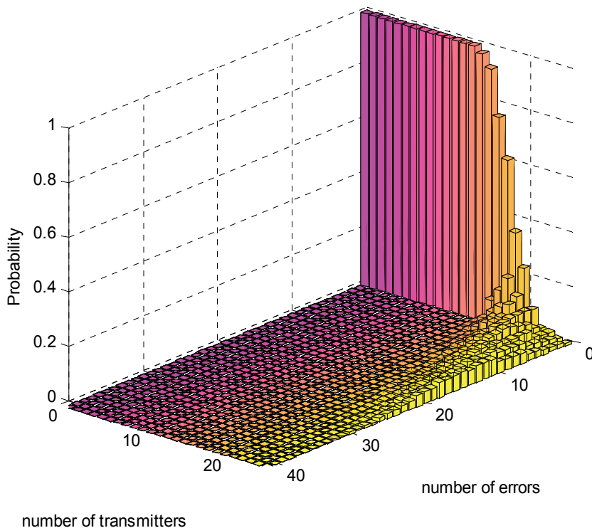
Fig. 5. Probability of errors in the RTS packets sent from 1 to 24 transmitters
