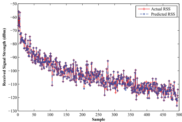
Fig. 3. Prediction results by using back-propagation neural network
