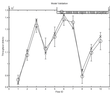
(c) NAMA with Node-Disjoint Routing Per-flow Throughput(50 Nodes Network, 10 flows)
