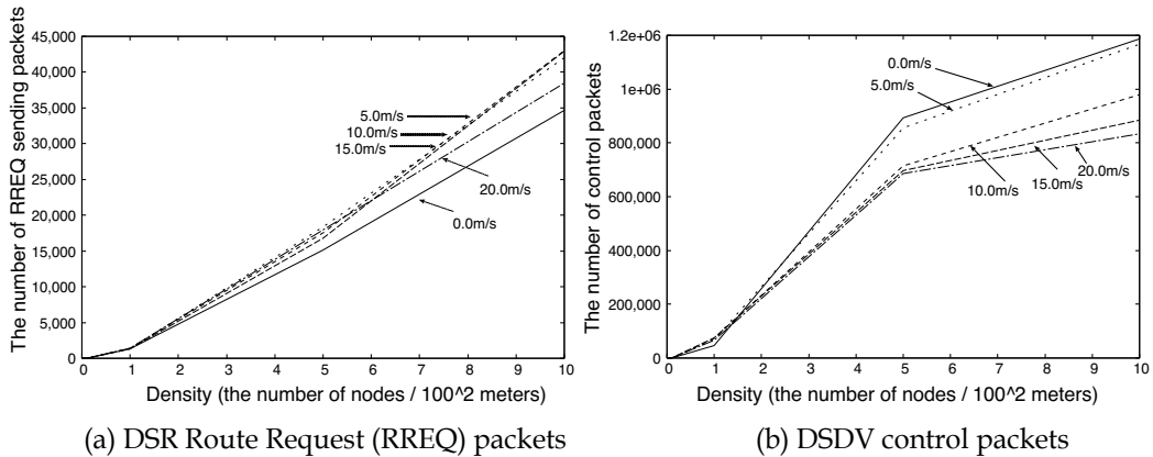
Fig. 7. The number of control packets varying the node speed.
