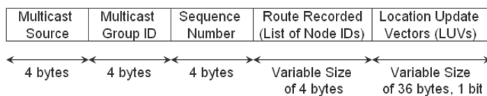
Fig. 15. Structure of the Multicast Tree Request Message
