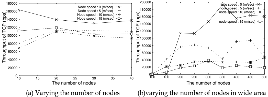
Fig. 3. The throughput of TCP.
