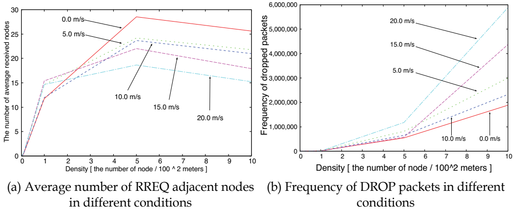
Fig. 8. Degradation features of RREQ.
