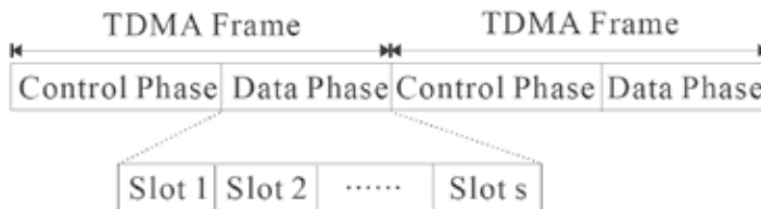
Fig. 1. The TDMA frame structure.
