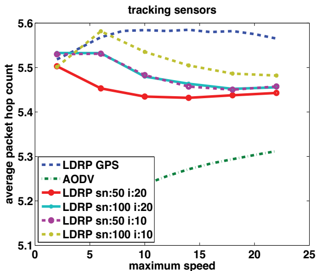
Fig. 6. Average path length in number of hops.
