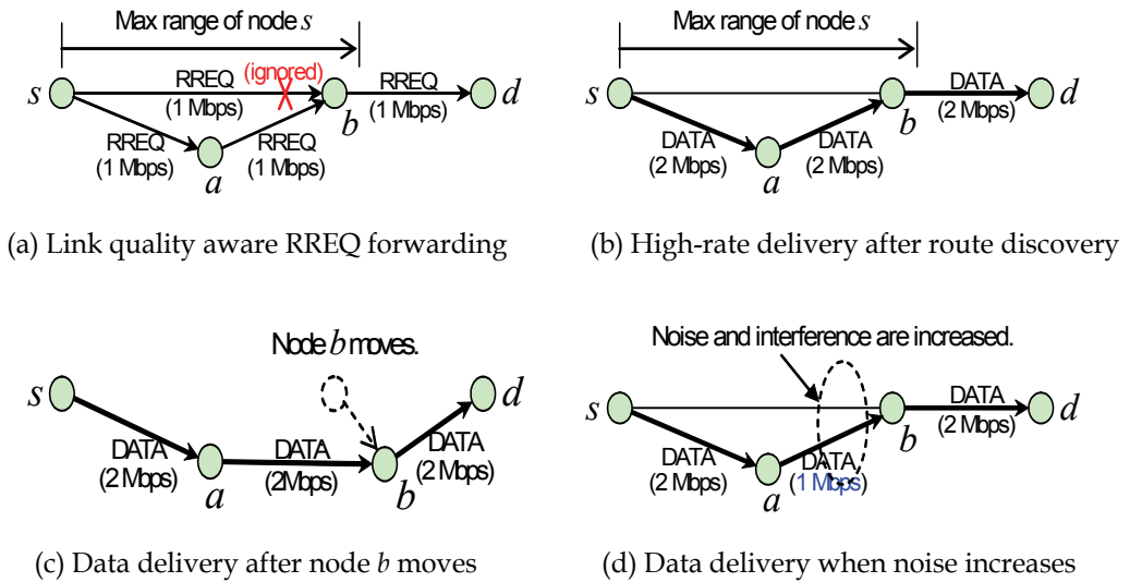
Fig. 3. Link quality aware RREQ forwarding and its resulting effects for the same example as in Fig. 1.
