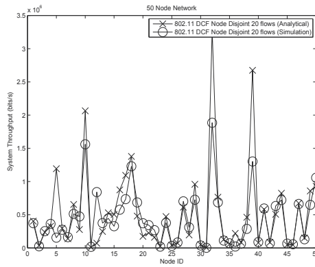
(a) 802.11 DCF with Node-Disjoint Routing Per-node Throughput (50 Nodes Network)
