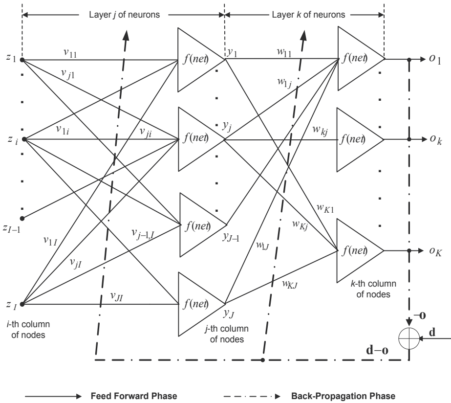
Fig. 2. Two-neuron layer network
