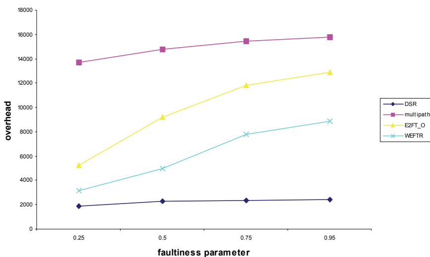
Fig. 5. Plot of the Overhead versus the Faultiness parameter for the various algorithms tested.
