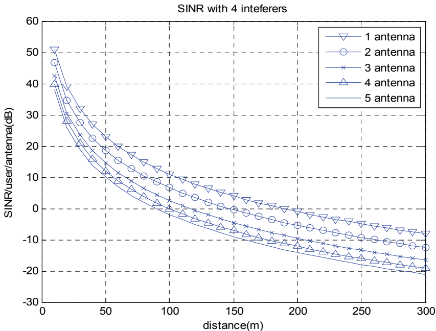
Fig. 4. SINR per user for receiving antenna by varying the distance
