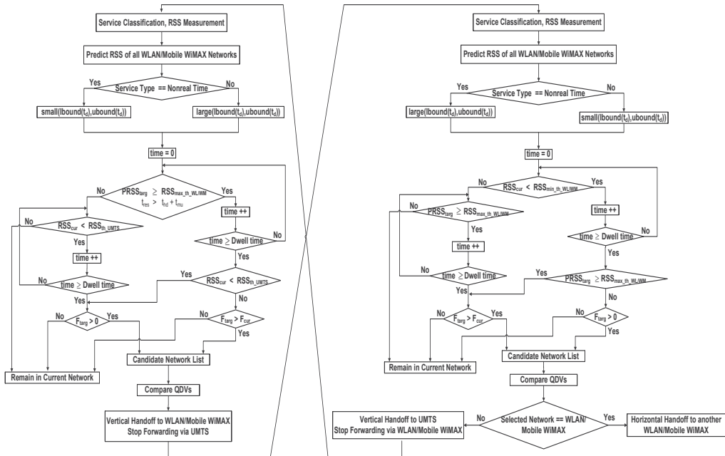
Fig. 5. Handoff decision algorithm when a mobile node is in UMTS or in WLAN/WiMAX
