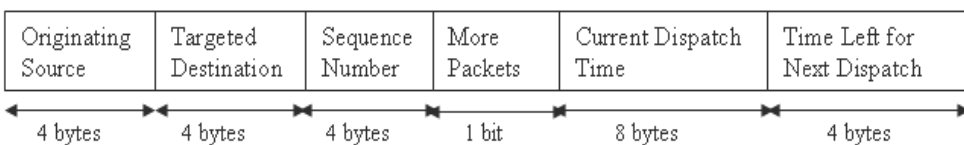
Fig. 4. Structure of the Header of the Data Packet
