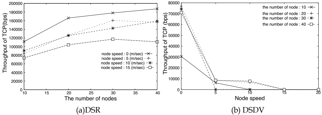
Fig. 4. The throughput varying the number of nodes.
