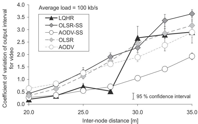
Fig. 5. Coefficient of variation of output interval for video.
