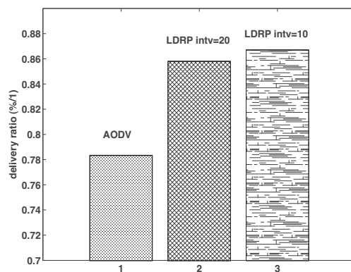
Fig. 12. Delivery ratio of the test flow on the obstructed scenario with nodes moving with speeds from 1 to 20 m/s.
