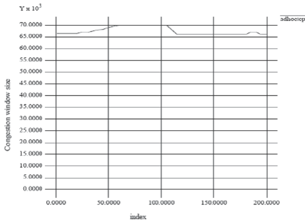
Fig. 5. ADHOCTCP congestion window in presence of bit error only
