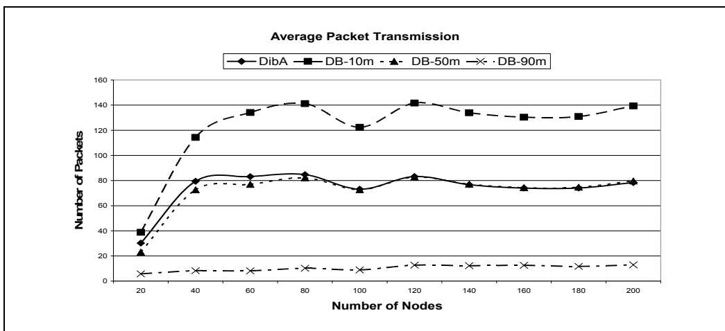
Fig. 13. APT - Normal - BGR 5p/s
