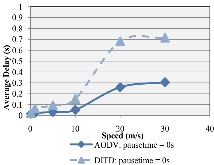
Fig. 16. Average end-to-end delay for highly mobile network (0 second pause time)
