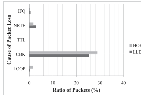
Fig. 12. Packet Loss Specification (12 Flows)
