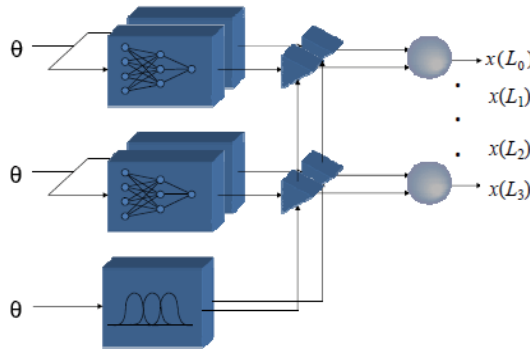
Fig. 16. Structure of the neuro-fuzzy estimator.
