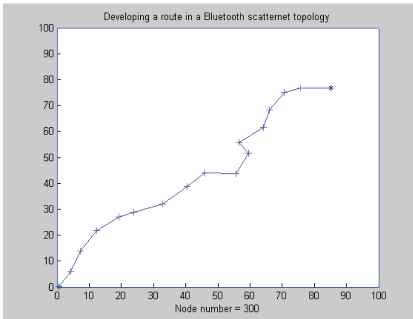
Fig. 4. Screenshot for a route creation connecting a sender and a receiver in a scatternet
