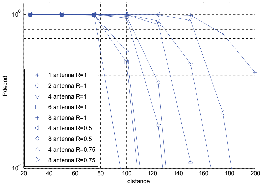
Fig. 11. Probability of correct packet reception for a single data transmission as a function of distance, with and without coding
