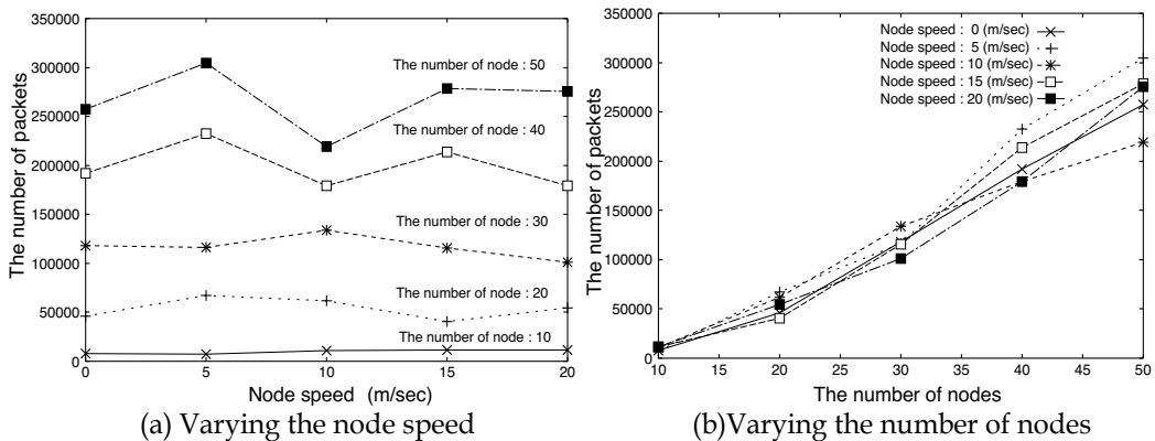
Fig. 1. The number of Route Request (RREQ) packets.
