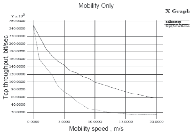
Fig. 6. ADHOCTCP performance in the presence of node mobility
