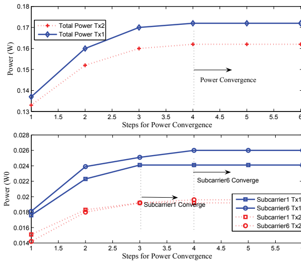
Fig. 9. Convergence of distributed power control
