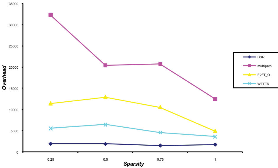
Fig. 3. Plot of the Overhead versus the Sparsity for the various algorithms tested.
