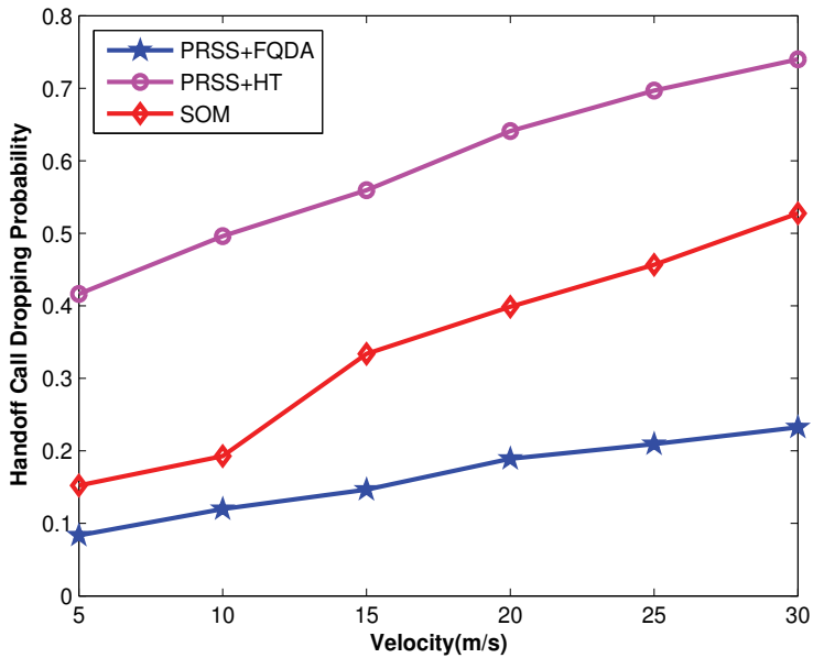
Fig. 15. Handoff call dropping probability versus mobile velocity (Number of users = 1,500 and Arrival rate = 3sec)
