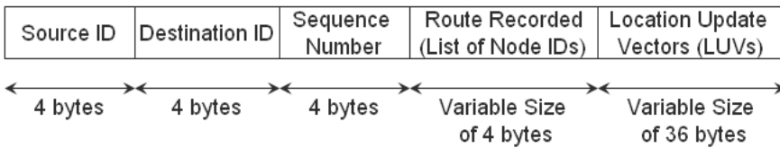
Fig. 23. Multi-path Route Request (MP-RREQ) Message
