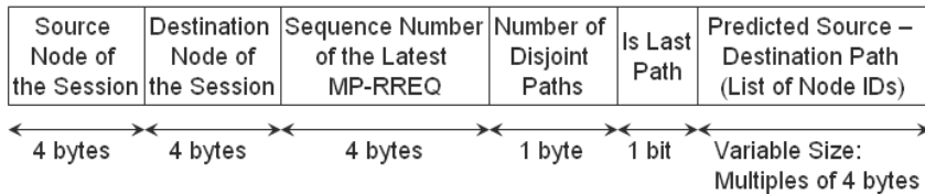
Fig. 27. Structure of the MP-LPBR-RREP Message
