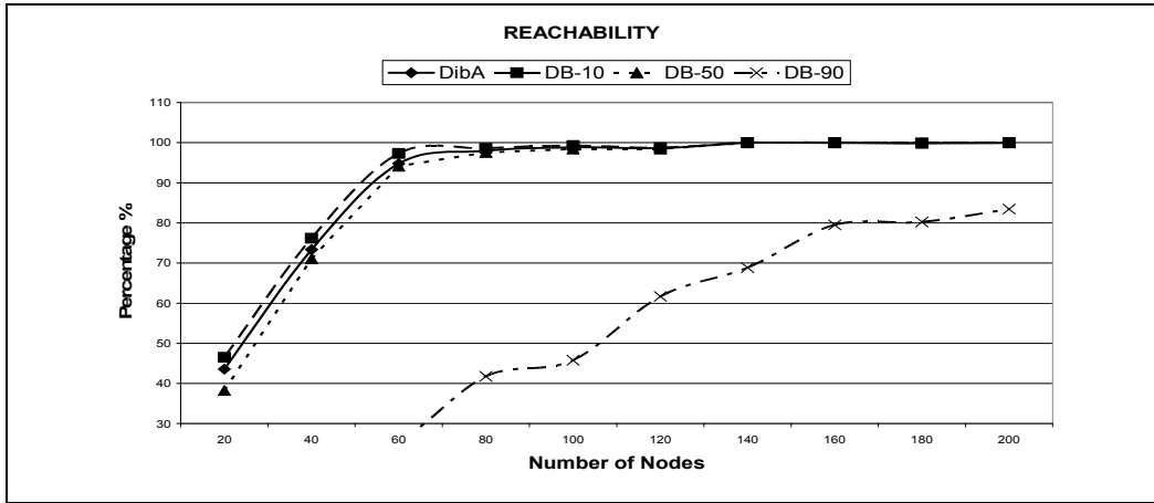
Fig. 11. Reachability - Normal - BGR 5p/s
