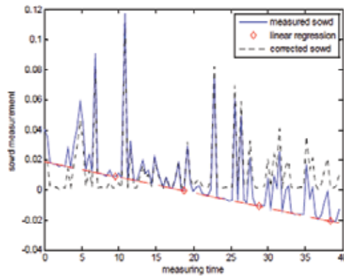
Fig. 10. Correction of clock incoherence through linear regression. Both axes are in seconds.
