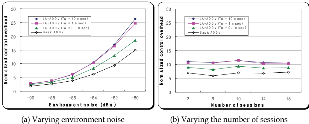
Fig. 7. Normalized control overhead.
