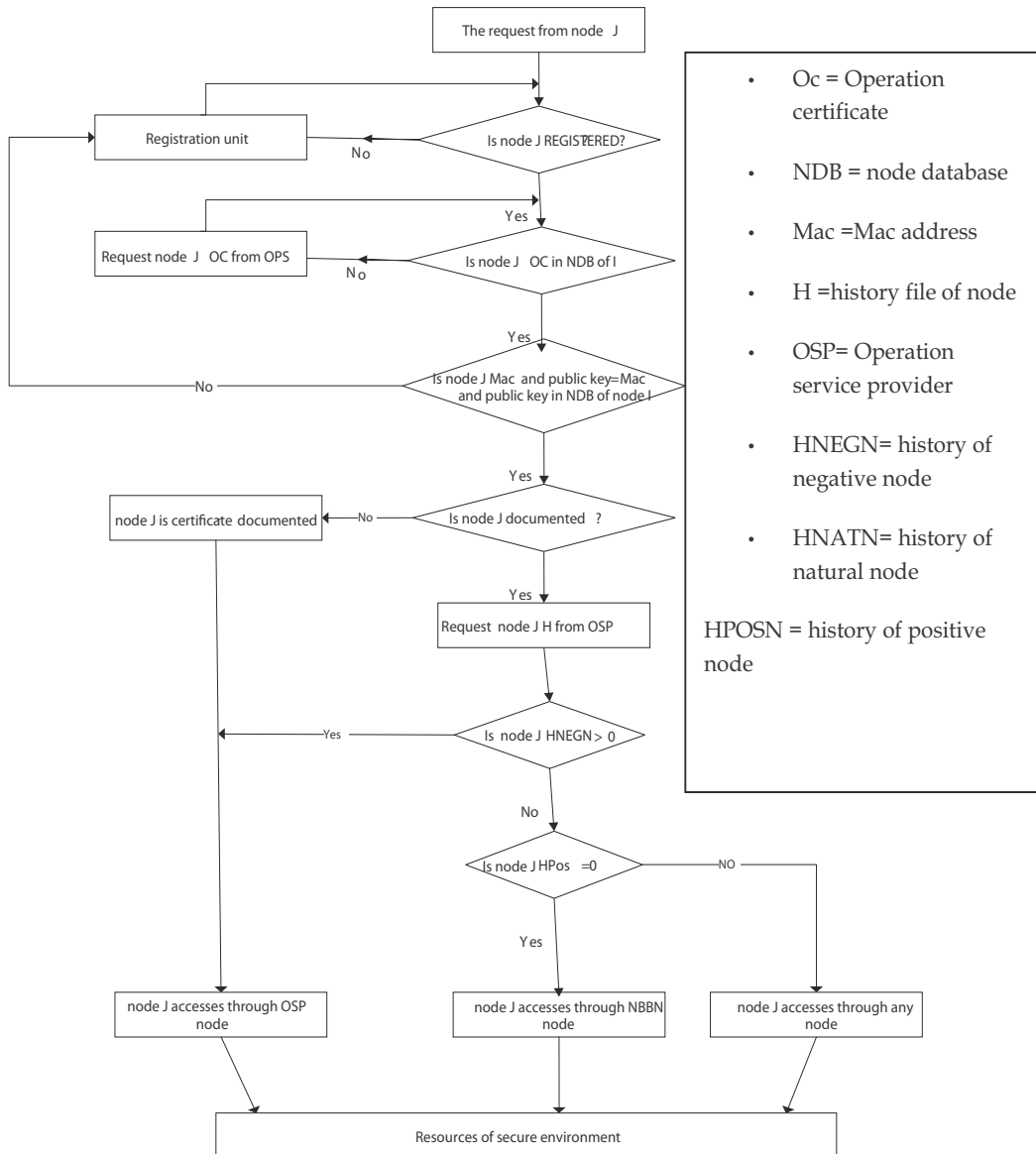
Fig. 3. Activity diagram
