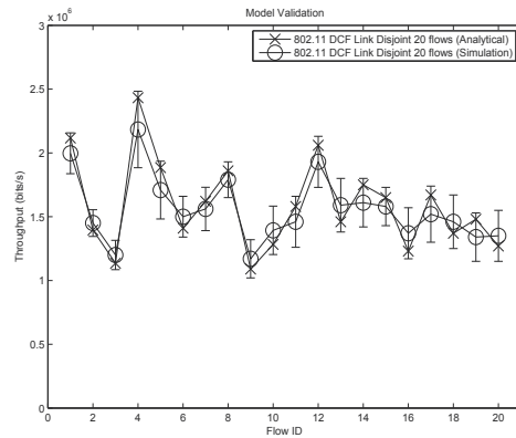
(c) 802.11 DCF with Node-Disjoint Routing Per-flow Throughput (50 Nodes Network, 20 Flows)
