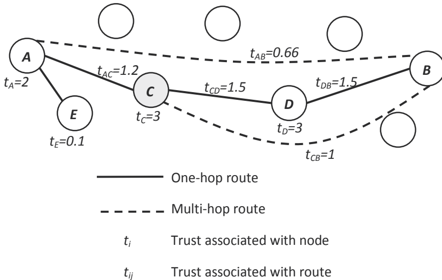
Fig. 7. Weighted Direct Trust Graph
