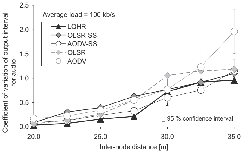
Fig. 4. Coefficient of variation of output interval for audio.
