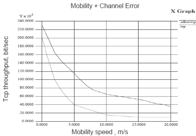
Fig. 7. ADHOCTCP performance in presence of node mobility and channel error
