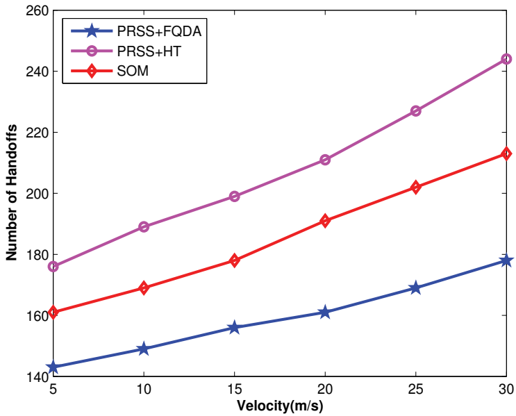
Fig. 14. Number of handoffs versus mobile velocity (Number of users = 1,500 and Arrival rate = 3sec)
