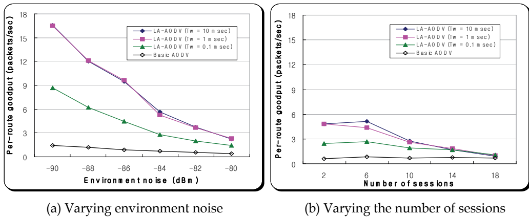
Fig. 6. Per-route goodput.
