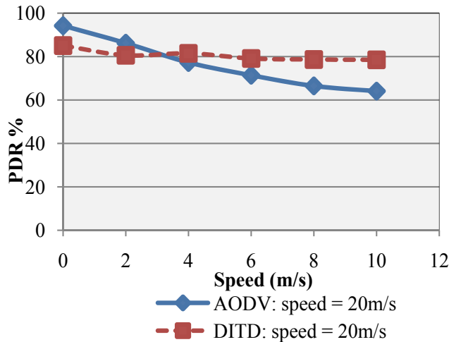
Fig. 20. Packet Delivery Ratio for fast moving network under black hole attack
