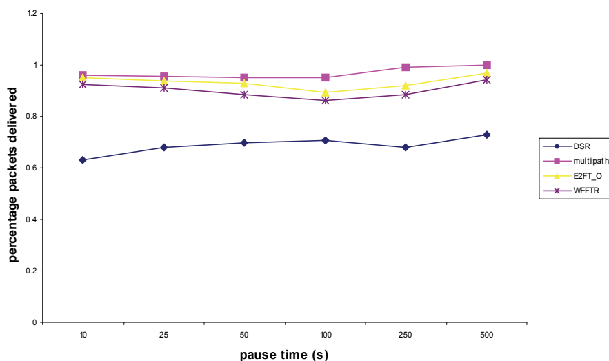
Fig. 2. Plot of percentage delivered packets versus Pause Time for the various algorithms tested.
