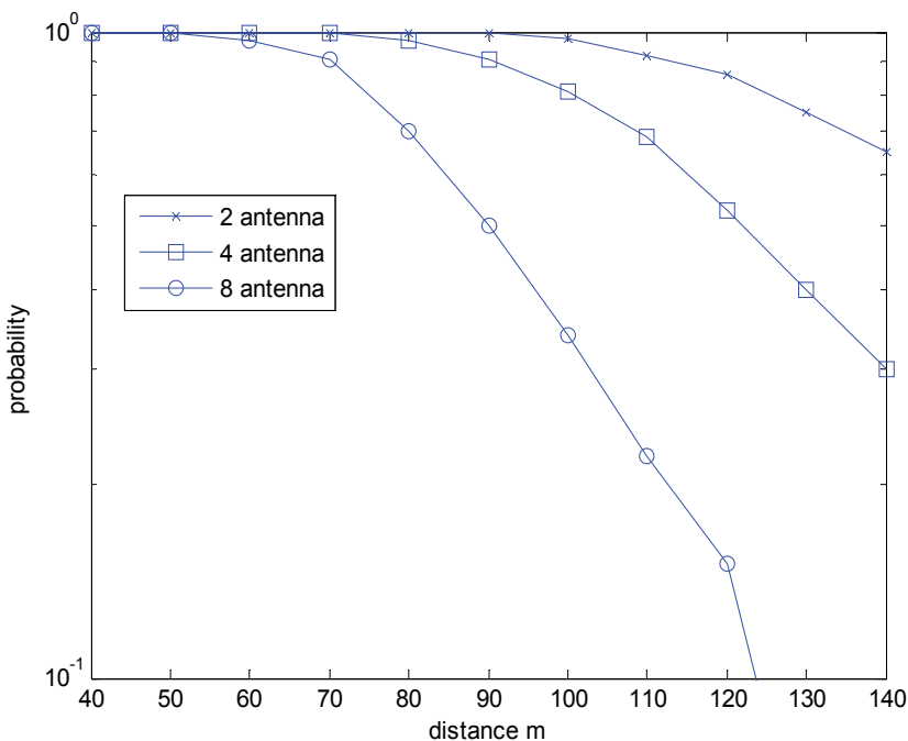
Fig. 14. Probability of correct receiving a data packet by varying the distance and number of transmitter antennas
