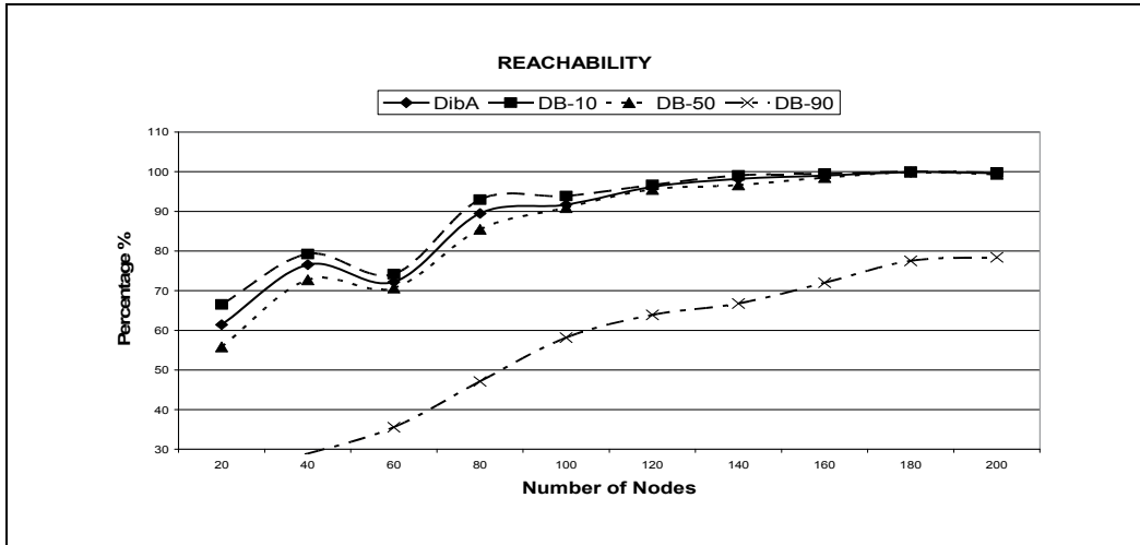
Fig. 14. Reachability - Diverse - BGR 5p/s
