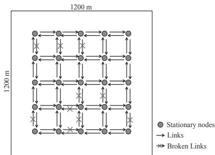
Fig. 8. Link State in 8 Flows Scenario
