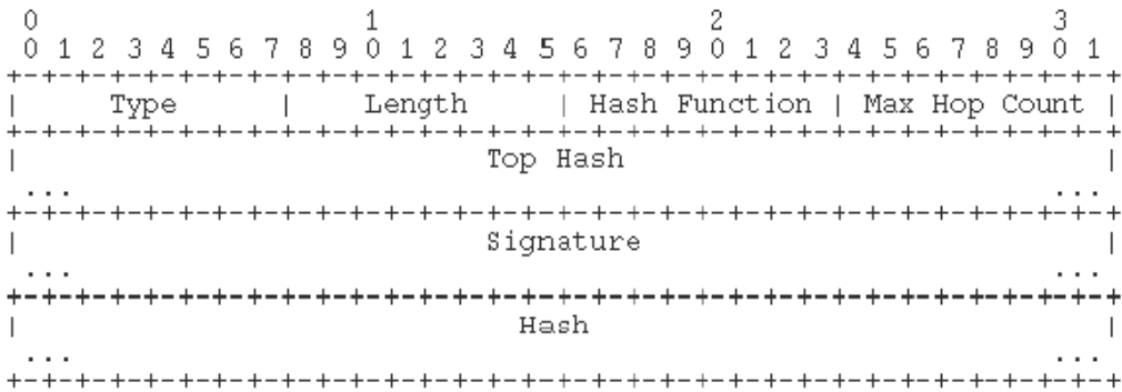
Fig. 1. RREQ Single Signature Extension
