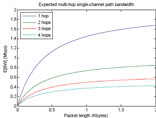
Fig. 4. Expected BW of a multi-hop channel path.
