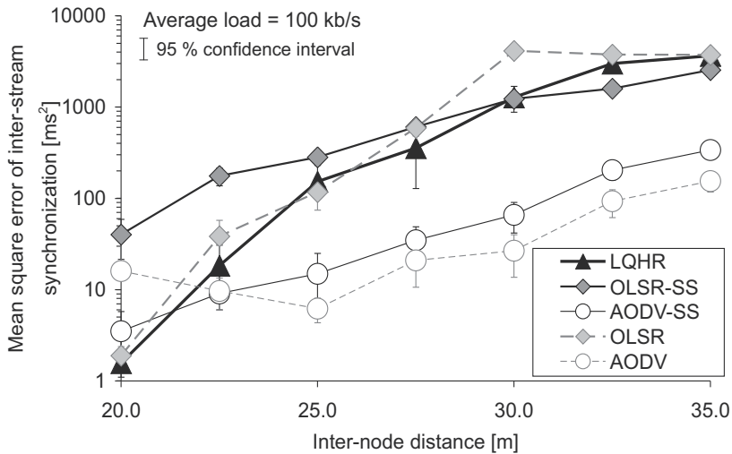
Fig. 8. Mean square error of inter-stream synchronization.
