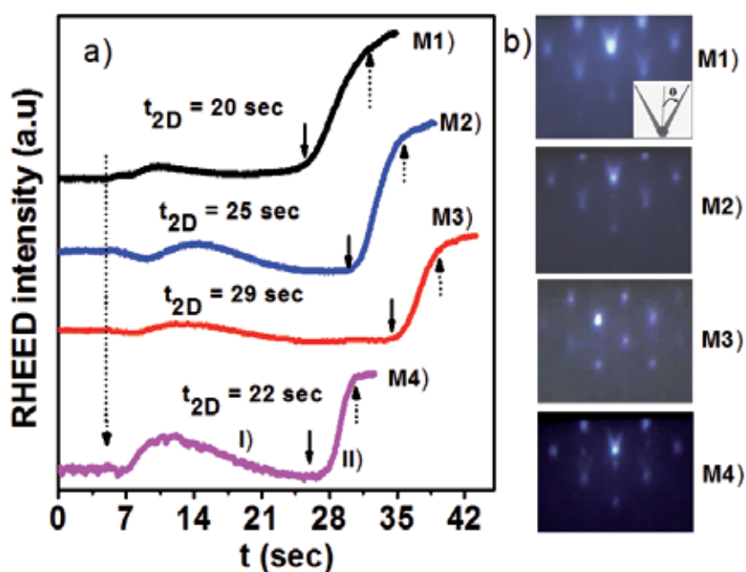
Fig. 1. (a) RHEED intensity of the transmission spot as a function of growth time ( t ) for InAs SAQDs grown at temperatures of: (M1) 480 °C, (M2) 490 °C, (M3) 510 °C, and (M4) 510 °C with Nitrogen. (b) RHEED patterns along the [01-1] after the growth of the InAs SAQDs. A constant Arsenic overpressure of 3 \times 10^{-7} Torr was employed in all the growths.
