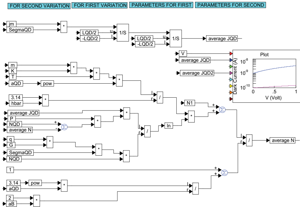
Fig. 3.2. Dark current density block diagram model of QDIPs.
