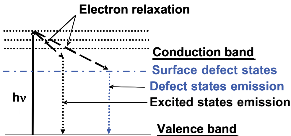
Fig. 1. Schematic diagram illustrating basic emission properties of CdSe quantum dots.
