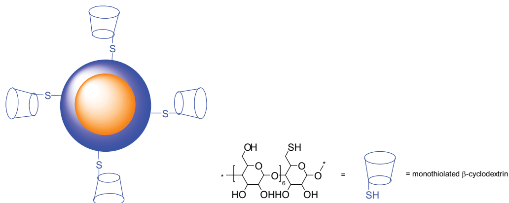
Fig. 16. structure of cyclodextrin-capped CdSe/Cds QDs
