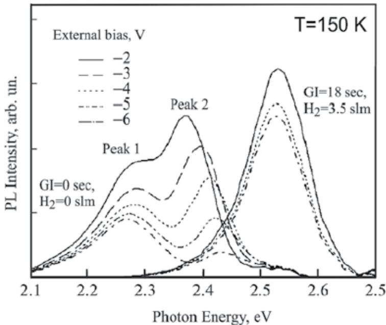
Fig. 6. Photoluminescence spectra of the InGaN/GaN QWs at various values of the reverse bias. (Tsatsulnikov et al., 2011a)
