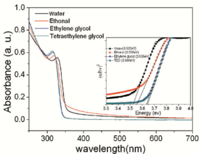
Fig. 4. UV-vis absorbance spectra of ZnO in different solutions. The inset depicts the results of band-gap energy calculation.
