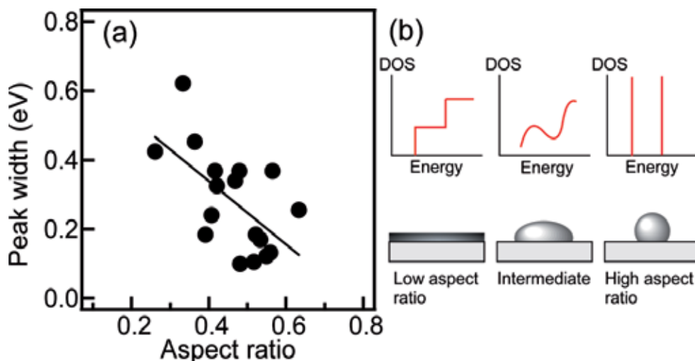
Fig. 11. (a) Dependence of peak width in STS on aspect ratio of QDs. (b) Illustration of density of states depending the QD shape.
