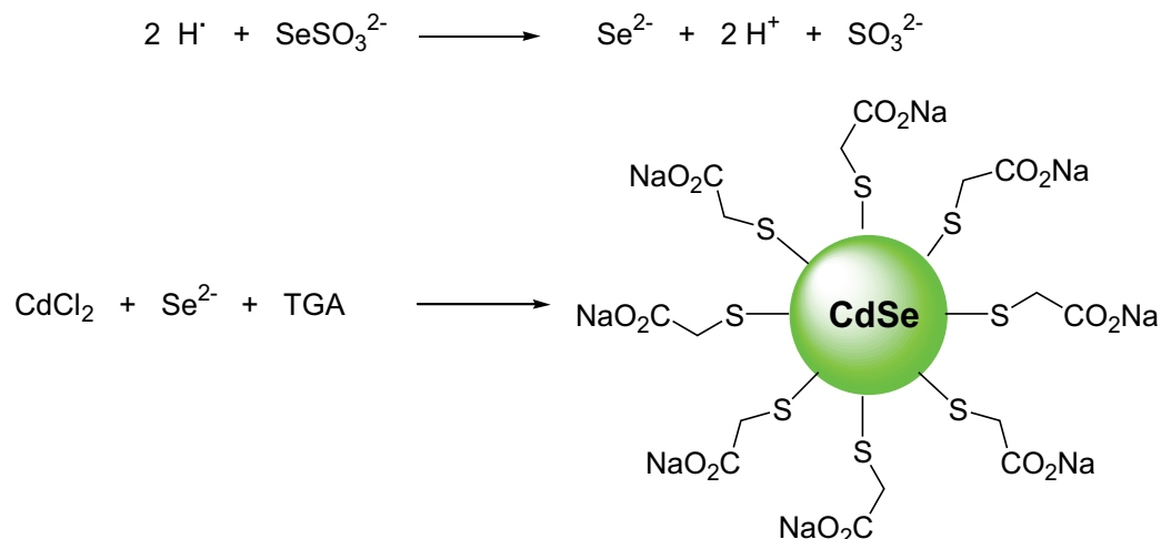
Fig. 17. Synthesis of CdSe@TGA QDs under ultrasonic irradiation
