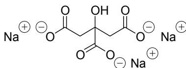
Fig. 10. Chemical structure of trisodium citrate
