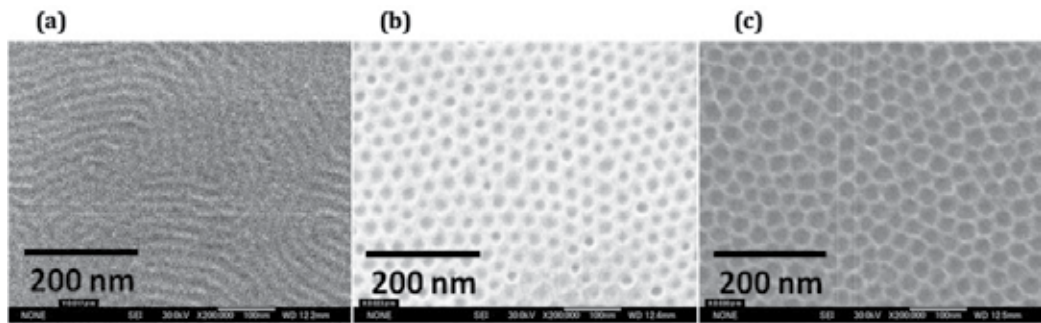
Fig. 5. Fabricated nanodots pattern using 2% solution of PS-PDMS block copolymer which is dropped with different volume onto 1 cm 2 silicon substrates. (a-c) 10, 20, and 40 \mu L, respectively.
