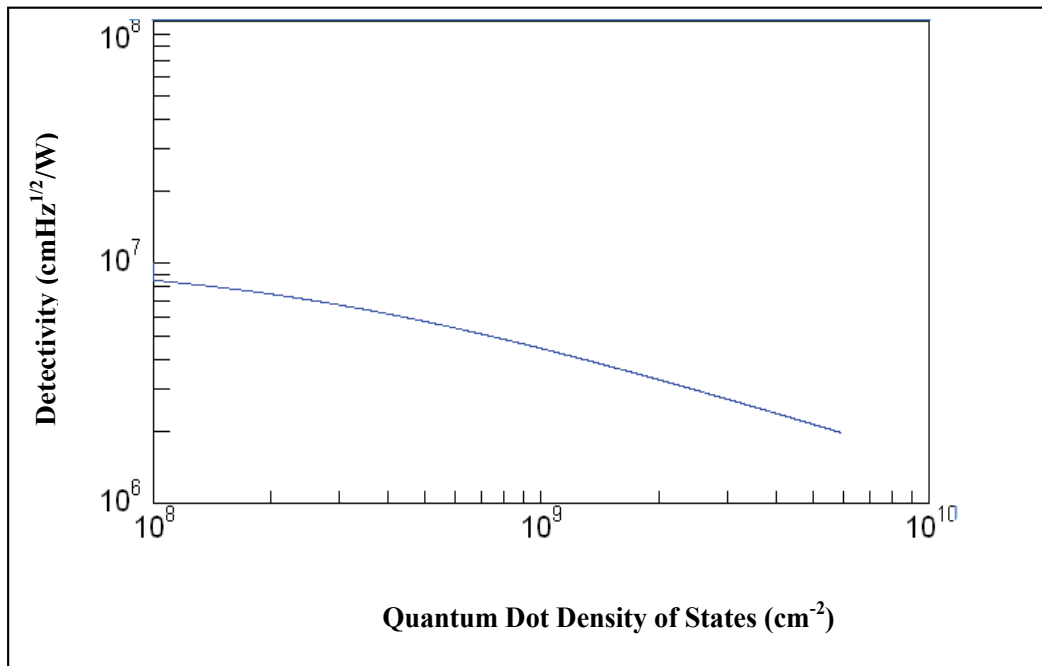
Fig. 3.10. Detectivity against quantum dot density of states.
