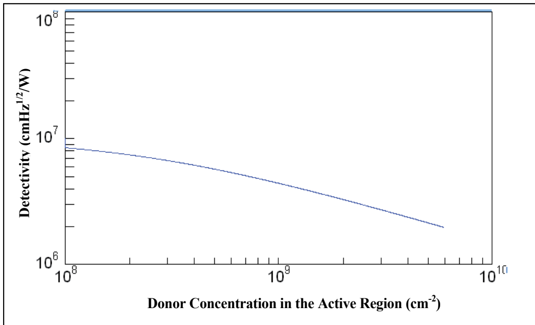
Fig. 3.11. Detectivity against \Sigma_D .
