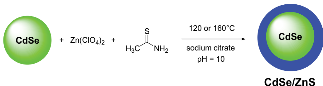
Fig. 13. Preparation of core/shell CdSe/ZnS QDs under microwave irradiation
