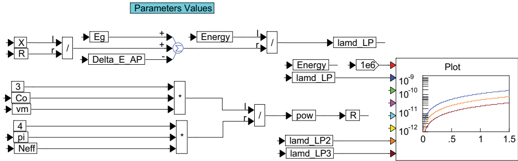
Fig. 3.1. Block diagram model that describes the effect of incident gamma energy on emission wavelength.
