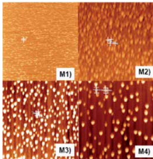
Fig. 3. 1 \times 1 \mu\text{m}^2 AFM images of InAs SAQDs (M1, M2, and M3) and InAsN SAQDs (M4).
