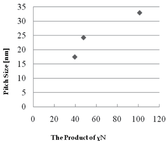
Fig. 7. The prediction of nanodots pitches of PS-PDMS BCPs with molecular weights of 30,000–7,500, 13,500–4,000, and 11,700–2,900.
