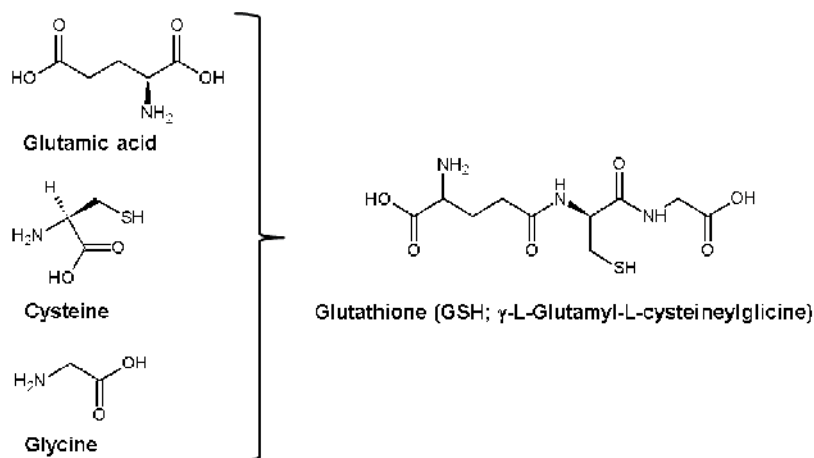
Fig. 1. Structure of glutathione
