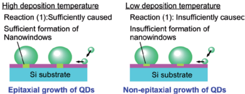
Fig. 4. Schematic of mechanism of epitaxial or non-epitaxial growth of QDs
