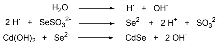
Fig. 8. Generation of \text{Se}^{2-} under sonication and preparation of CdSe nanocrystals
