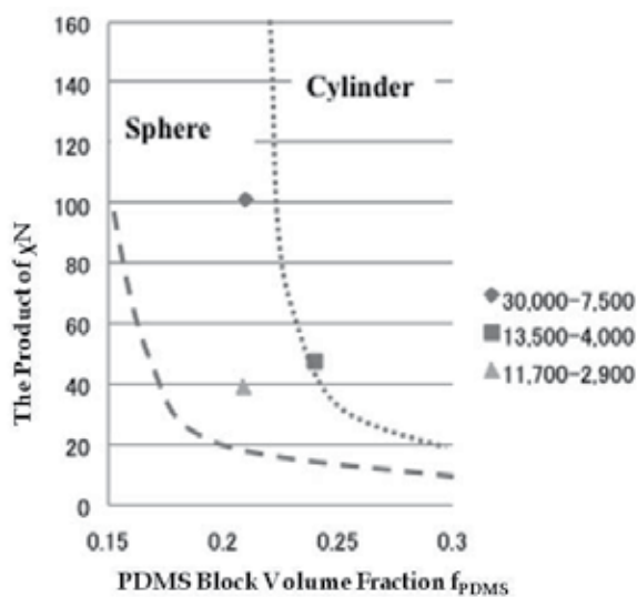
Fig. 11. The position of our adopted PS-PDMS in mean-field phase diagram for BCP melts.
