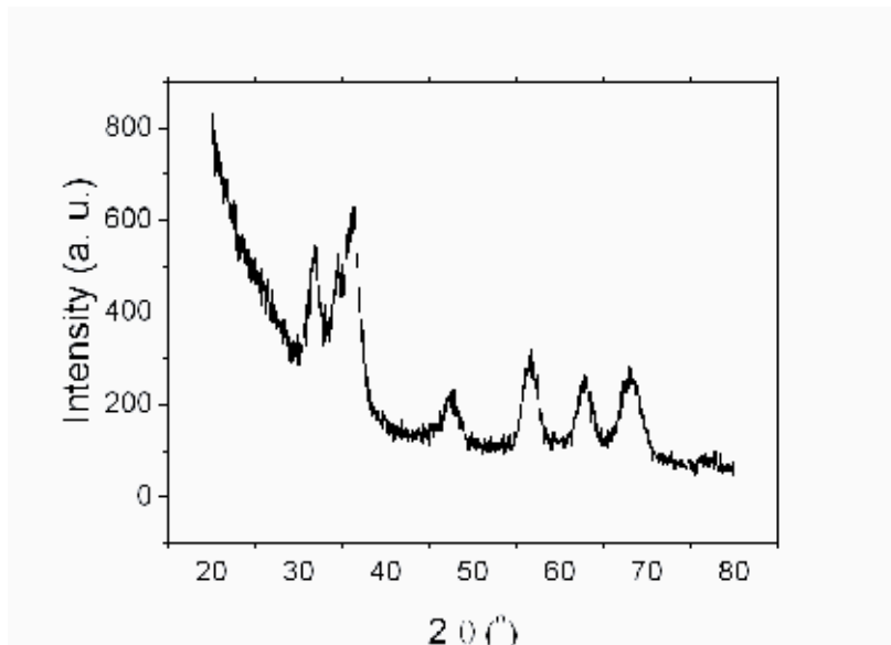
Fig. 2. XRD patterns of washed ZnO.
