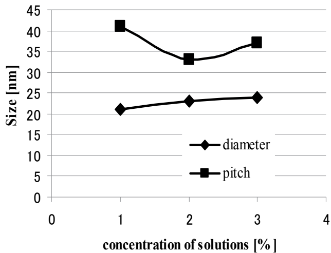
Fig. 4. Relation between nanodot size and concentration.
