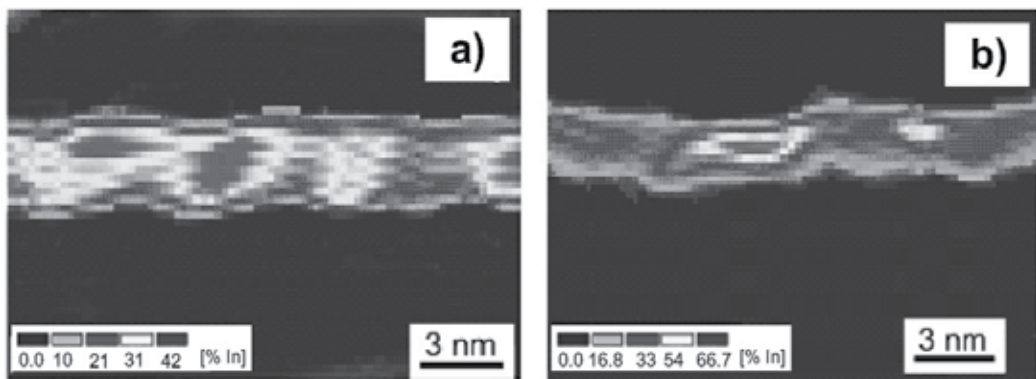
Fig. 5. HRTEM images of the InGaN QWs grown in nitrogen atmosphere (a) and with admixing of hydrogen during growth (b). (Tsatsulnikov et al., 2011a)
