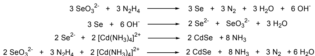
Fig. 7. Ultrasonic-assisted synthesis of CdSe nanocrystals
