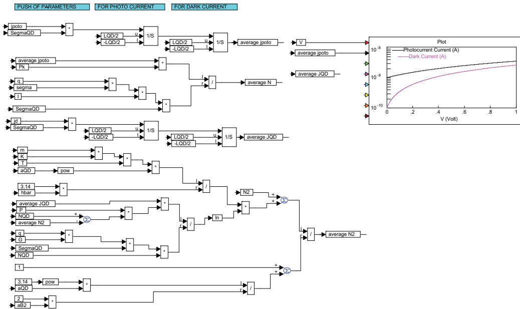
Fig. 3.3. Photocurrent density block diagram model of QDIPs.
