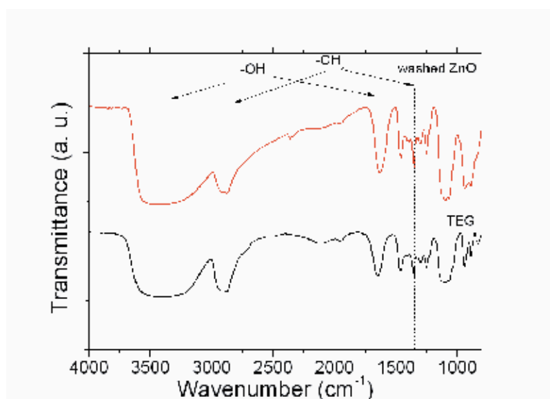
Fig. 5. FT-IR spectra of TEG and washed ZnO.
