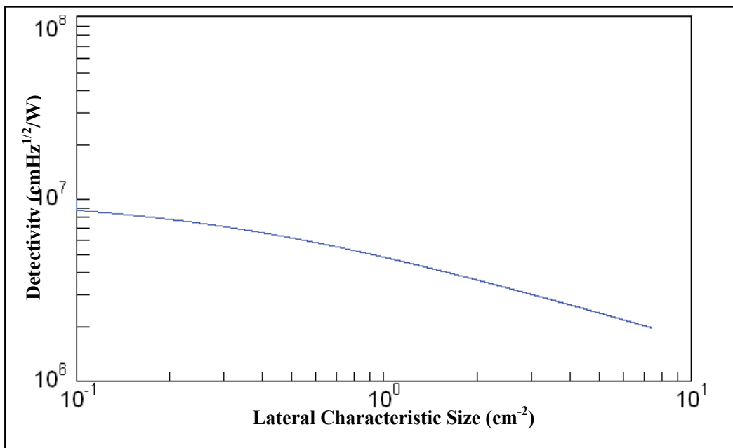
Fig. 3.12. Detectivity against a_{\text{QD}} .
