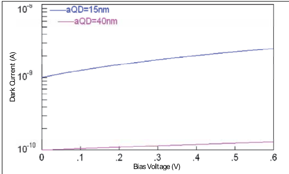
Fig. 3.7. Dark current and biasing voltage results at different lateral characteristic size of quantum dot.
