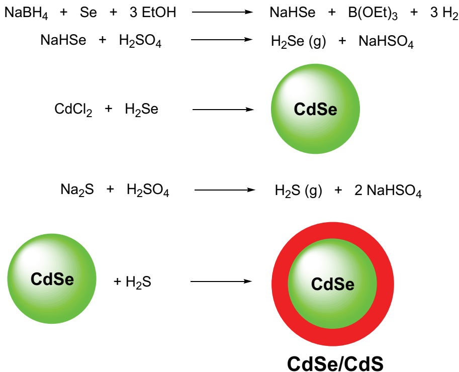
Fig. 15. Synthesis of core/shell CdSe/CdS QDs
