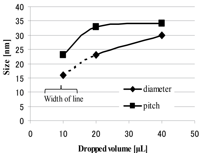
Fig. 6. Relations between the dropped volume of PS-PDMS solution and the size of nanodots. The dashed line indicates that the pattern morphology alters into random line.
