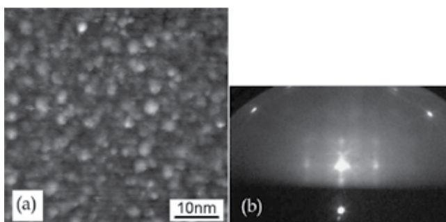
Fig. 6. (a) STM image and (b) RHEED pattern of the ultrathin SiO 2 films with predeposited Ge in 2-ML amounts at temperatures of 650°C.
