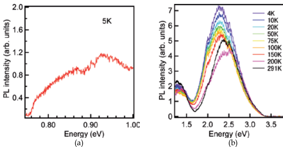
Fig. 18. PL spectra around 0.9 (a) and 2 eV (b) of SiO 2 /8-ML Ge 0.85 Sn 0.15 QDs/Si(001) structure.
