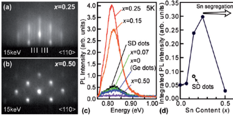
Fig. 14. (a), (b) RHEED pattern of Si/Ge 1-x Sn x QDs/Si(001) structures with x of 0.25 (a) and 0.5 (b). (c) PL spectra of Si/Ge 1-x Sn x QDs/Si(001) structures with various x. (d) Dependence of integrated PL intensity on Sn content x.
