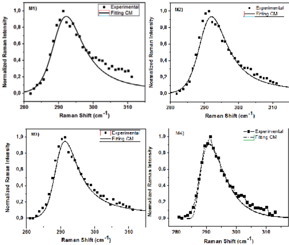
Fig. 8. Fitting on Raman spectra to the Confinement Model (CM). The square points are the experimental data and the continuous line is the CM by using the Eq(6).
