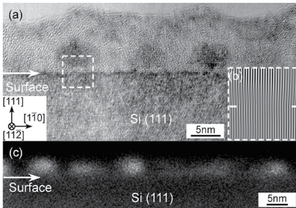
Fig. 8. (a) Cross sectional HRTEM image and (c) STEM image of epitaxial 8-ML Ge 0.85 Sn 0.15 QDs on Si(111) formed under the epitaxial QD growth condition. (b) IFFT image of dotted square area in (a). Two white lines in (b) indicate interface between QDs and substrate.
