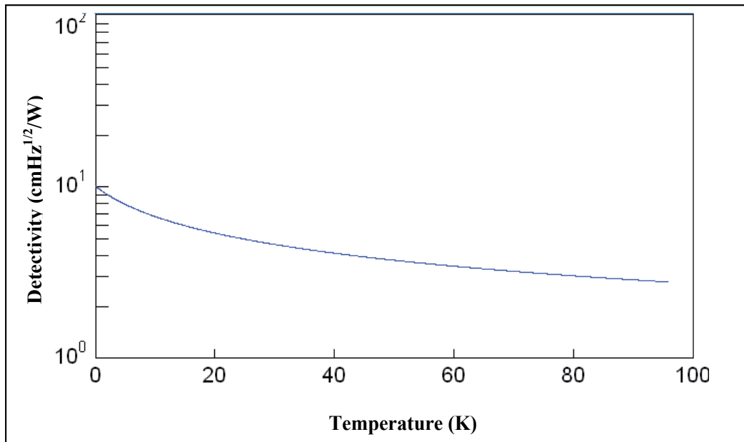
Fig. 3.9. Detectivity against temperature.
