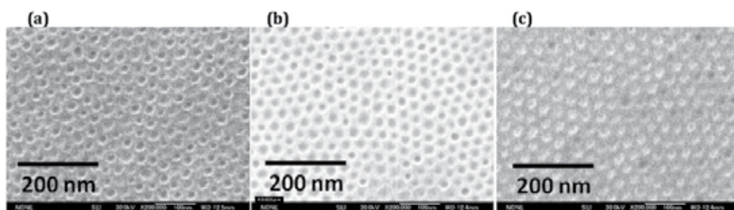
Fig. 3. Fabricated nanodots pattern using PS-PDMS block copolymer with molecular weight 30,000-7,500, which dissolved onto different concentrations those are 1%, 2%, and 3% corresponding to images (a), (b), and (c), respectively.
