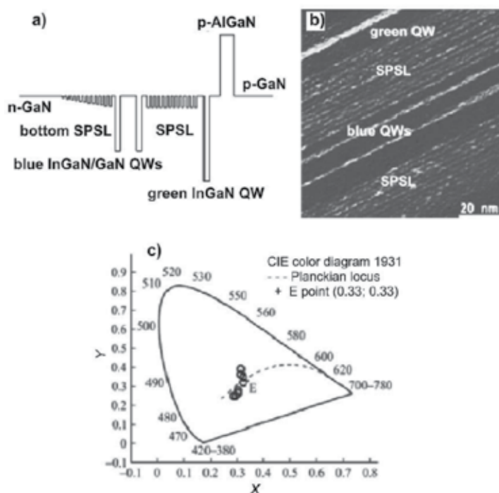
Fig. 12. Scheme (a), HRTEM image (b) of the active region of the monolithic white LED. . c- 1931 CIE chromaticity diagrams (points show chromaticity coordinates at various currents). (Tsatsulnikov et al., 2010c)
