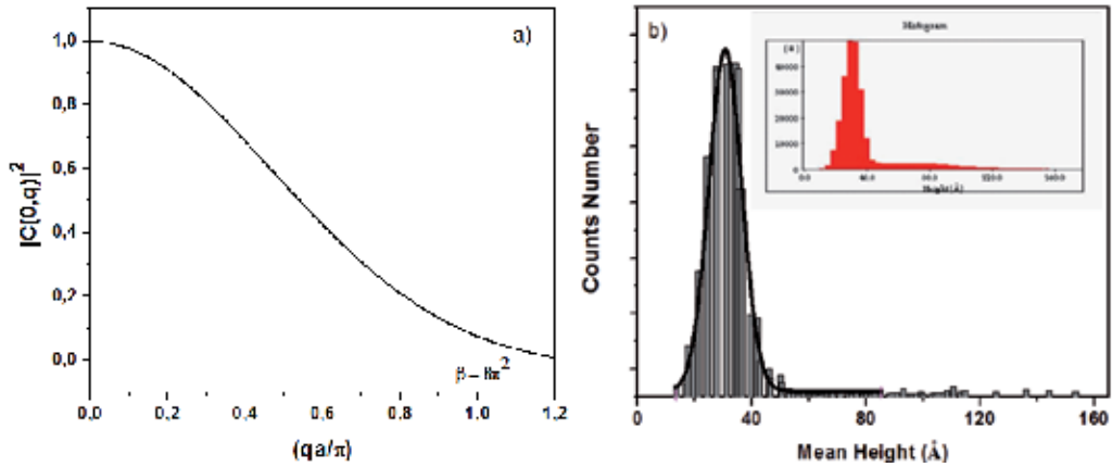
Fig. 6. (a) Squares of the Fourier transform |Q(0, q)|^2 used in the confinement phonon model (CM), \beta = 8\pi^2 . (b) Diameter distribution of the InAs Qdots (M4-sample) with mean height L = 35 Å. The solid curve is a log-normal fit to the distribution. The inset in (b) is the histogram of the sample M4.
