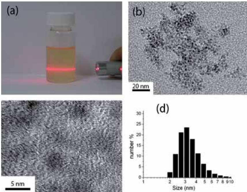
Fig. 1. (a) The Tyndall effect on as-prepared ZnO-TEG solution; (b) bright-field TEM image of as-prepared ZnO; (c) high-resolution TEM image of as-prepared ZnO; (d) size distribution of ZnO in TEG solution.
