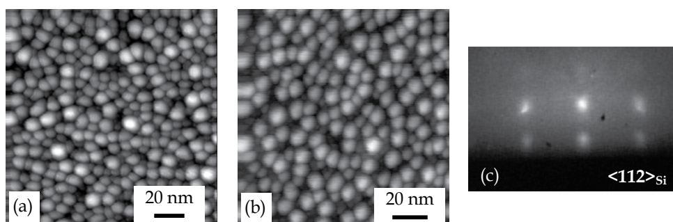
Fig. 2. STM images of Si (a) and Ge QDs (b) on Si (111) substrates formed by deposition of 8-ML Si and 5-ML Ge. (c) RHEED pattern of Ge QDs shown in (b).
