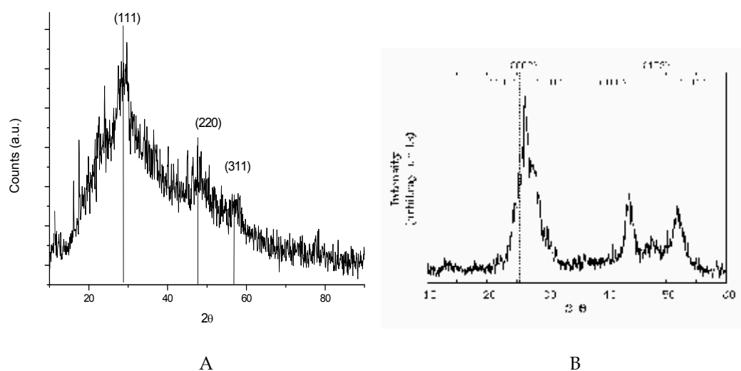
Fig. 4. Diffraction patterns of synthesized A)ZnS and B)CdS.
