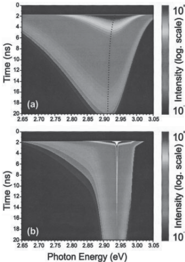
Fig. 2. Time/wavelength plots of PL for nonresonant (a) and resonant (b) excitations for sample grown at 820 °C. White spot corresponds to the scattered laser light. (Krestnikov et al., 2002a)
