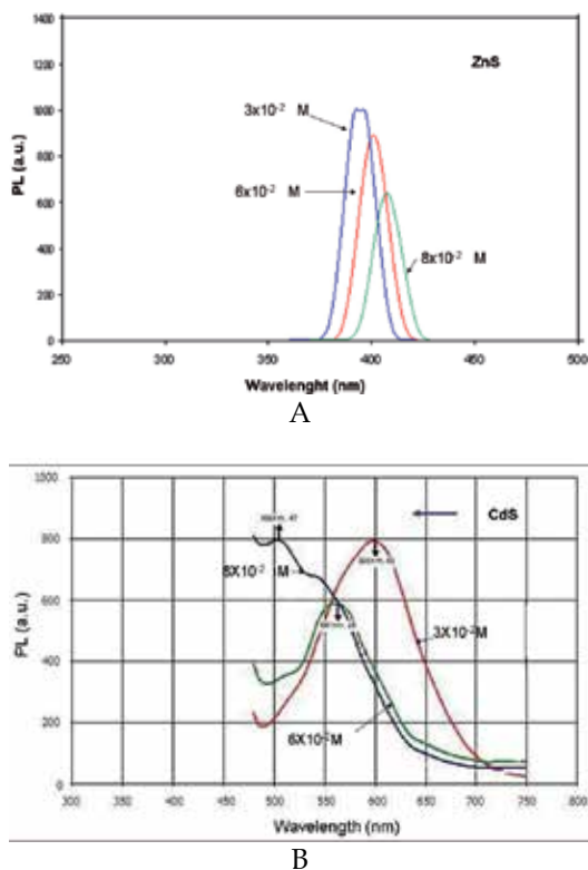
Fig. 2. PL spectra for ZnS and CdS.
