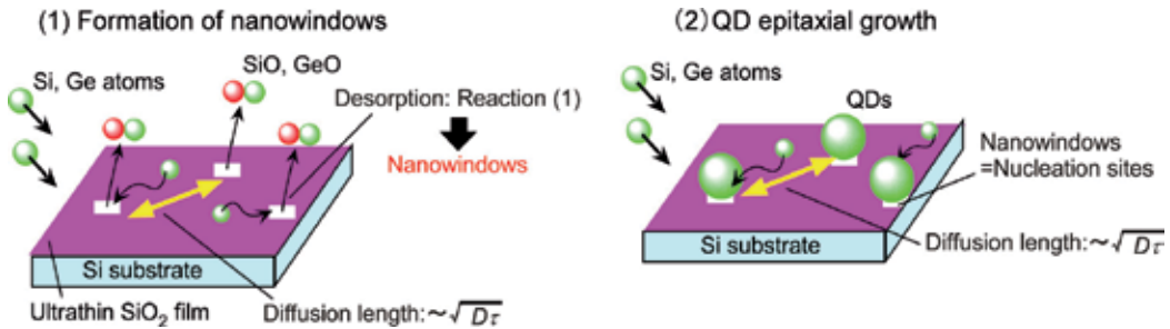
Fig. 3. Illustration of mechanism of ultrahigh density QD formation by ultrathin \text{SiO}_2 film technique.
