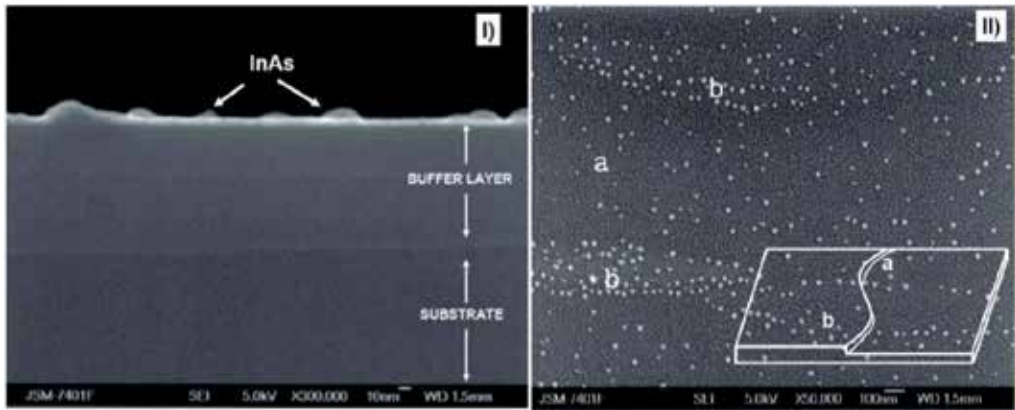
Fig. 2. (I) Cross-sectional HRSEM image ( \times 300,000 ) of InAs SAQDs. (II) Plane view HRSEM image ( \times 50,000 ) of InAs SAQDs. The inset shows schematically the preferential sites for SAQDs nucleation.
