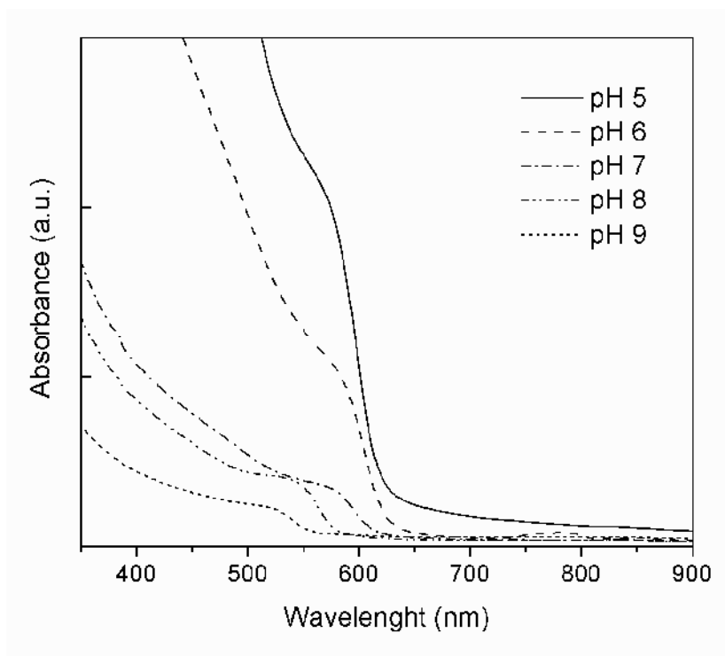
Fig. 8. UV-Vis spectra for CdSe at different pH values.
