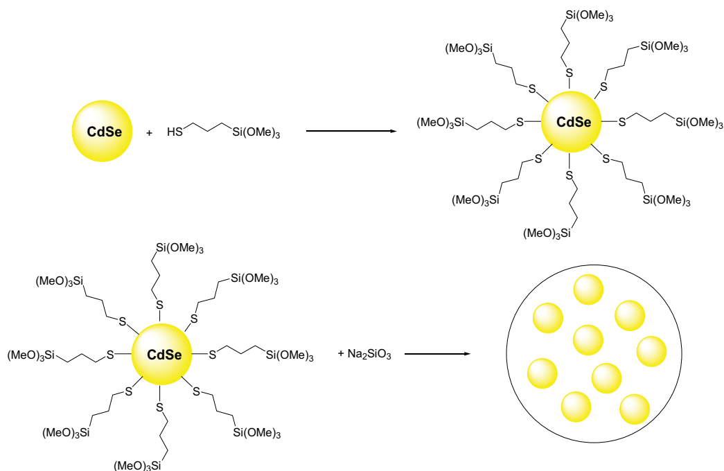
Fig. 12. Preparation of silica nanospheres containing CdSe QDs
