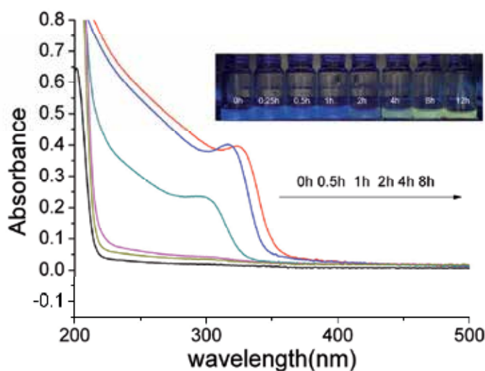
Fig. 8. UV-Vis absorbance spectra of UV-light irradiated TEG solution. The inset depicts the colours of emission light under UV light irradiation.
