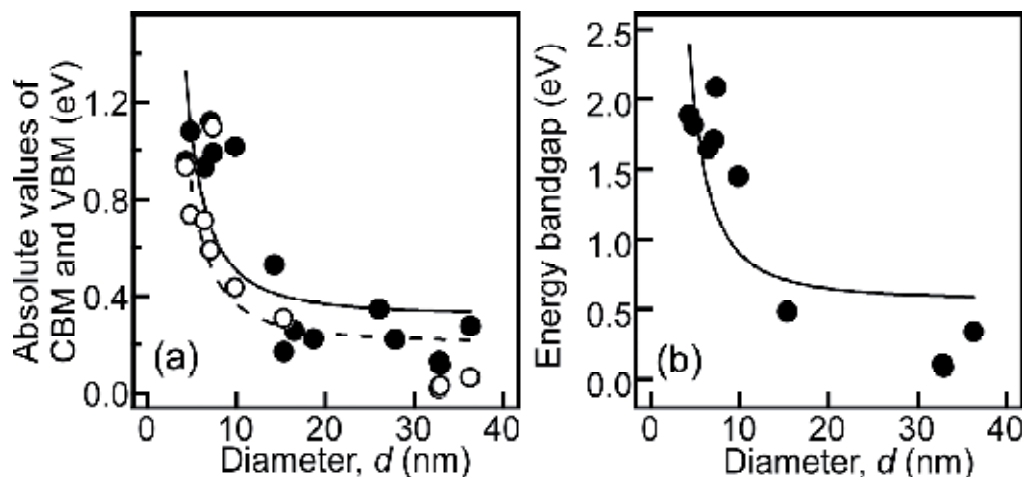
Fig. 10. (a) CBM (circles) and VBM (cricles) estimated from STS results of Ge 0.85 Sn 0.15 QDs. (b) Energy bandgap calculated from CBM -VBM .
