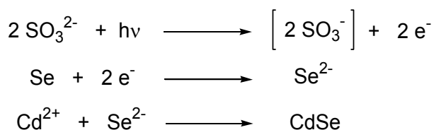
Fig. 14. Photo-assisted synthesis of CdSe nanoparticles
