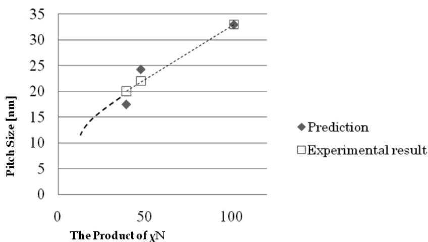
Fig. 10. A graph of the pitch sizes of nanodots according to prediction and experimental results.
