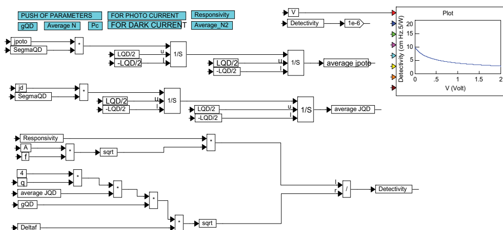
Fig. 3.4 Detectivity block diagram model of QDIPs.
