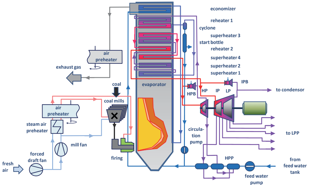
Fig. 15. Structure of the power plant model
