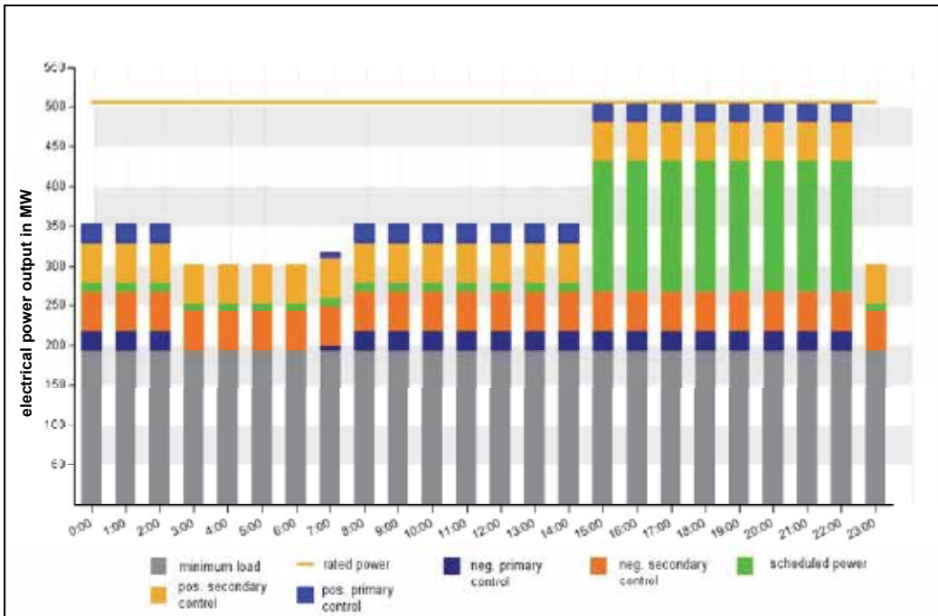
Fig. 11. Simulated schedule with reserved control areas for primary and secondary control for a single power plant
