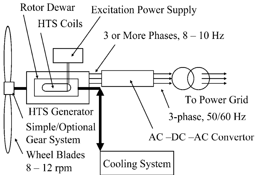
Fig. 7. The schematic diagram of a HTS generator system.
