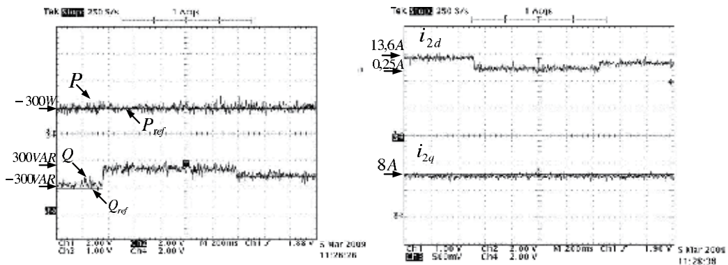
(a) Response of step test of the reactive power (800VA/div.).
