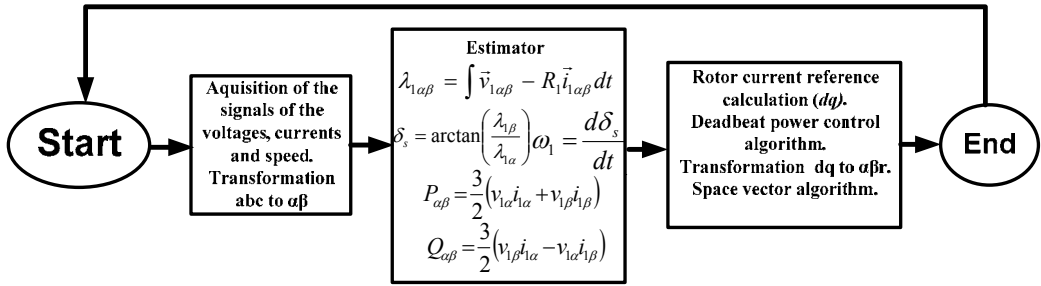
Fig. 5. The flowchart of the DSP program.
