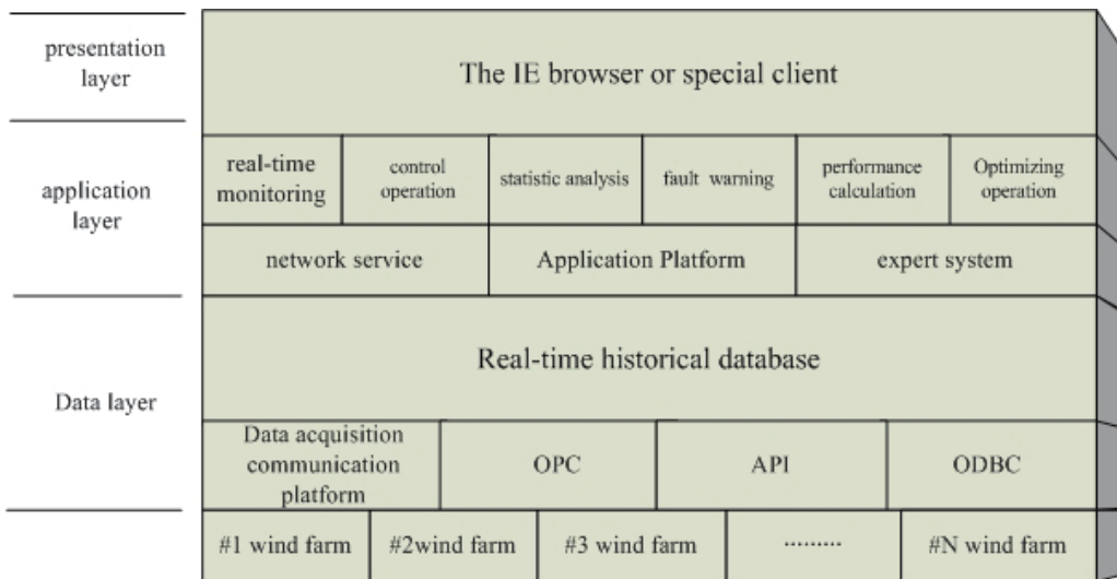
Fig. 4. The design of software structure
