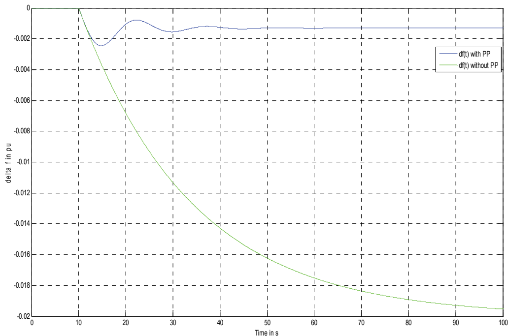
Fig. 2. Frequency deviation in pu while \Delta p_{GV} = +1\%
