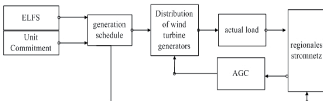
Fig. 15. Automatic generation control(AGC)
