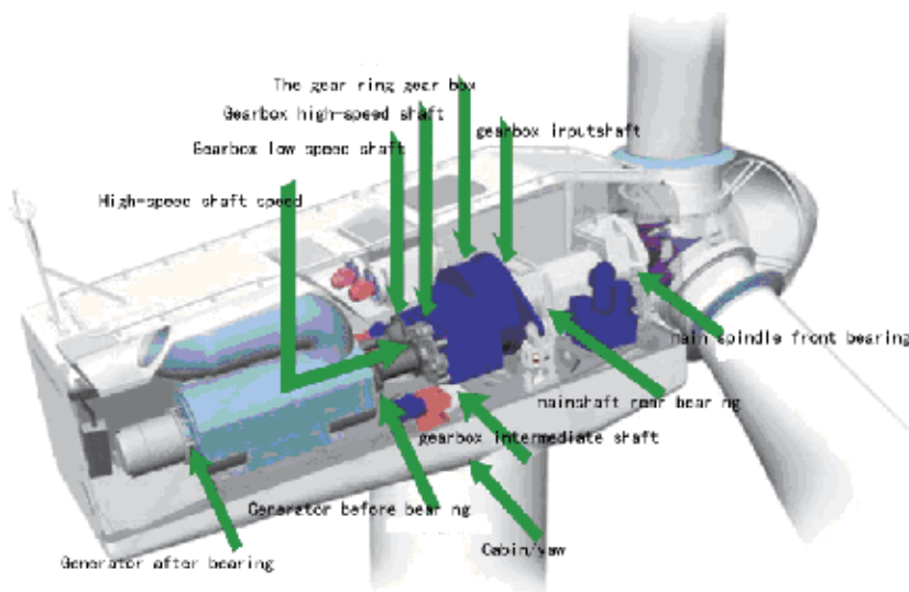
Fig. 11. The scheme of fans' monitoring
