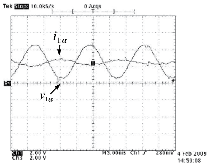
Fig. 12. The stator voltage(18V/div.) and current (0.38A/div.).
