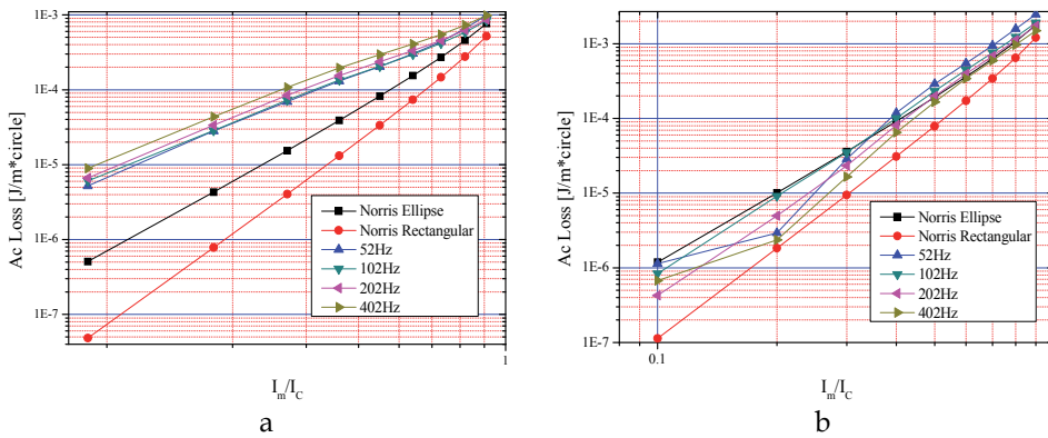
Fig. 22. AC losses in 344C YBCO (a) and Bi2223 (b) superconducting wires compared with the predictions of the Norris model.
