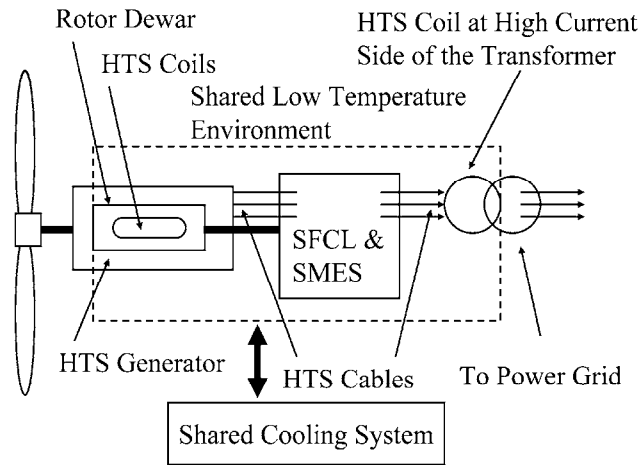
Fig. 25. Combination of HTS devices in the wind farm.
