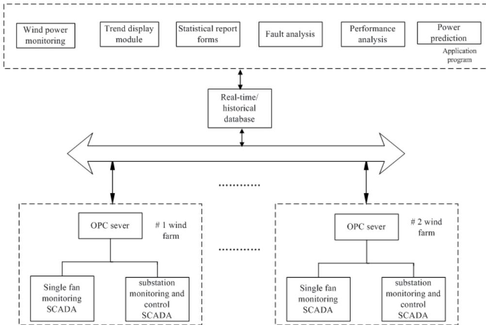
Fig. 3. SCADA software development diagram
