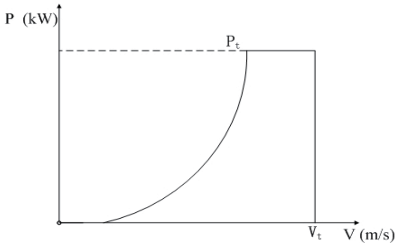
Fig. 13. The wind generators' power characteristics
