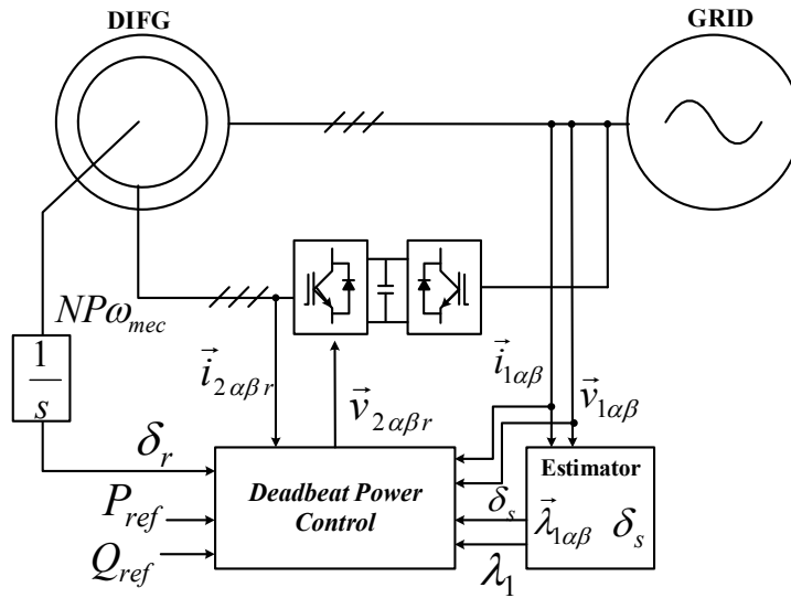
Fig. 3. Deadbeat power control diagram for DFIG.
