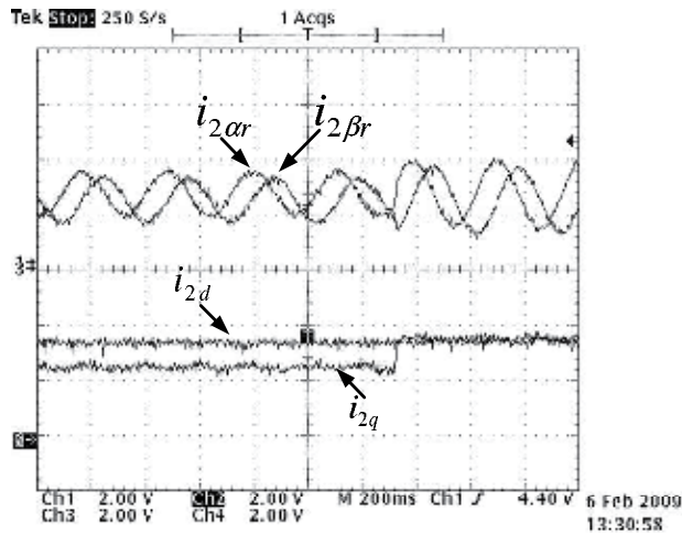
Fig. 9. Response of step test for i_{2q} (1.66 A/div.).
