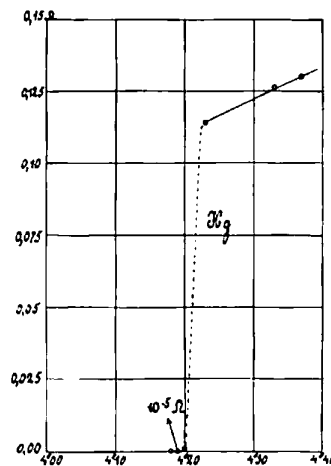
Fig. 1. The zero resistance transition of Hg measured in 1911 by Kamerlingh Onnes.
