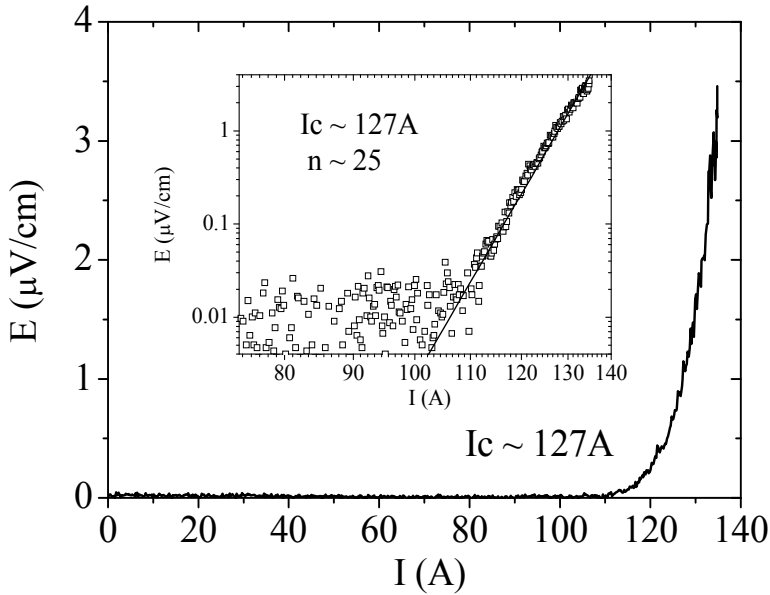
Fig. 4. The electric field - current (E-I) correlations measured in HTS wire at 77 K, self field. The inset plots the same curve in exponential coordinates to show the estimation of n value.
