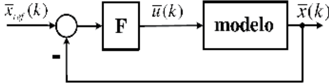
Fig. 2. Deadbeat control block diagram.
