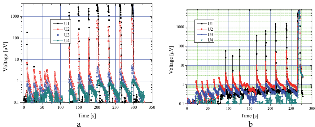
Fig. 19. Thermal heating induced quench in HTS wires working at 0.5 (a) and 0.9 (b) I_c .
