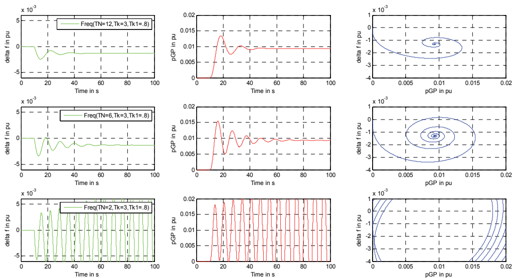
Fig. 5. Effect of a reduced acceleration time constant due to reduced inertia onto the primary controller stability
