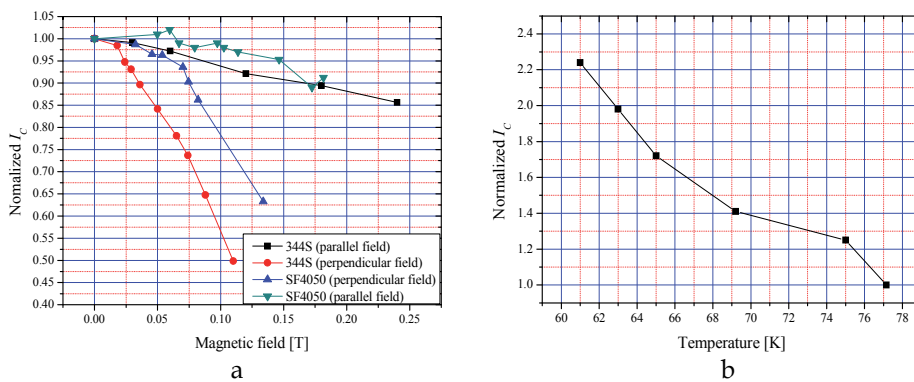
Fig. 11. Normalized I_c vs. field (a) and temperature (b) in wires from SuperPower and AMSC.
