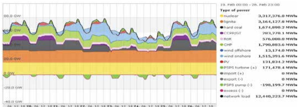
Fig. 13. 7 days period – winter scenario 2010 without import/export capability
