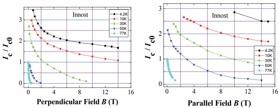
Fig. 12. Normalized I_c vs. field and temperature in wires from Innova.
