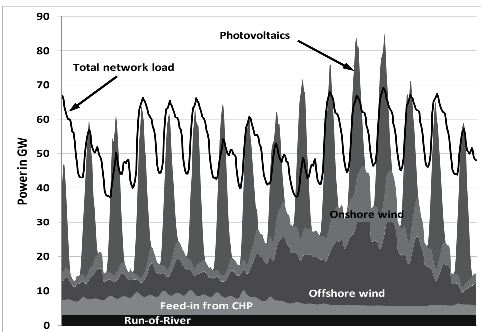
Fig. 12. Non-dispatchable power feed-in for a two weeks summer period in 2025
