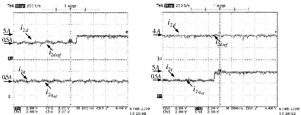
(a) Response of step test of the i_{2d} .
