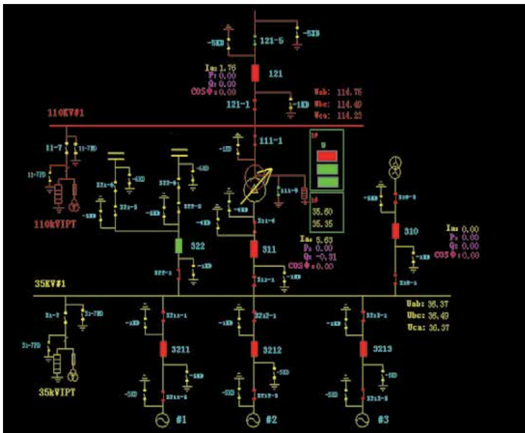
Fig. 16. Automatic generation control(AGC)
