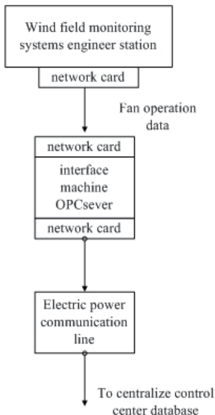
Fig. 6. OPC application program structure
