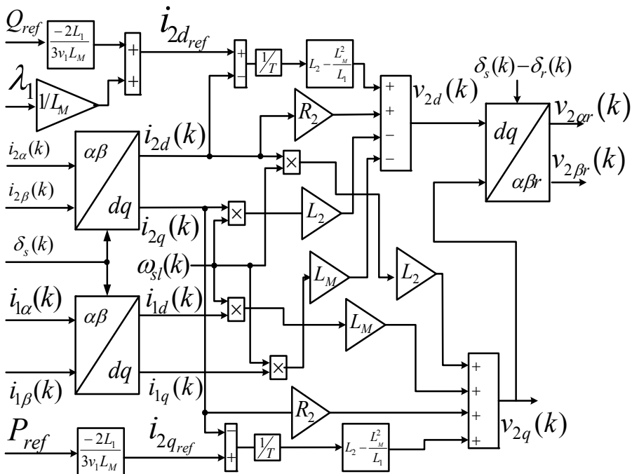
Fig. 4. Detailed deadbeat power control algorithm.
