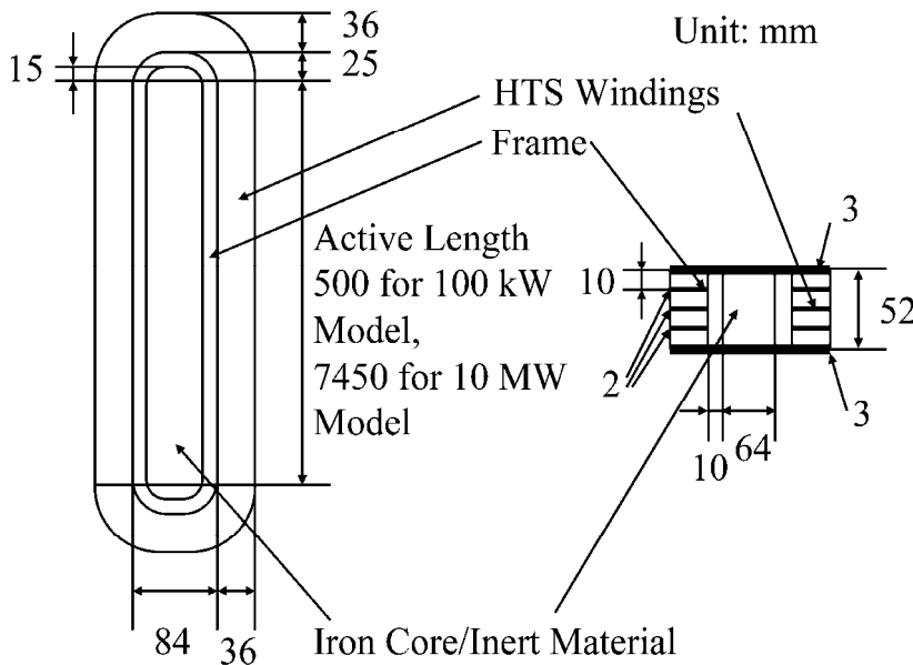
Fig. 10. Scheme of the excitation coil in the model generator.
