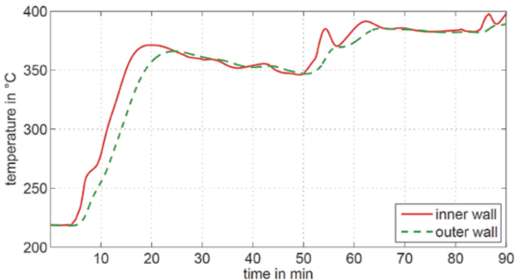
Fig. 16. Metal temperatures in the SH 2 outlet header
