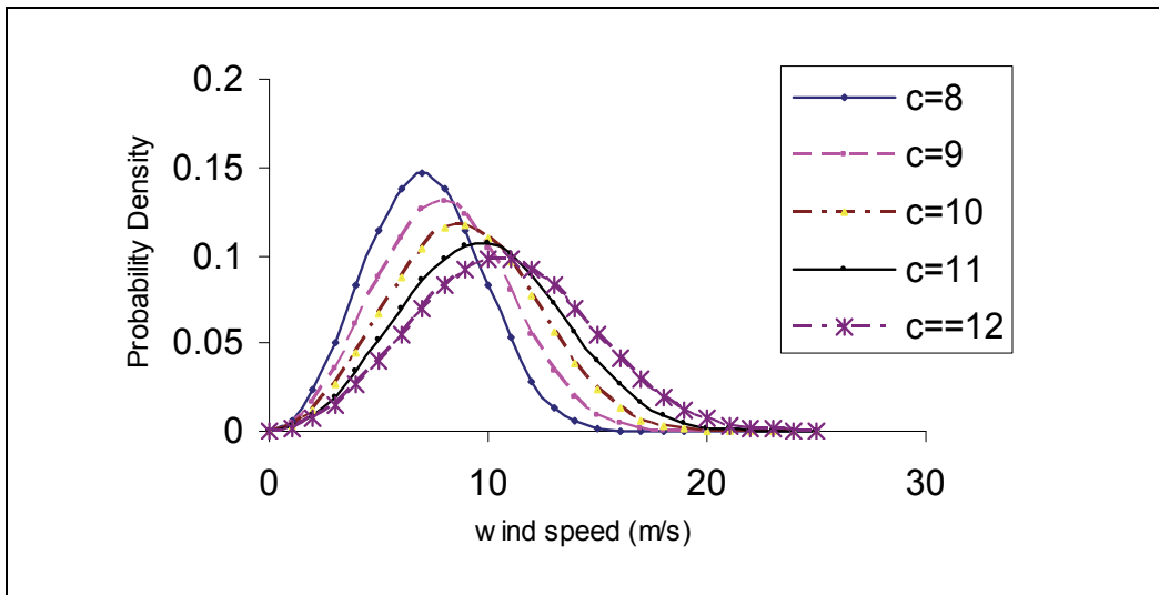
Fig. 2. Weibull Distribution Density versus wind speed under a constant value of k=3 and different values of c
