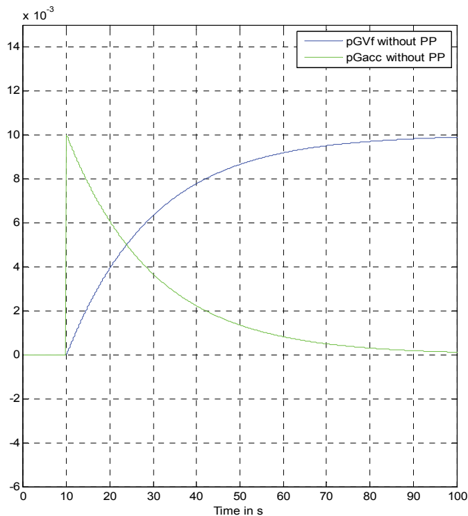
Fig. 3. Disturbance of the power balance covered by accelerating power and the consumer self-controlling effect
