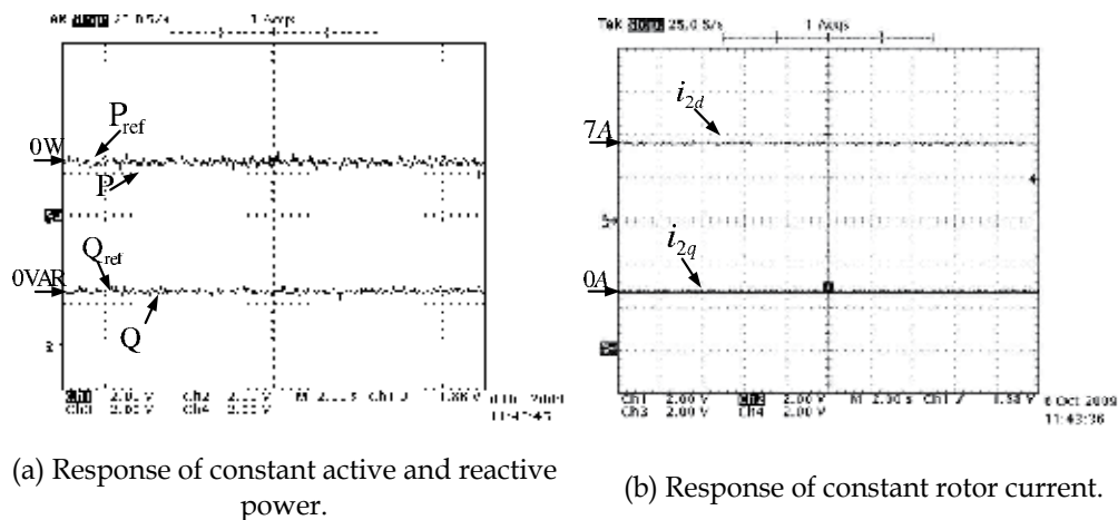
Fig. 13. Response of the active and reactive power and rotor current.
