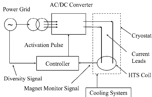
Fig. 17. Schematic diagram of SMES.
