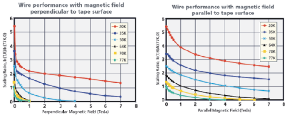
Fig. 13. Normalized I_c vs. field and temperature in Bi2223 wires from AMSC (AMSC 2009).
