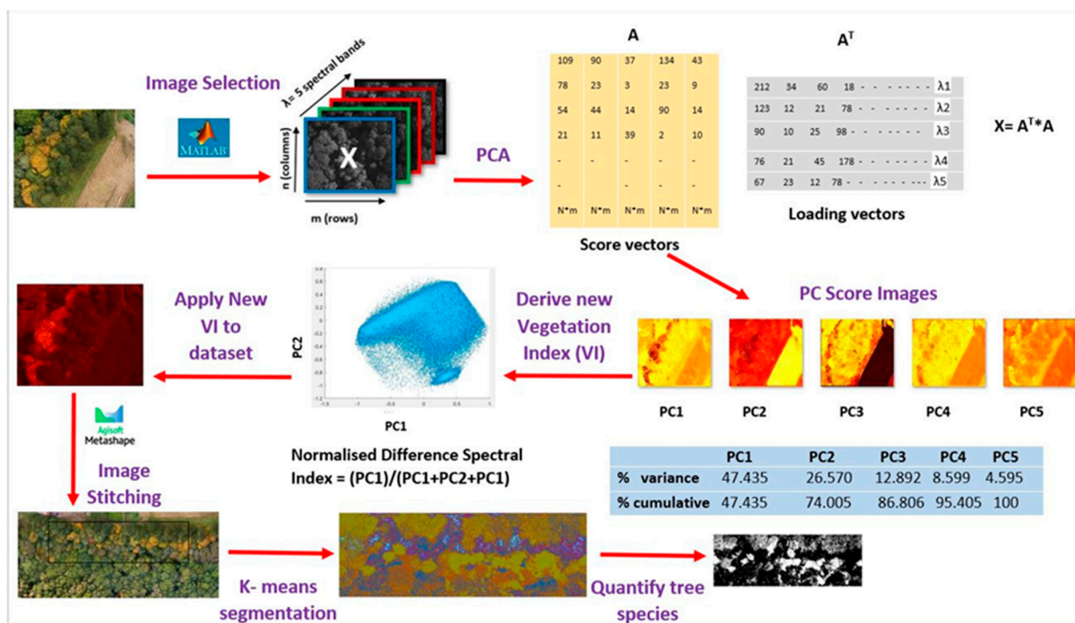
Figure 2. Workflow of the data processing required to investigate the ASNW.
