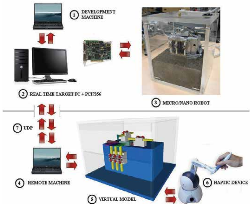
Fig. 8. Micro/nanorobot system components
