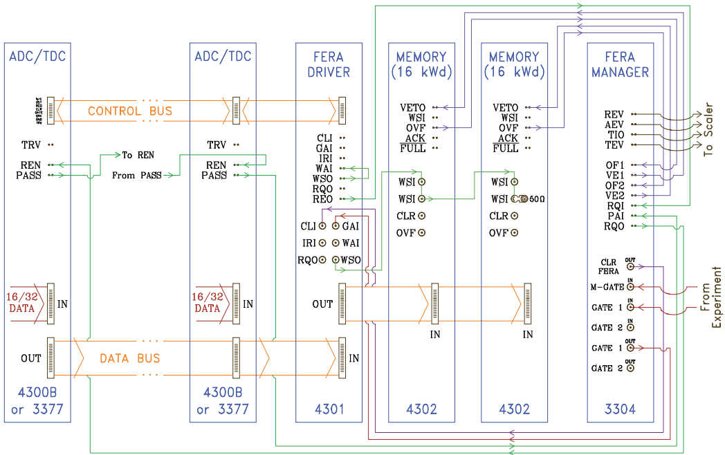
Fig. 1. Diagram of the standard FERA System interconnections.
