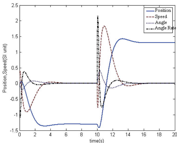
Fig. 8. Reaction to a ramp shaped speed input
