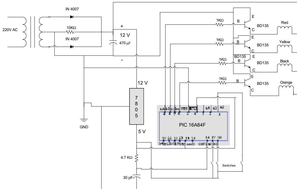
Fig. 11. Complete circuit diagram
