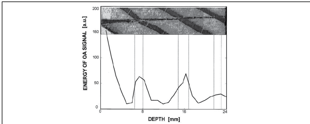
Fig. 9. Energy of optoacoustic signals vs. wood density profile. Reprinted from (Grad & Možina, 1998) with kind permission from Elsevier
