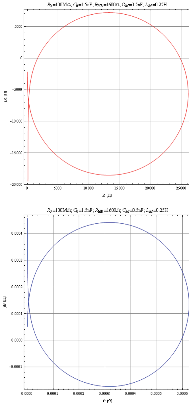
Fig. 2.2.4 Circle diagrams of input electric impedance and admittance of piezoelectric transducer at R_{MR}=1600\Omega , L_M=0.25\text{H} , C_M=0.5\text{nF} i C_0=1.5\text{nF} , R_c=50\Omega
