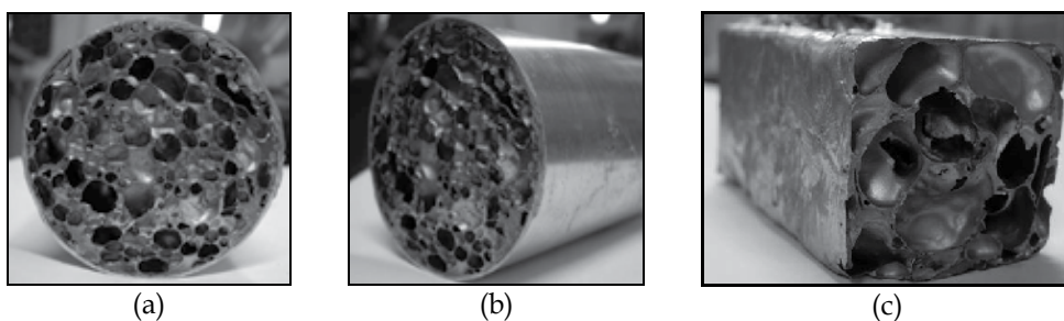
Fig. 7. MGI foam cores attached by mechanical bonding (front and lateral view (a-b) and foam part with parallelepiped shape (c))
