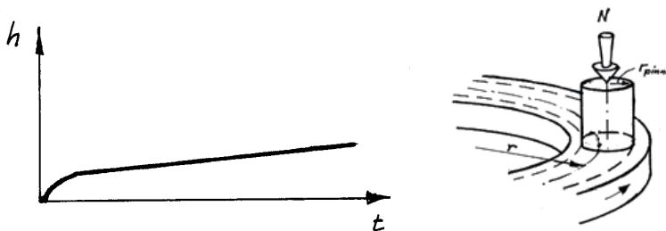
Fig. 8. A schematic wear curve from a pin-on-disc test with a flat ended cylindrical pin
