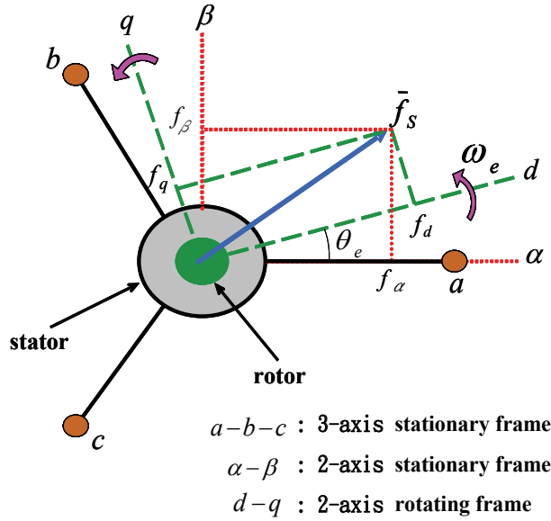
Fig. 2. Transformation between stationary axes and rotating axes
