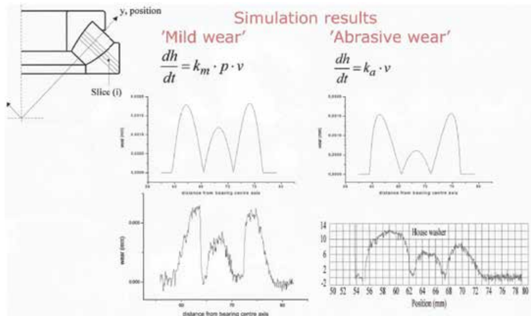
Fig. 3. Abrasive wear compared with mild sliding wear
