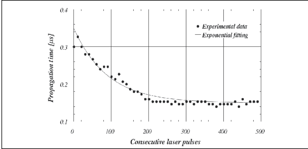
Fig. 11. Propagation time of the longitudinal stress waves vs. the number of consecutive laser pulses during laser drilling of a 1.2-mm thick stainless-steel sample. Experimental data are fitted with an exponential curve. Reprinted from (Strgar & Možina, 2002b) with kind permission from Springer Science+Business Media
