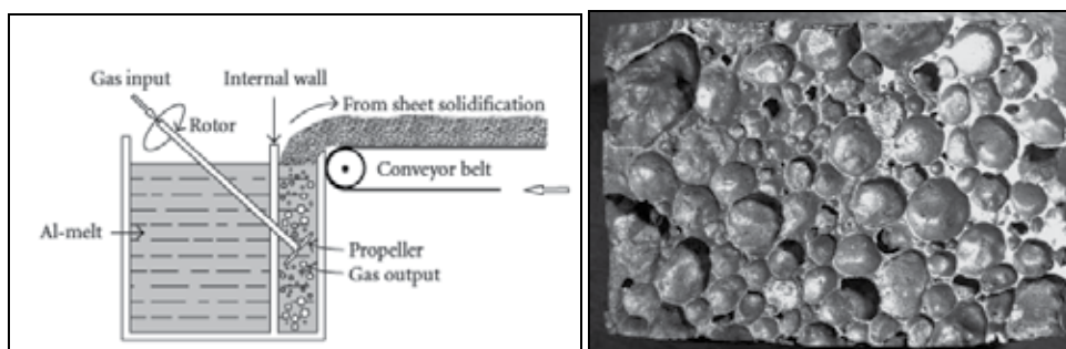
Fig. 6. Apparatus for MGI and example of foam obtained by MGI
