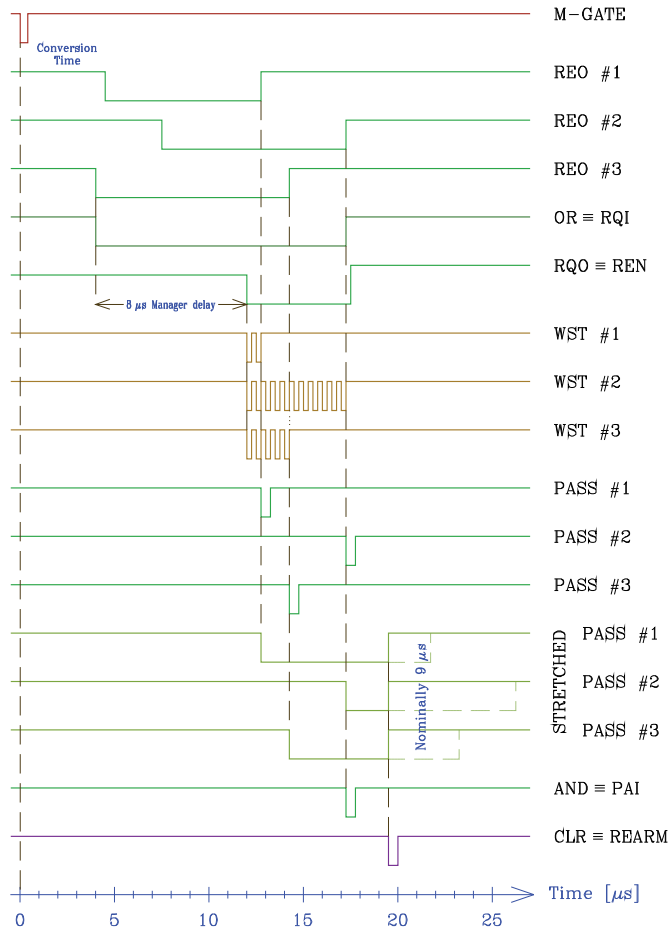
Fig. 5. FERA Readout timing – the most relevant signals for the Full FERA system shown in Fig. 4. To make the short pulses visible they are shown not to scale – the width of the M-GATE is about 50-100 ns, the write strobes (WST) are 50 ns wide with a 100 ns spacing, the PASS and CLR pulses are about 60-80 ns wide.
