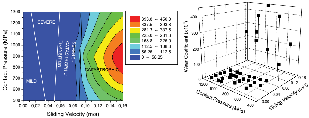
Fig. 6. Wear coefficient map according to Lewis and Olofsson [9].
