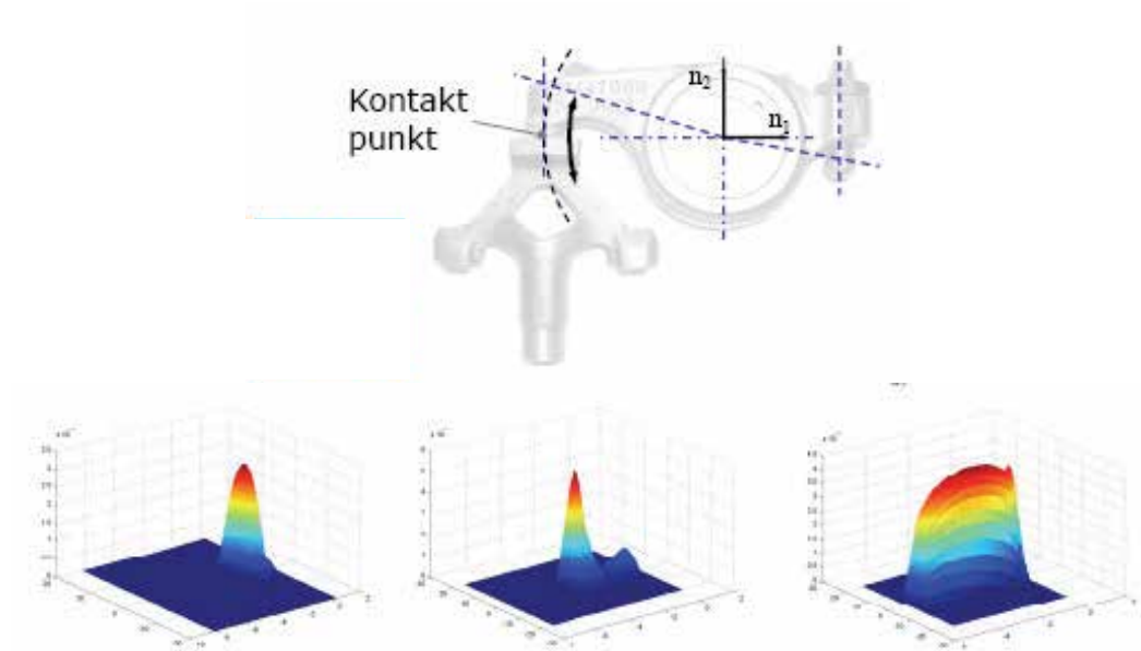
Fig. 17. Some wear simulation results obtained by Spiegelberg [23]
