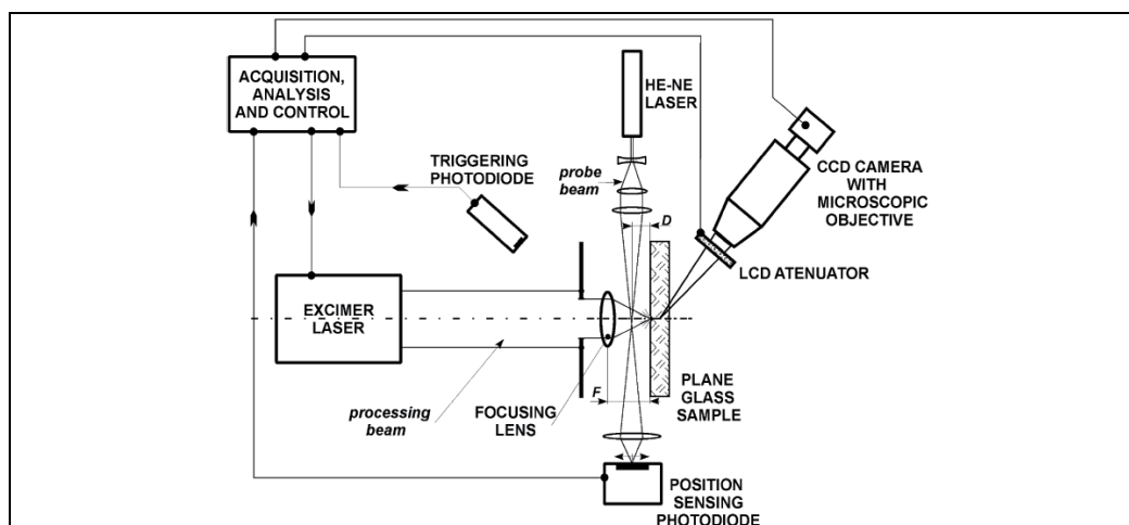
Fig. 14. The set-up for laser drilling of specified micro-holes into ampoules. Reprinted from (Petkovšek et al., 2008) with kind permission from Springer Science+Business Media
