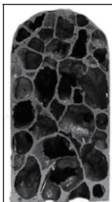
Fig. 8. \text{TiH}_2 foam sample obtained by cold uniaxial pressure
