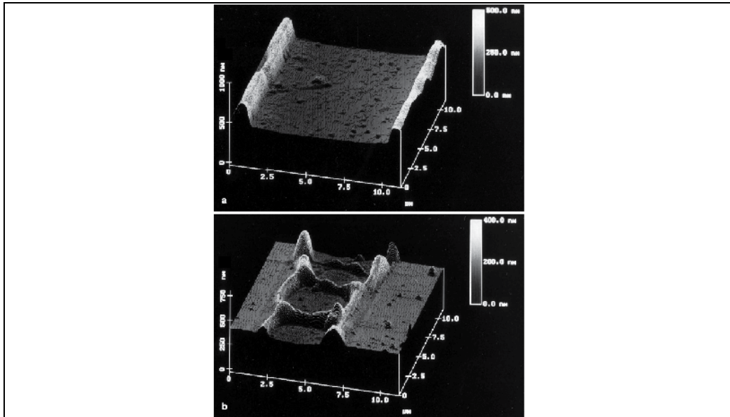
Fig. 22. AFM images of graduation lines for different writing parameters (size 11 \times 11 \mu\text{m} ). Reprinted from (Kopač et al., 1996a) with kind permission from Springer Science+Business Media
