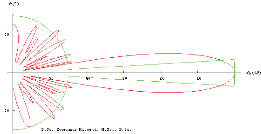
Fig. 6.3.1 Directivity patterns of sonar antenna at elliptic CS of the main lobe, if we have azimuth angle \theta_{-3\text{dB}}=4.8^{\circ} and the value of given elevation angle \varphi_{-3\text{dB}}=15^{\circ} then with the level of suppression of minor lobes of characteristic LoSoS = -45 \text{ dB} we have that is DI=28.5 \text{ dB}
