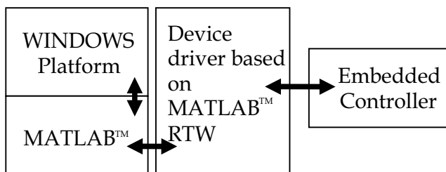
Fig. 9. MATLAB TM RTW Kernel
