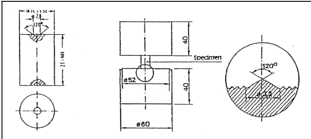
Fig. 3. Test specimens and grooved dies used in standardized upsetting testing (Kudo, 1975).
