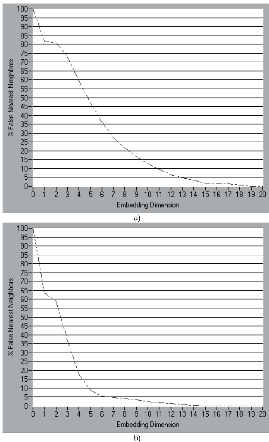
Fig. 4. Embedding dimensions d determined with false nearest neighbor a) for an active driver d = 19 , b) for a mild driver d = 15
