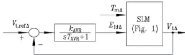
Fig. 3. Block diagram of SLM with voltage control
