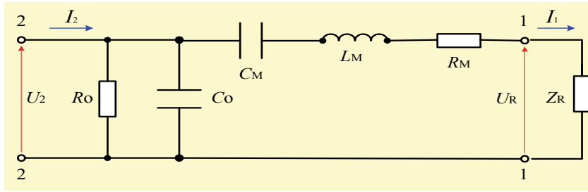
Fig. 2.2.1 Electric block scheme is given in a general form of equation of electric parameters on the input and electric analogy of mechanical parameters of vibration system
