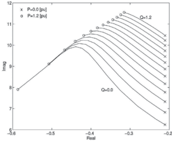
Fig. 2. Conjugate eigenvalue loci as a function of loading, turbogenerator, 160 MVA
