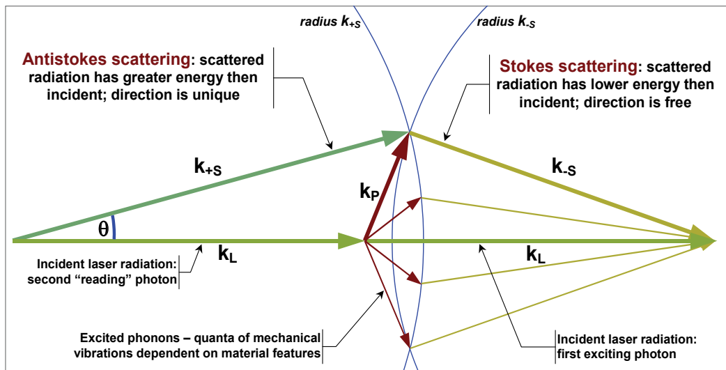
Fig. 15. A schematic diagram of the Raman scattering mechanism (multi-photon/phonon interaction)
