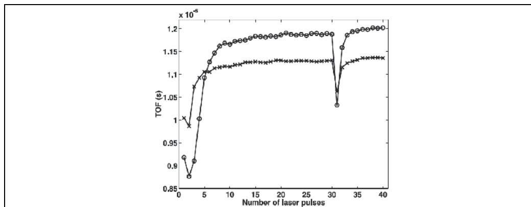
Fig. 19. Times of flight of the OD signals detected during the laser cleaning of a stainless-steel surface with low (×) and high (°) surface contaminant particle density. Reprinted from (Bregar & Možina, 2003) with kind permission from Springer Science+Business Media
