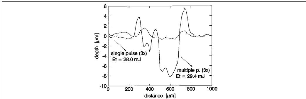
Fig. 24. Profiles of craters ablated into a stainless steel surface using single pulses (the dash-dot line) and multiple pulses (the solid line) with similar total energy. Reprinted from (Diaci & Možina, 1993) with kind permission from Elsevier
