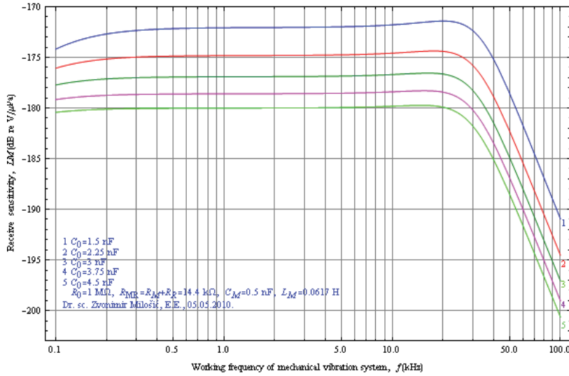
Fig. 4.3 Functional dependence of the level of the receive voltage sensitivity on the frequency at different parameters contained in mechanical, electric and acoustical part of transducer body calculated with given different numerical values of C_0 noticed inside figure
