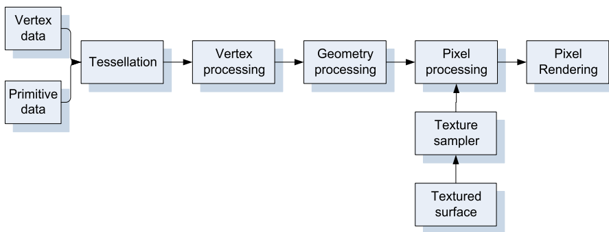
Fig. 2. Direct 3D graphics pipeline
