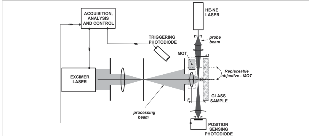
Fig. 13. The set-up for laser drilling of specified micro-holes into ampoules
