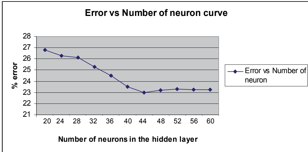
Fig. 8. Performance (in % error) curve on the neuron number in the hidden layer
