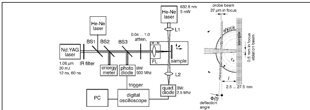
Fig. 2. A typical LBDP set-up
