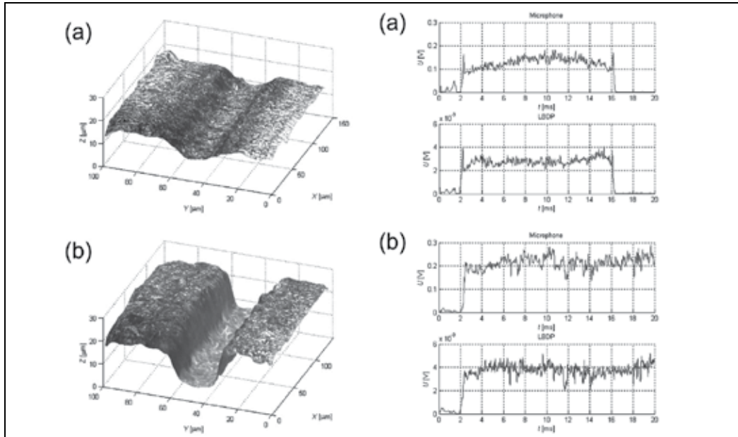
Fig. 18. 3D scans (left) and amplitudes of OD signals (right) of a shallow (a) and good (b) engraving. Reprinted from (Gorkič et al., 2009) with kind permission from Springer Science+Business Media
