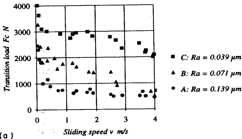
Fig. 7. The influence of surface roughness on the transition load of a lubricated sliding steel contact. Ball ( d=10 mm) and disc material: SAE52100, H_{v,ball} = 8000-8500 MPa, H_{v,disc} = 5800-6300 MPa, R_{a,ball} = 0.008\mu\text{m} . Lubricant: ISO VG 46 mineral oil. [12]
