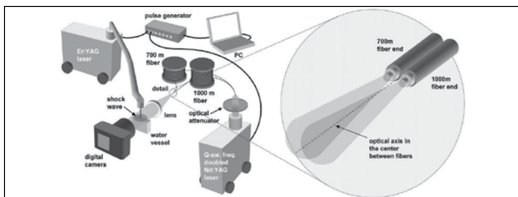
Fig. 6. A novel double-exposure shadowgraph set-up. Reprinted from (Perhavec & Diaci, 2010) with kind permission from Strojniški vestnik – Journal of Mechanical Engineering
