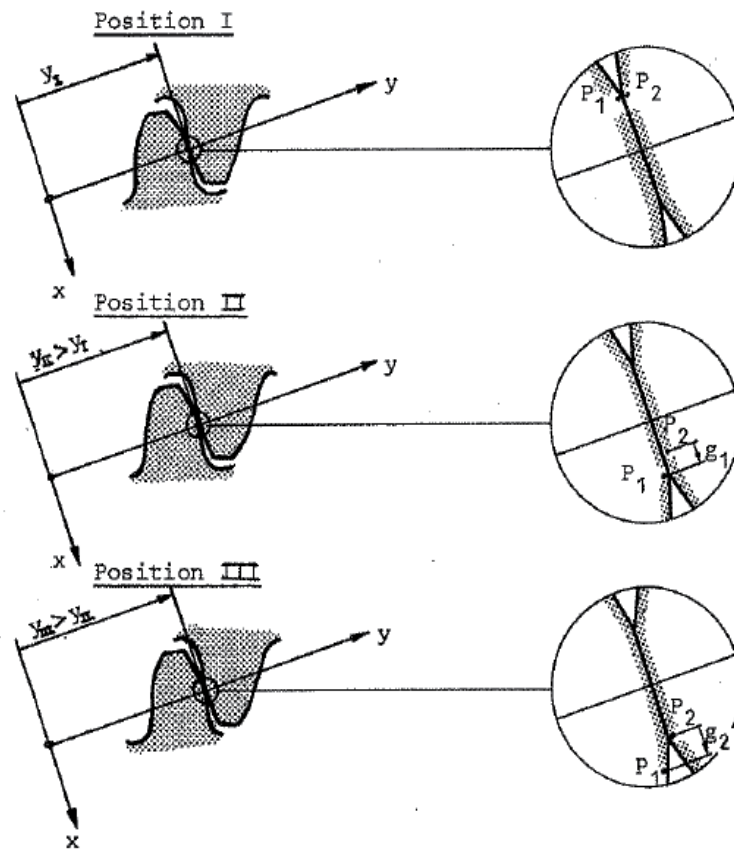
Fig. 9. The distance, g_1 , point P_1 on the pinion flank and the distance, g_2 , point P_2 on the gear flank slide during one mesh; position I corresponds to the moment in time when P_1 and P_2 come into contact with each other, while positions II and III correspond to the moments in time when P_1 and P_2 disengage, respectively. [8]
