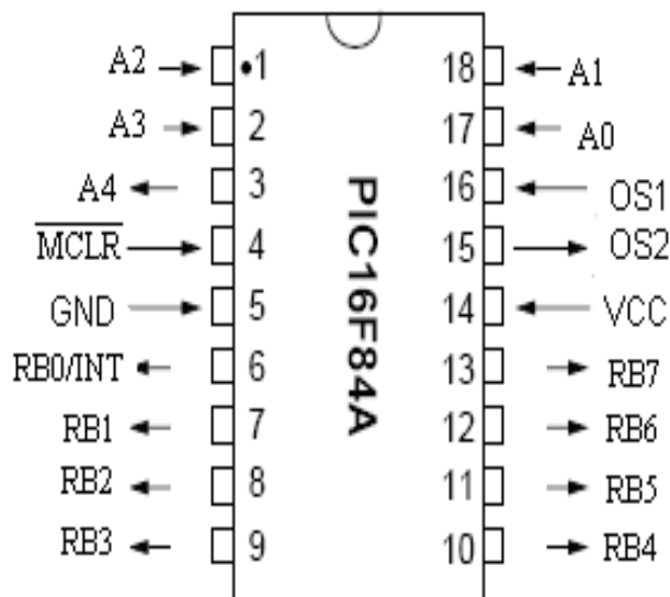
Fig. 9. PIC 16F84A Microcontroller outline
