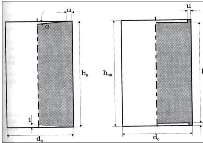
Fig. 2. Test specimens of compression test (ICFG document 11/01, 2001).
