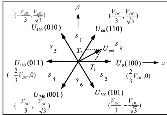
Fig. 4. Basic vector space and switching patterns
