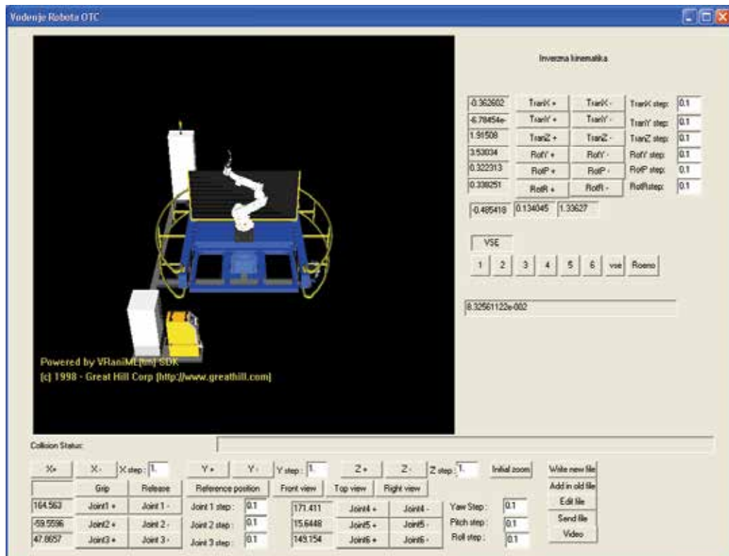
Fig. 5. Teach pendant of the telerobotic application using a haptic device
