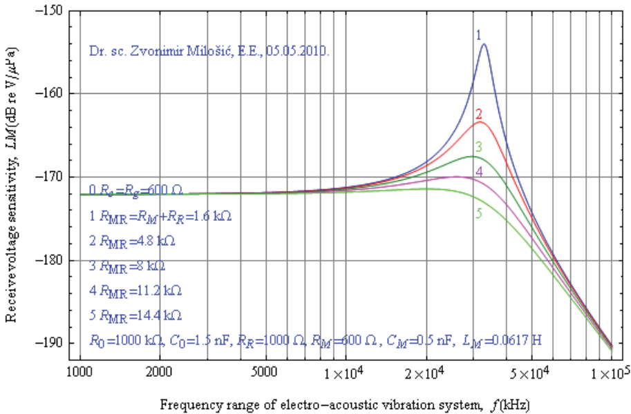
Fig. 4.2 Functional dependence of the level of the receive voltage sensitivity on frequency at different parameters contained in mechanical, electric and acoustical part of transducer body calculated with given numerical values inside figure
