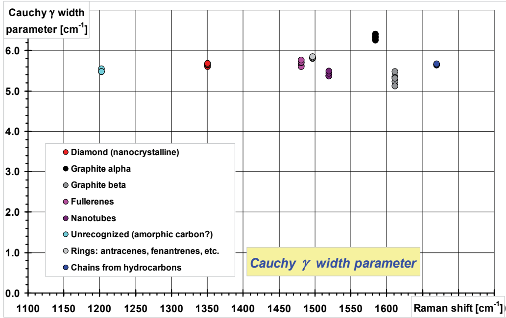
Fig. 21. Distribution of the \gamma parameter for all the analyzed peaks in the five Raman spectra of the hard carbon layers
