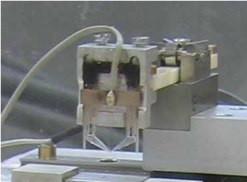
Fig. 9. Close look of a real micro/nano-robot tip gripper
