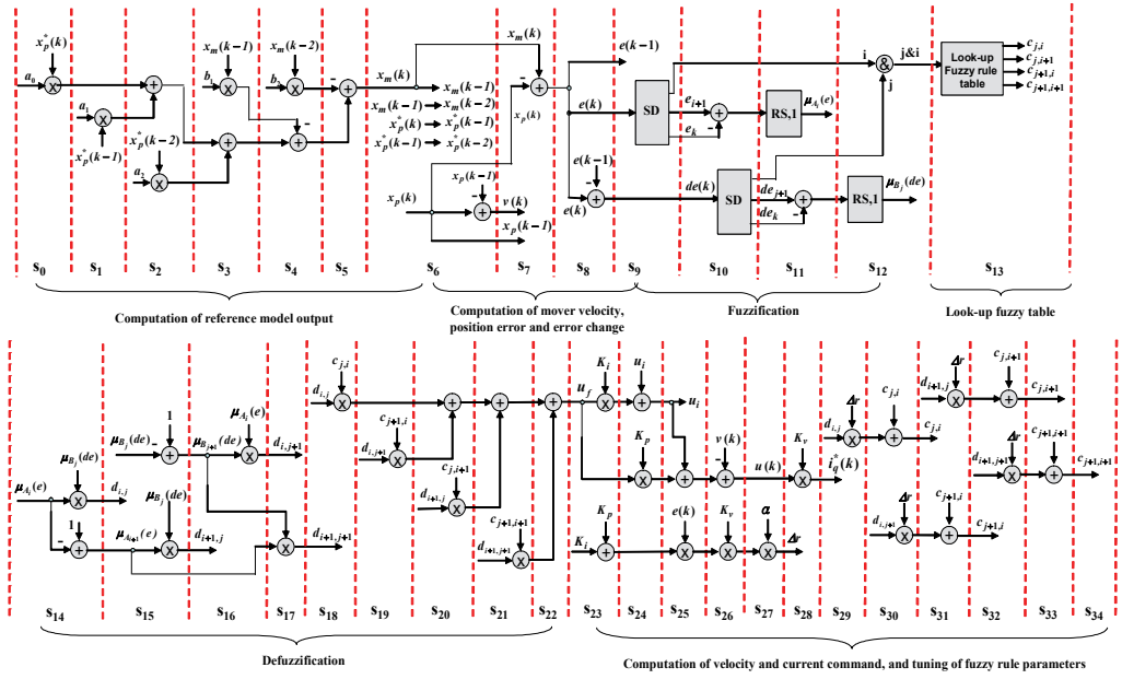
Fig. 10. State diagram of an FSM for describing the AFC in position loop and P controller in speed loop
