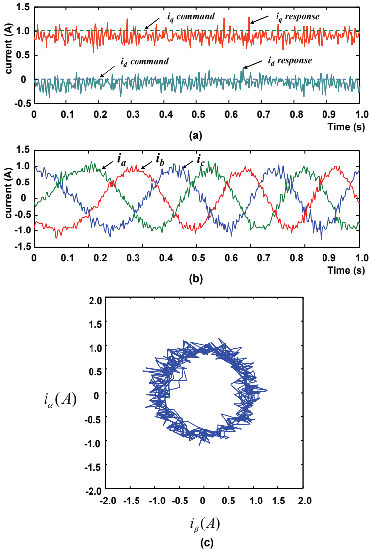
Fig. 12. (a) i_d^*, i_q^* and i_d, i_q response in current control loop (b) Three phase waveforms (c) i_\alpha, i_\beta response in current control loop
