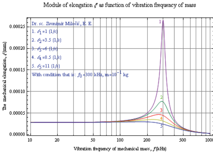
Fig. 1.2 Dependence of module of elongation of mass \xi(f) with concentrated parameters on working frequency f
