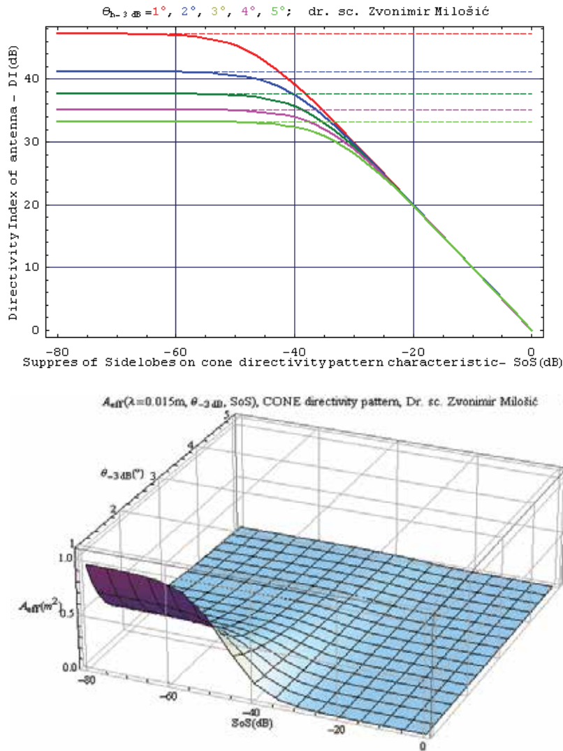
Fig. 6.2.1 Directivity index and effective aperture of antenna at cone directivity pattern characteristic in condition of circle CS of main lobe (Milošić 2008)
