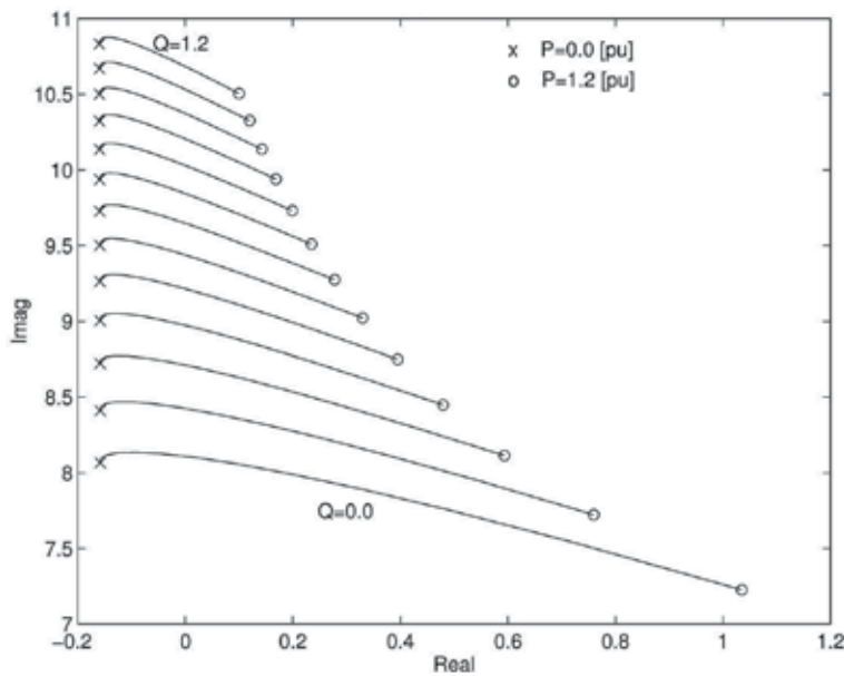
Fig. 5. Conjugate eigenvalue loci as a function of loading, hydrogenerator with voltage control system, 158 MVA
