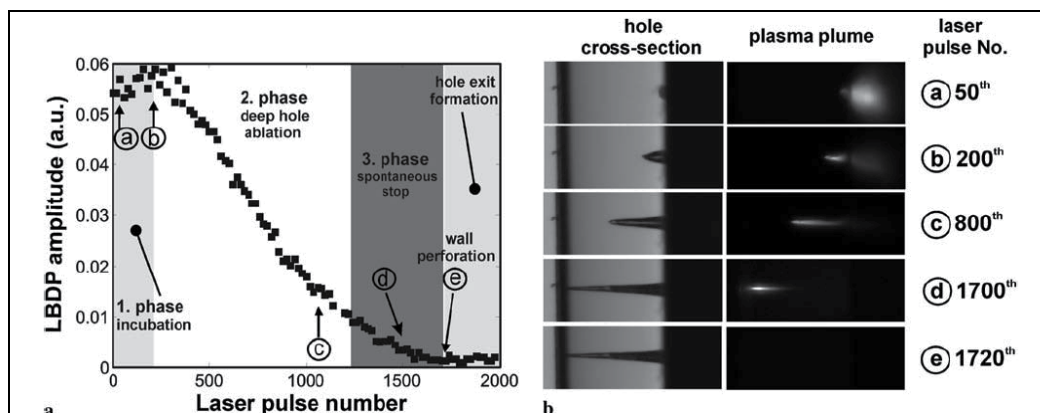
Fig. 15. Phases of the micro-drilling process evident in (a) LBDP signal amplitude diagram and (b) characteristic micrograph images of the hole cross-section and the corresponding plasma plume. Reprinted from (Petkovšek et al., 2008) with kind permission from Springer Science+Business Media
