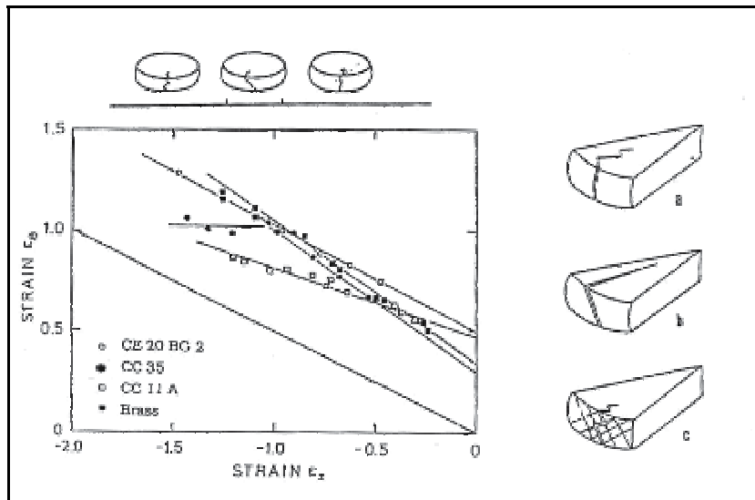
Fig. 7. Formability diagrams for several materials. Cracking modes and their occurrence in the forming limit diagrams (ICFG document 11/01, 2001).
