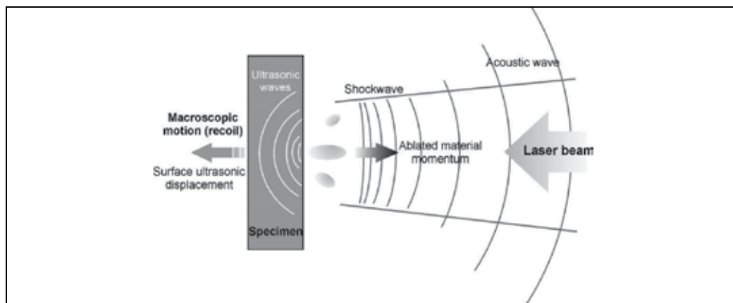
Fig. 1. Optodynamic phenomena during laser material interaction
