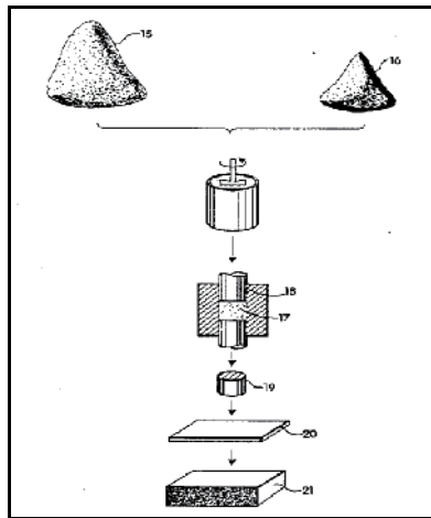
Fig. 1. Sintering of metal powders (US Patent 5,151,246)
