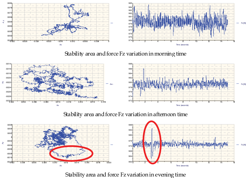
Fig. 17. Stability area and Fz force variation, along Oz, for the 34 years old subject
