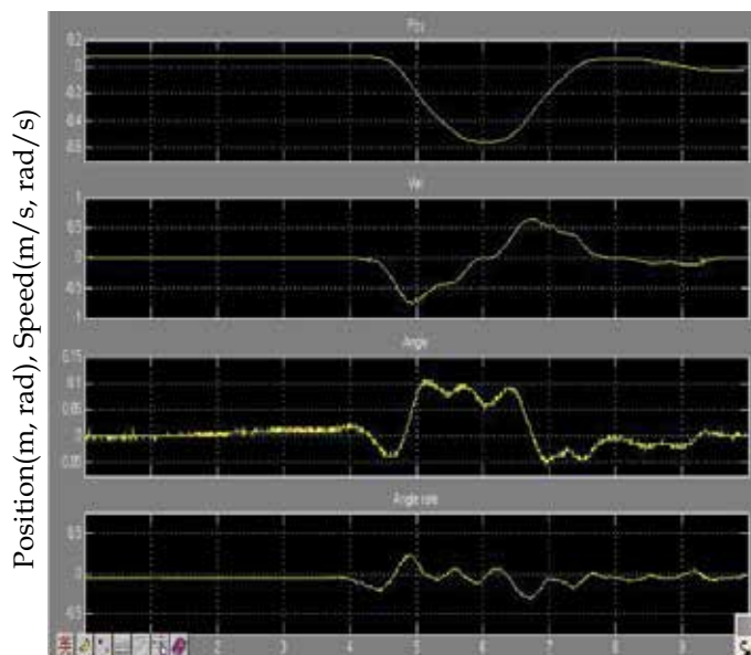
Fig. 13. Real-time control result of T-WIP output response using pole placement controller
