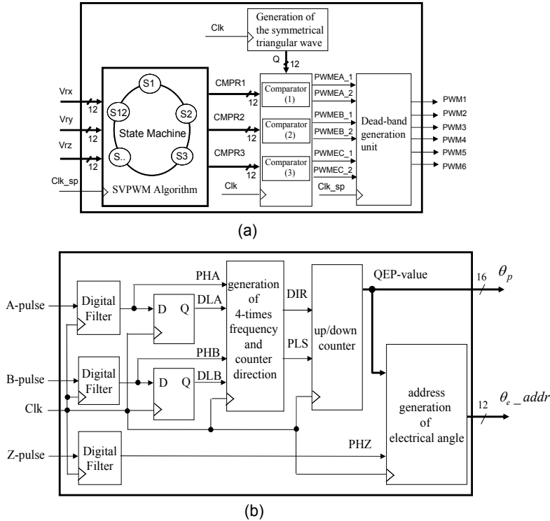
Fig. 11. (a) Circuit of SVPWM generation (b) circuit of QEP detection and transformation
