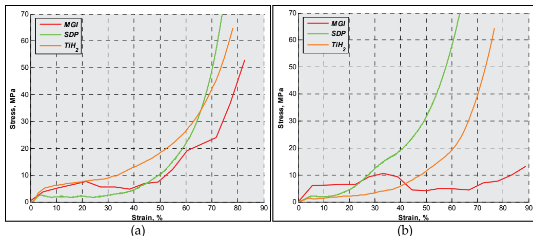
Fig. 16. Stress-strain diagram for 3 samples: a) relative density of 0.25 ( \text{TiH}_2 370-750-5, SDP 30-2-550, MGI 300-8-20), b) relative density of 0.31 ( \text{TiH}_2 310-850-0, SDP 30-3-600, MGI 300-2-15)
