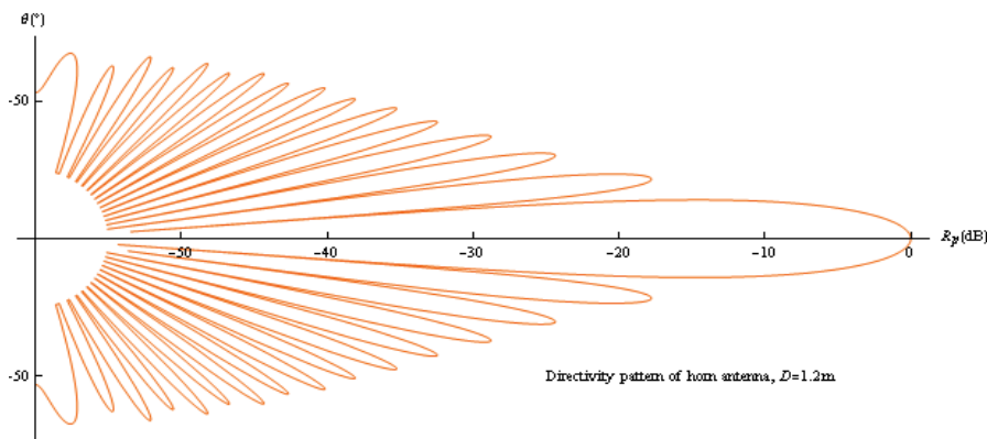
Fig. 5.5 Directivity pattern characteristic of contemporary horn antenna at relations of outside diameter and wave length D_2/\lambda=16 to (5.1)
