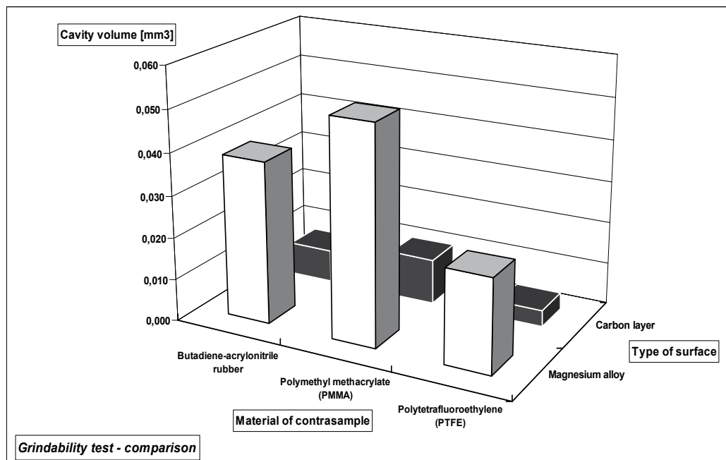
Fig. 7. Comparison of volumetric wear of the specimens of magnesium alloy AZ31 (one covered by the hard carbon coating and the second – without this coating) determined by tribologic measurements
