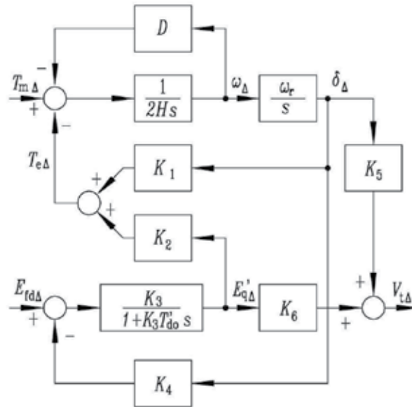
Fig. 1. Simplified linearized model of the synchronous generator connected to an infinite bus conjugate roots and 1 real root. The influence of the machine loading on the synchronous generator dynamic characteristics can be evaluated by eigenvalue loci analysis. The dominant complex conjugate eigenvalues are especially interesting for the dynamic stability analysis. They are directly related to the period and damping ratio of the rotor angle oscillation. The results of the numerical eigenvalue analysis of a typical 160 MVA turbogenerator are presented. The turbogenerator has following parameters:
