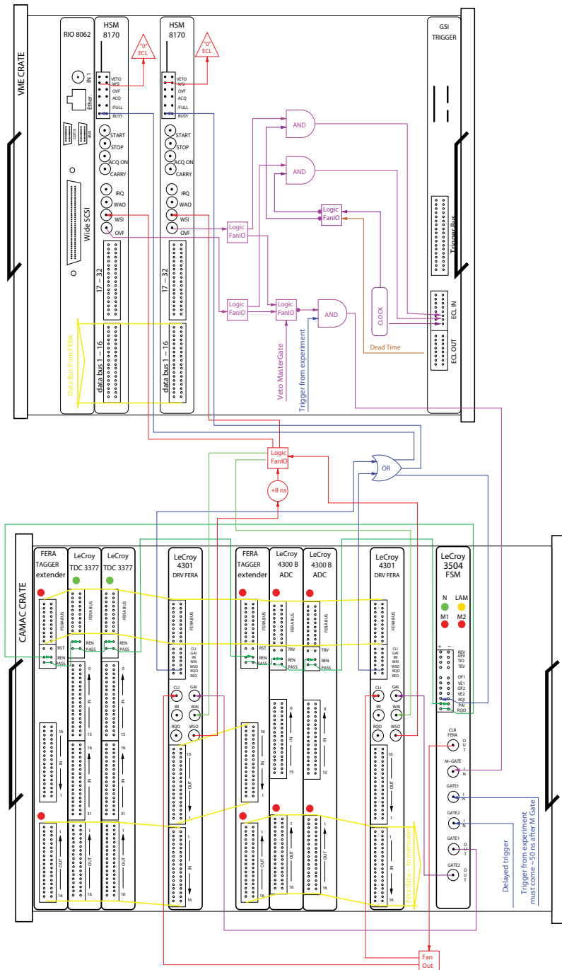
Fig. 7. Full FERA system equipped with the VME buffer Memories (here HSM 8170 serviced by a RIO2 front-end processor). The connections are slightly different than in the case of the CAMAC memories due to particularities in the requirements of the VME modules.
