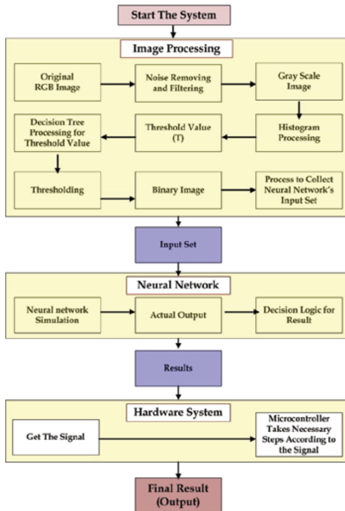
Fig. 2. Major components of the Textile Defect Detector
