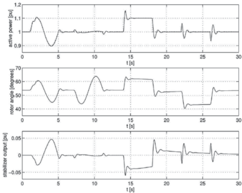
Fig. 9. Generator active power P_e , rotor angle \delta and stabilizer output u_p in the nominal operating point with DAC-PSS
