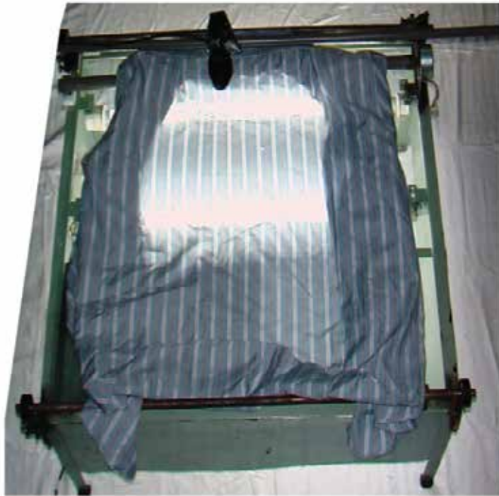
Fig. 13. The real test-bed implementation
