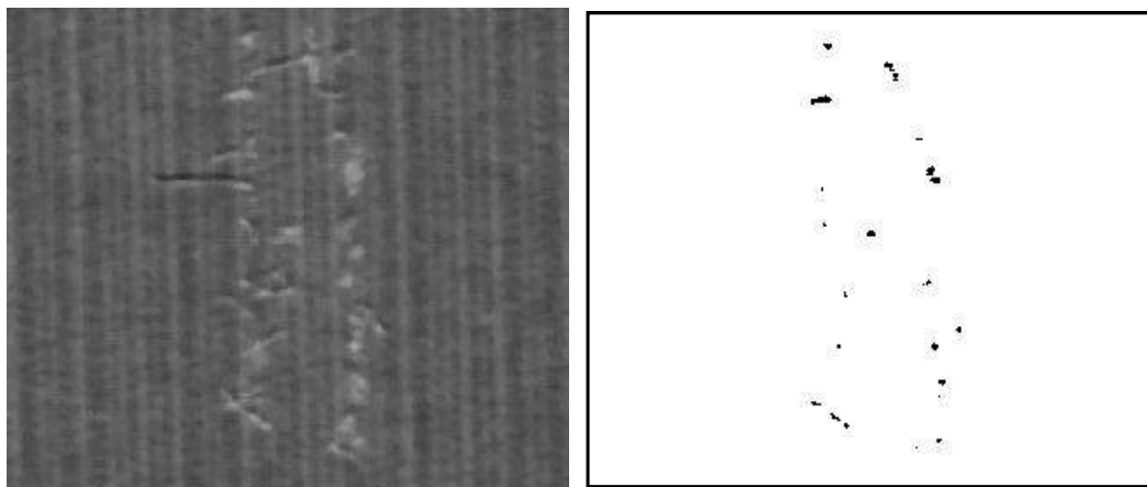
Fig. 4. Faulty scratch grayscale (left) and binary (right) fabric images
