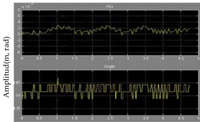
Fig. 14. Real-time control results of vibration scale for T-WIP at equilibrium
