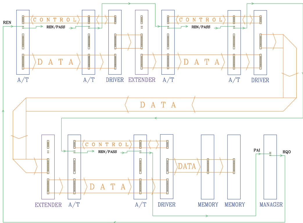
Fig. 3. Schematic diagram of an example of the Separate Gate system, employing the FERA Extender/Tagger as just the data bus extender. Only the REN/PASS chain and the ECL busses are shown.
