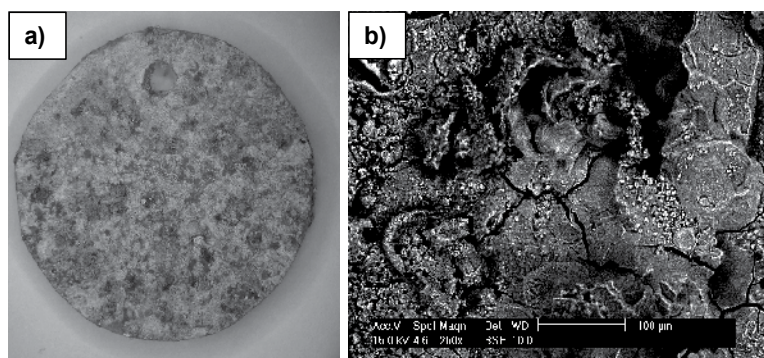
Fig. 8. Microscopic images of AZ31 magnesium alloy specimens without the hard carbon layer after 5h exposition in a salt spray chamber: a) magnification 3x, b) magnification 250x
