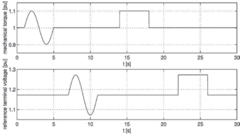
Fig. 7. Mechanical torque T_m and reference terminal voltage V_{t,ref}
