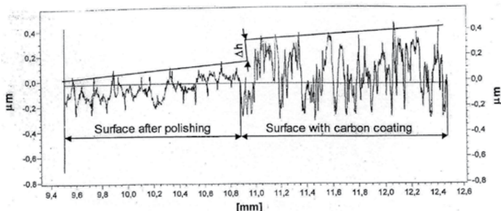
Fig. 5. Results of measurements of the thickness of hard carbon coating deposited on magnesium alloy AZ31 carried out by the method of direct profilography; the thickness of hard carbon coating ( \Delta h ) is equal to 220 nm
