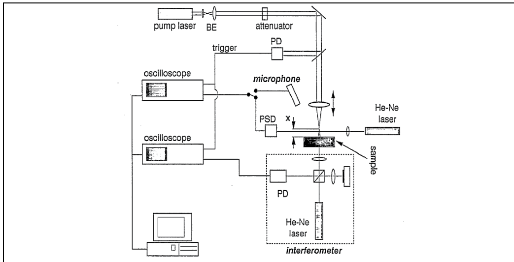
Fig. 7. A set-up for simultaneous detection of OD wave in air and in the workpiece. Reprinted from (Hrovatin & Možina, 1995) with kind permission from Elsevier
