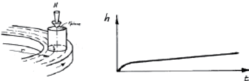
Fig. 1. Pin-on-disc test
