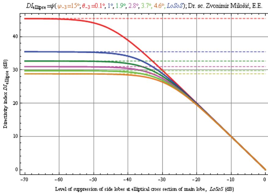
Fig. 6.3.2 Graphic presentation of DI as function of angles of sensitivity \theta_{3\text{dB}} in azimuth and \varphi_{3\text{dB}} in elevation and the level of suppression of side lobes LoSoS of the sonar antenna (Milošić 2007, 2008)
