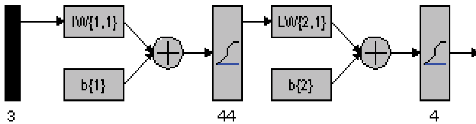
Fig. 7. Design of Feed Forward Back propagation Neural Network
