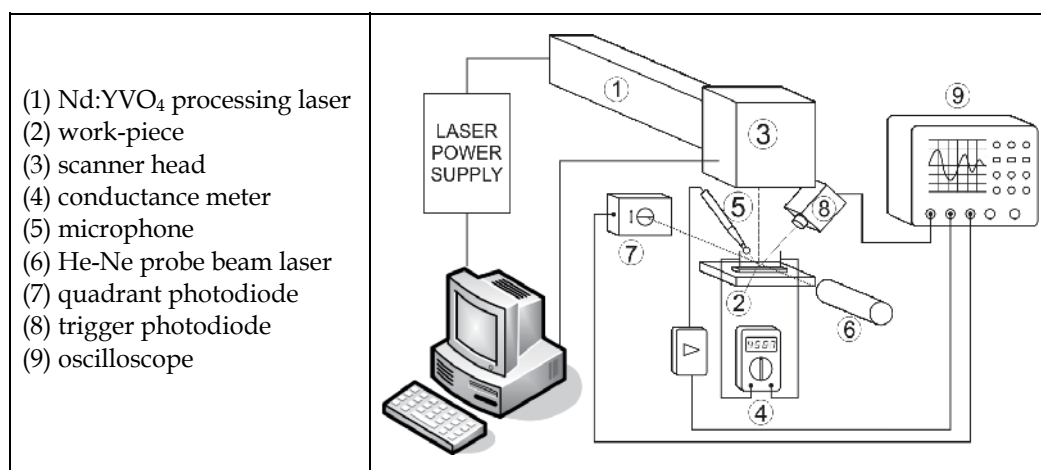
Fig. 17. Experimental set-up for OD analysis of laser engraving. Reprinted from (Gorkič et al., 2009) with kind permission from Springer Science+Business Media
