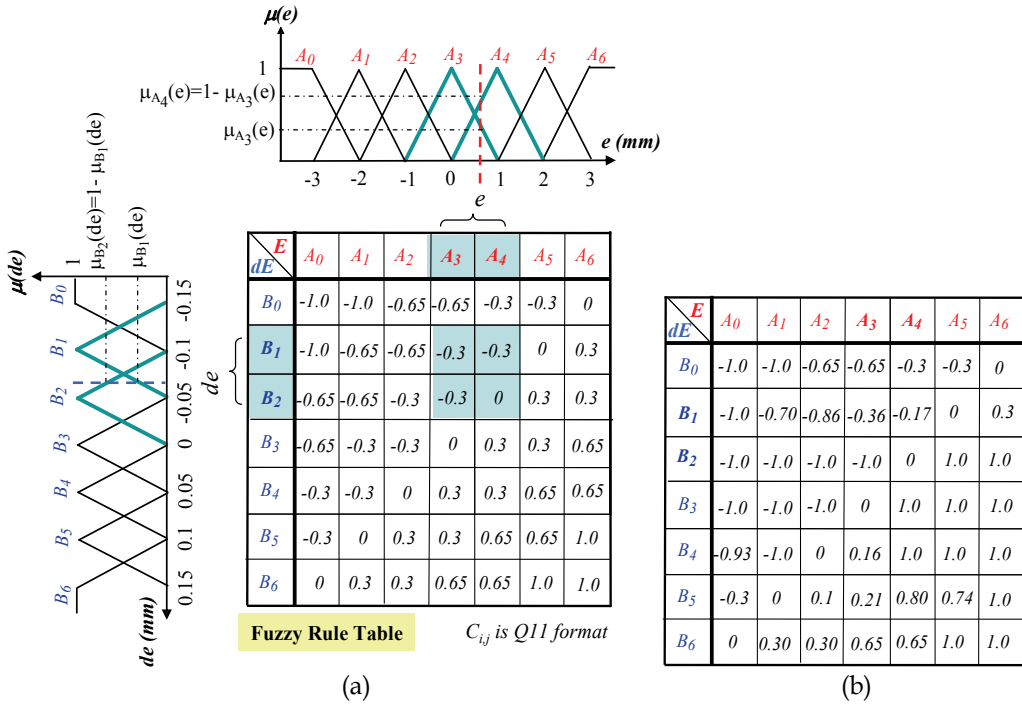
Fig. 13. Fuzzy membership function and (a) the initial fuzzy rule table in experiment (b) the tuned fuzzy rule table at 4 th second
