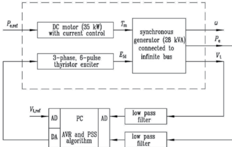
Fig. 12. Testing system block diagram
