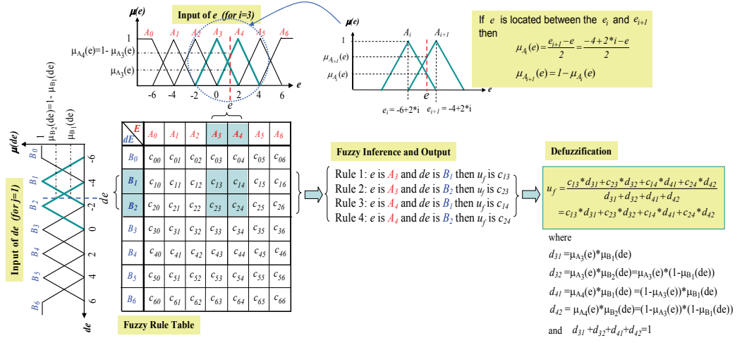
Fig. 7. The symmetrical triangular membership function of e and de , fuzzy rule table, fuzzy inference and fuzzification
