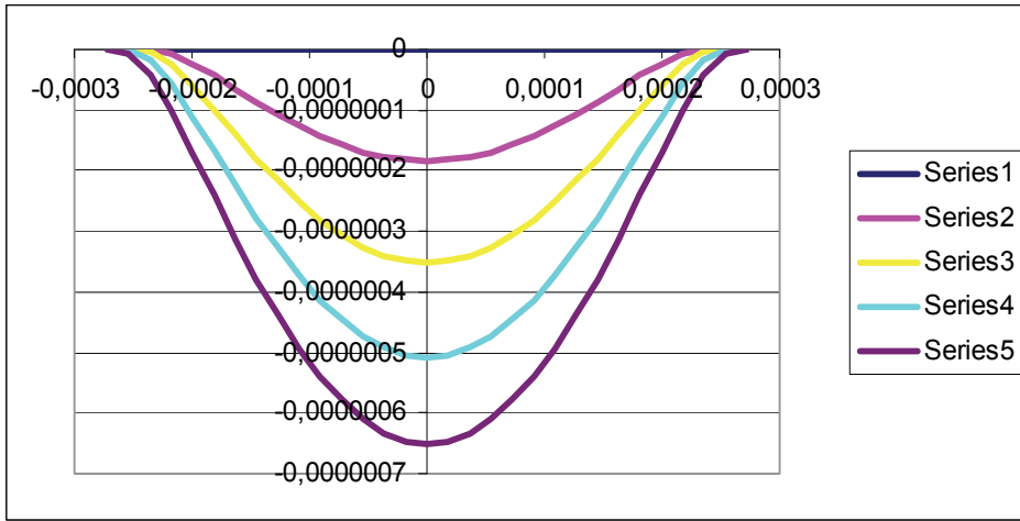
Fig. 14. Simulated wear of an ellipsoidal roller 1 interacting with a cylindrical roller 2. R_{1x} = 25 \cdot 10^{-3} \text{ m} , R_{1y} = 12.5 \cdot 10^{-3} \text{ m} , R_{2x} = 25 \cdot 10^{-3} \text{ m} , F_N = 100 \text{ N} , v_1 = 1.25 \text{ m/s} , v_1 - v_2 = 0.06 \text{ m/s} . Series 1 is at t=0 , Series 2 is after n revolutions, Series 3 is after 2n rev., Series 4 is after 3n rev. and series 5 is after 4n rev.. The figure shows the change in shape of the contact surface of the rollers during running.
