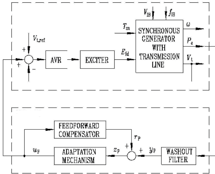
Fig. 6. Block diagram of the DAC-PSS structure
