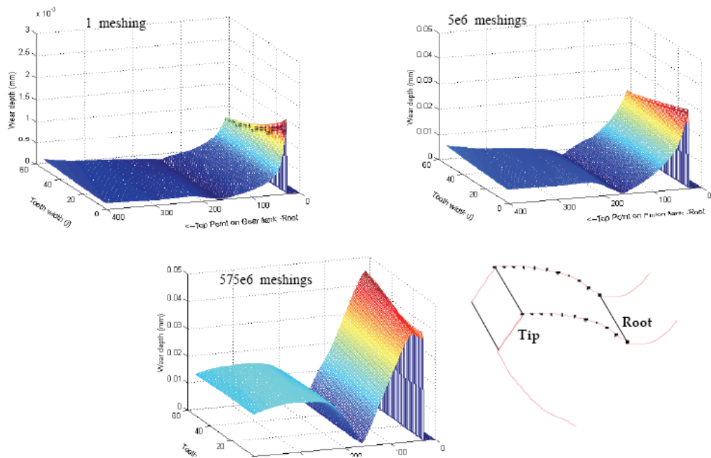
Fig. 15. Wear simulation results obtained by Flodin [18]
