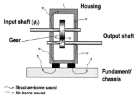
Fig. 18. Noise excitation from a gearbox [22]
