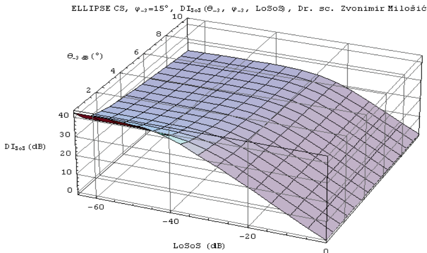
Fig. 6.3.3 Graphic presentation of DI(\theta_{3\text{dB}}, \varphi_{3\text{dB}}, LoSoS) in three dimensions have a special meaning by comparison of different sonar systems (Milošić 2007, 2008)
