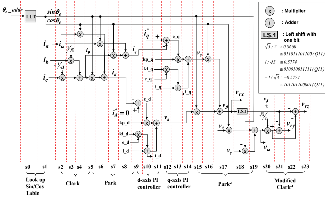
Fig. 9. Designed CCCT circuit in Fig. 8
