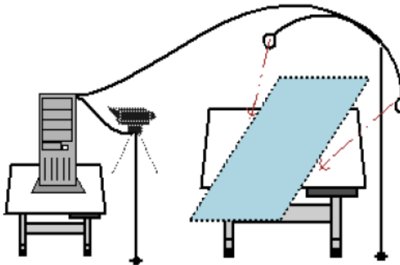
Fig. 1. Real-time Environment of Textile Defect Detector
