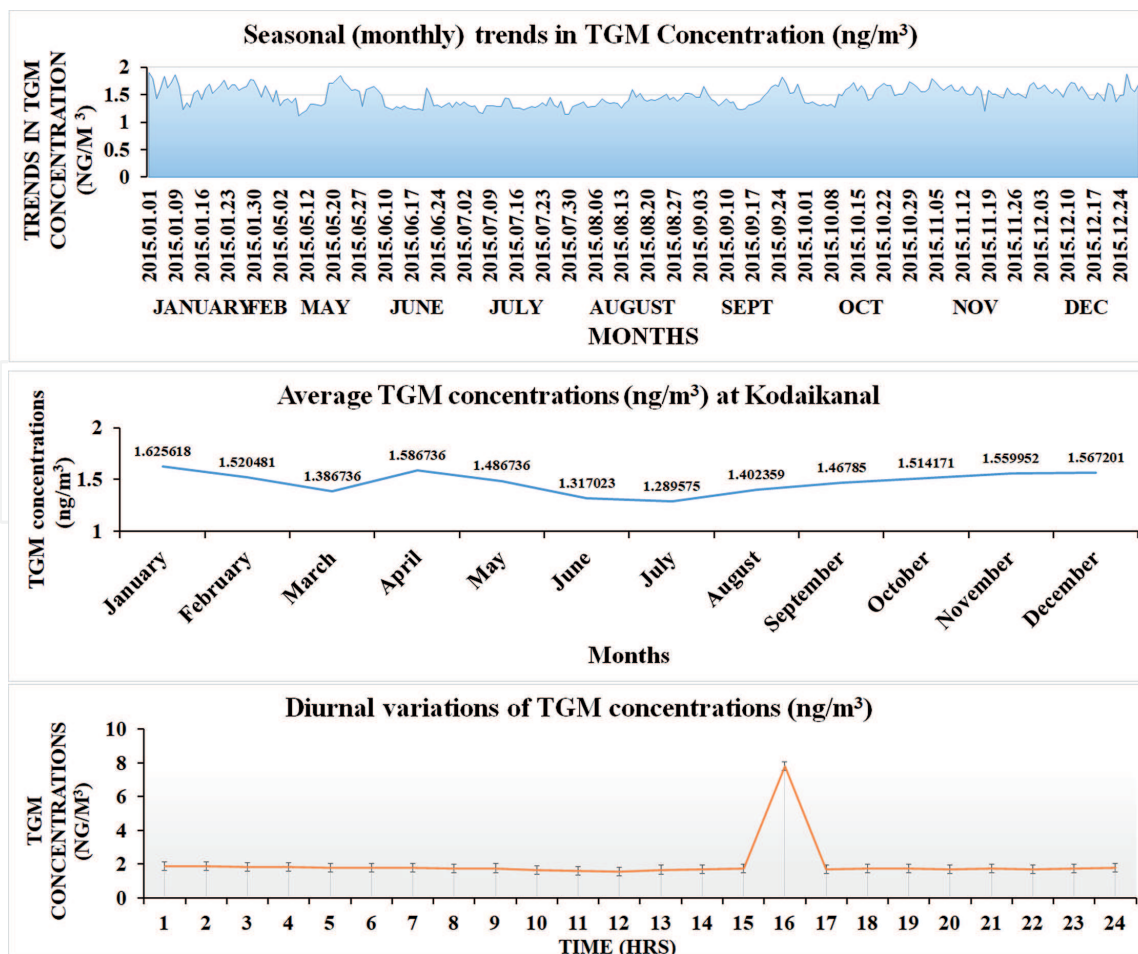
Figure 2. Diurnal and monthly variation of TGM concentration in high-altitude background station (Kodaikanal) in South India.
