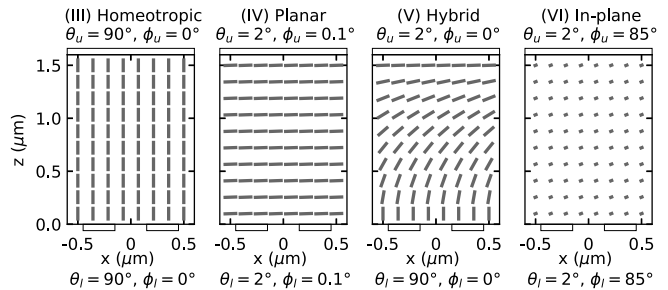
FIG. 1. Illustration of the surface alignment configurations analysed in sections III-VI where grey line segments represent the starting director configurations (at time = 0) chosen for the simulations. Pre-tilt, \theta , and pre-twist, \phi , at the upper ( u ) and lower ( l ) alignment layer are indicated, where \hat{n} = (\cos \theta \cos \phi, \cos \theta \sin \phi, \sin \theta)^T .
