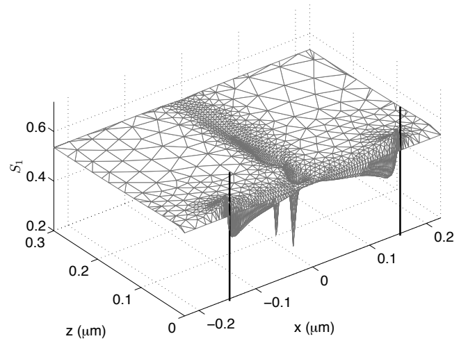
FIG. 4. Order parameter S_1 in the vicinity of the electrode edges at 34 \mu\text{s} , 1 \mu\text{s} after disclination formation. Dark lines show the positions of the electrode edges. Dips in order along x = 0 correspond to disclinations. The high electric field above the electrodes gives rise to an order parameter in excess of that of the bulk ( S_0 = 0.535 ), which peaks above the electrode edges. Between electrodes the clash between the surface alignment and reorienting liquid crystal gives rise to a biaxial arrangement of liquid crystal and, correspondingly, a drop in S_1 .
