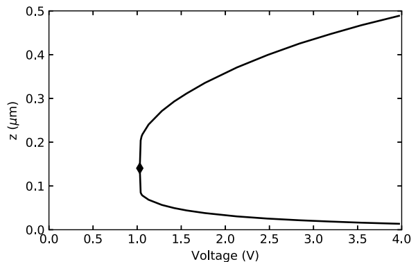
FIG. 7. Steady-state vertical position of \pm 1/2 disclinations as a function of voltage, as the applied voltage is reduced from \pm 3.97 \text{ V} . Height is almost temperature invariant, but for the weak dependence of the permittivity on the order parameter.
