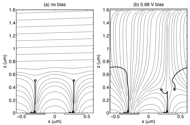
FIG. 9. Director streamlines at steady-state with planar alignment. In (a) \pm 5.19 V is applied to the lower electrodes and the upper electrode is grounded. Steady-state is reached after \sim 2 ms. With a bias in (b), the approach to steady-state is slowed significantly, as the -1/2 lines migrate to the same height driven by their mutual repulsion (after 16 ms).
