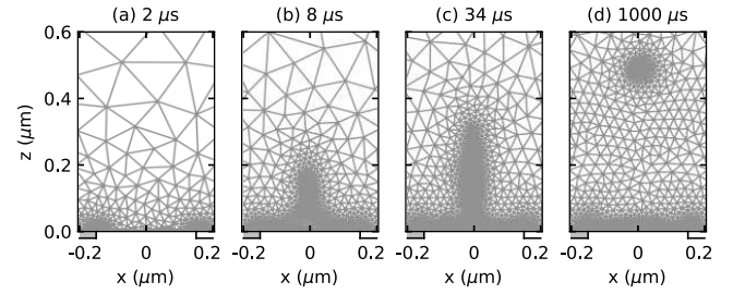
FIG. 3. Mesh in the vicinity of the electrode edges at four different times. Throughout the modelling window the element edge-length varies from 0.25 to 400 nm. Element count peaks at 34 \mu\text{s} with 8400 triangles.
