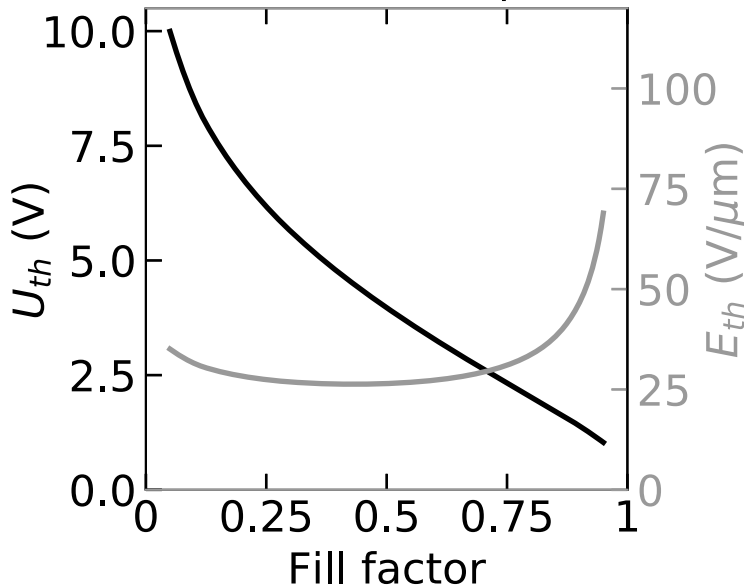
(a) Homeotropic
