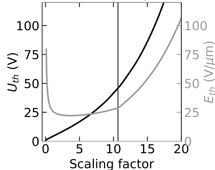
(c) Homeotropic
