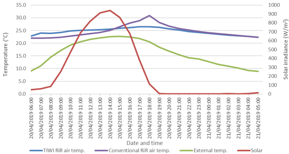
Figure 7-21 internal and external environmental conditions experienced during a warm and sunny 24-hour period during the baseline test
