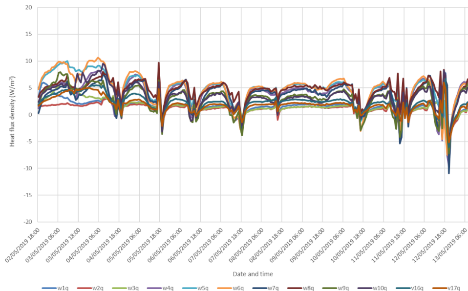
Figure 7-20 Heat flux density measured by each HFP on the conventional RiR post-retrofit
