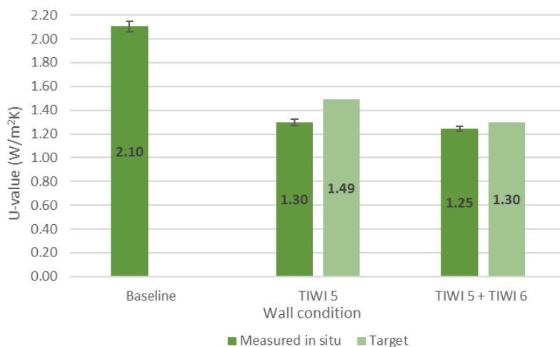
Figure 3-7 Mean in situ U-value and retrofit target U-values for the test wall of House C in each condition
