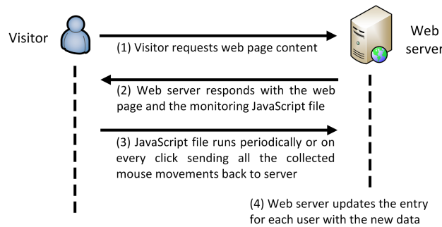
Fig. 4. Mouse movement collection process.
