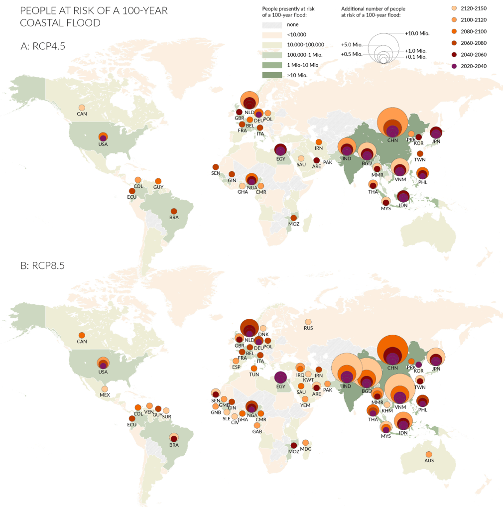
Fig. 4. Number of people at risk of 100-year coastal flood in 2020 (green shades; landlocked countries with grey stripes). The colour of the circles indicates when an impact threshold is exceeded for the median value of RCP4.5 (a) and RCP8.5 (b) according to IPCC SROCC (Oppenheimer et al., 2019) projections. Impact thresholds considered are 0.1, 0.5, 1, 5 and 10 million people per country that will become at risk of a 100-year flood event, in addition to the people currently at risk of a 100-year flood event, assuming present population and protection. The size of the circles indicates the additional number of people that become at risk compared to the current population at risk. Where circles have similar colours, risk increases rapidly. Countries with dark colours have an early increase of risk. Countries with small circles have lower risk until 2150. This information is provided for countries, in which the minimum threshold of 100,000 people additionally at risk will be exceeded by 2150. (For interpretation of the references to colour in this figure legend, the reader is referred to the web version of this article.)
