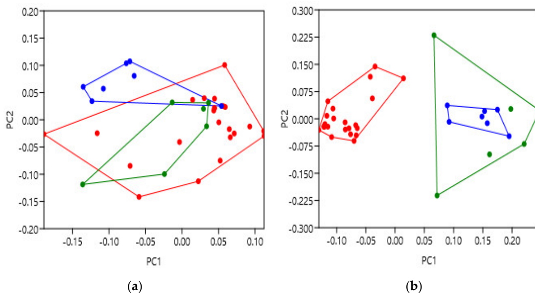
Figure 3. Principal component analysis to show the \beta_2 -adrenergic receptor ( \beta_2 AR) shape variation between activation states. Inactive structures are red, active are blue and active with G_s coupled are green. (a) PC score comparison for the extracellular face of the \beta_2 AR transmembrane bundle. (b) PC score comparison for the intracellular face of the \beta_2 AR transmembrane bundle. The supporting statistical data are summarised in Tables 2 and 3. Additional supporting figures are found in Appendix B Figure A1.
